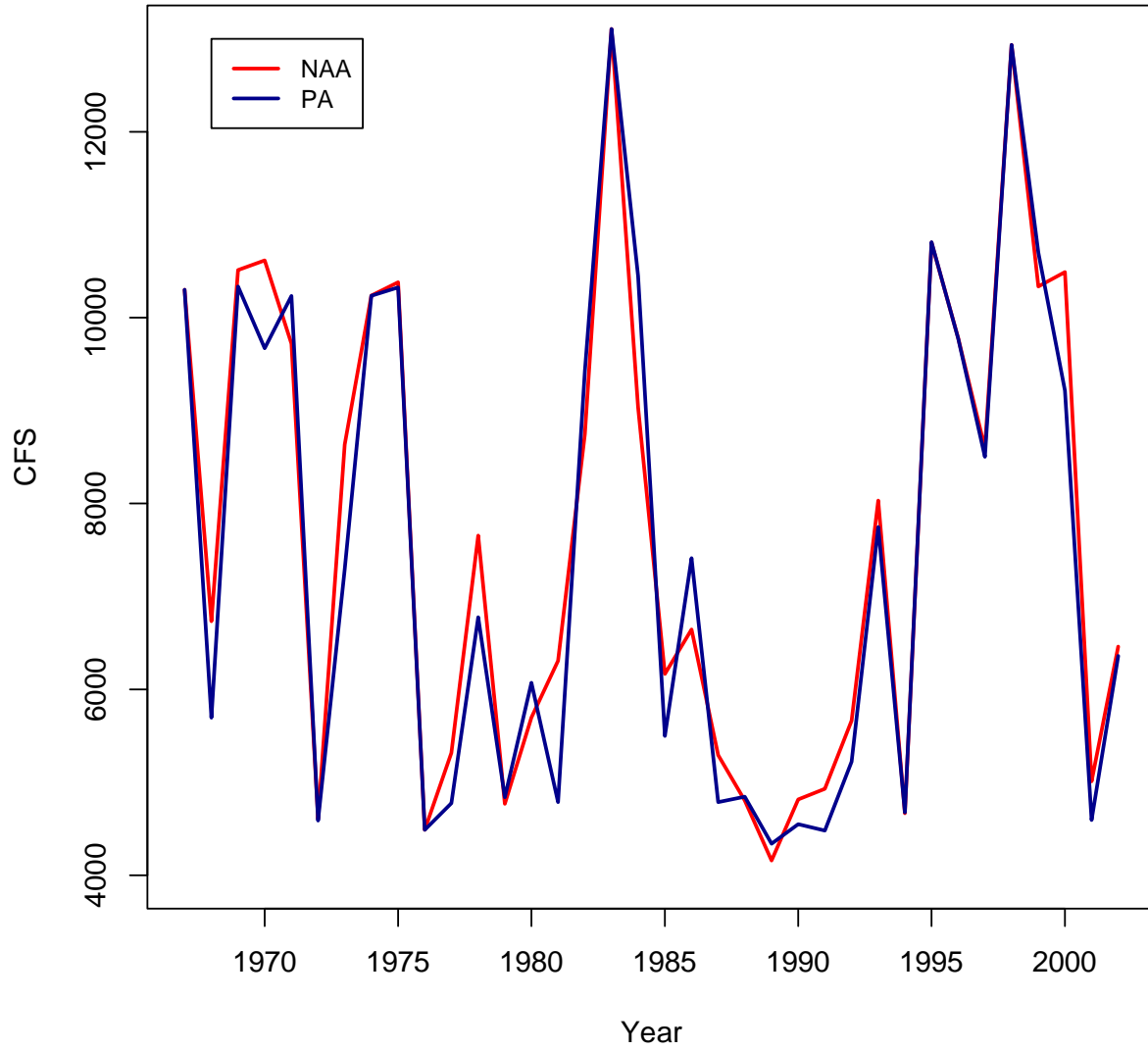
Figure 5.D-160. OBAN FLMIN Covariate: Minimum of monthly mean flow between August and November at Bend Bridge in cubic feet per second (CFS).
