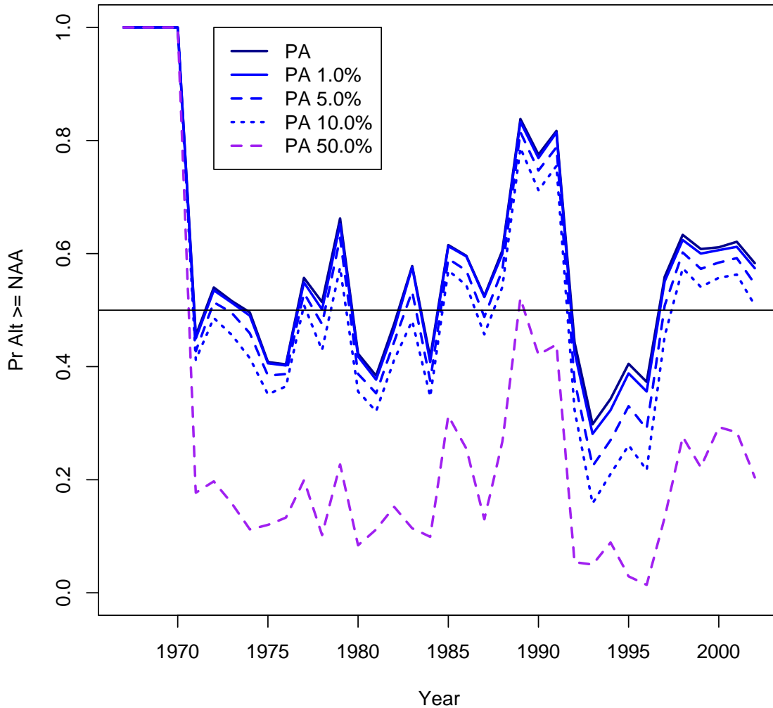
Figure 5.D-183. OBAN: Probability of higher annual abundance in a PA scenario relative to the NAA scenario. The horizontal black line at 0.5 indicates an equal probability that escapement is higher in a PA scenario relative to the NAA scenario.
