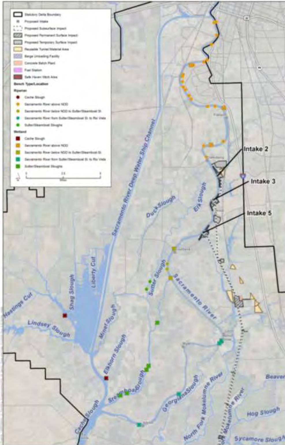
Figure 5.D-84. Benches Analyzed for Inundation Effects of the PA.
