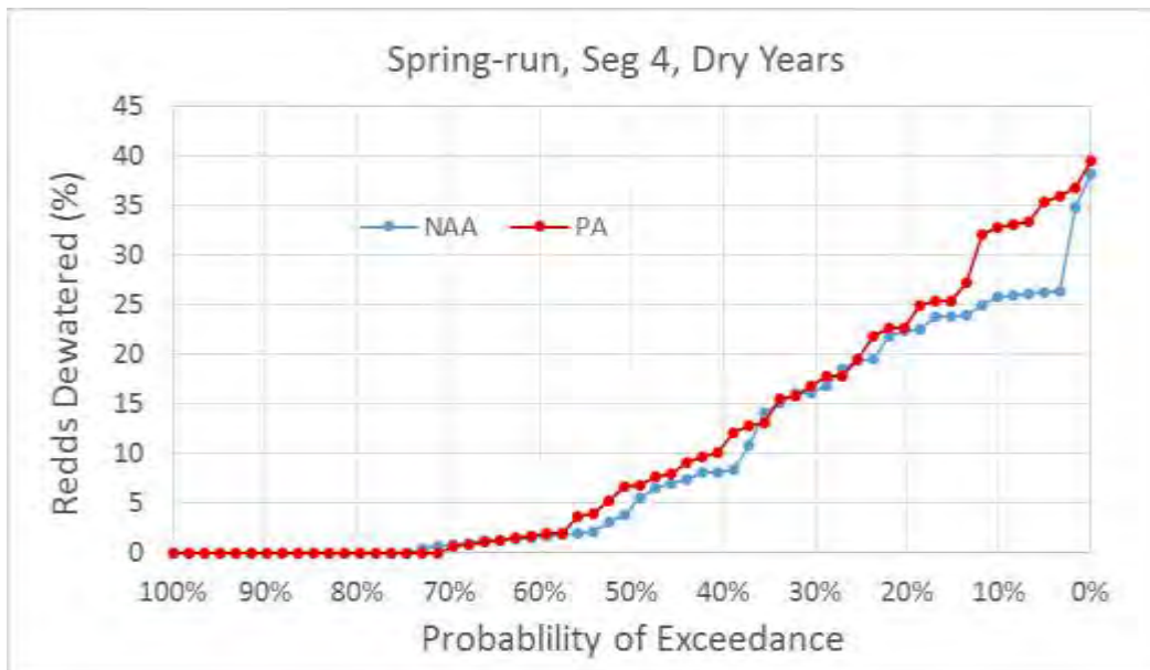
Figure 5.D-121. Exceedance Plot of Spring-Run Chinook Salmon Percent of Redds Dewatered for NAA and PA Model Scenarios in River Segment 4, Dry Water Years
