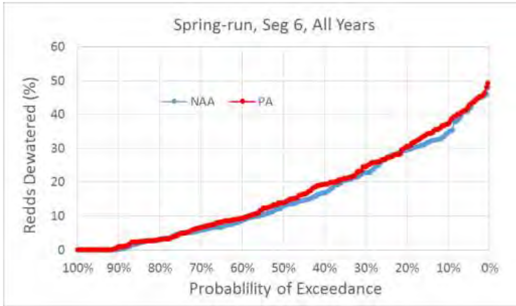
Figure 5.D-112. Exceedance Plot of Spring-Run Chinook Salmon Percent of Redds Dewatered for NAA and PA Model Scenarios in River Segment 6, All Water Years
