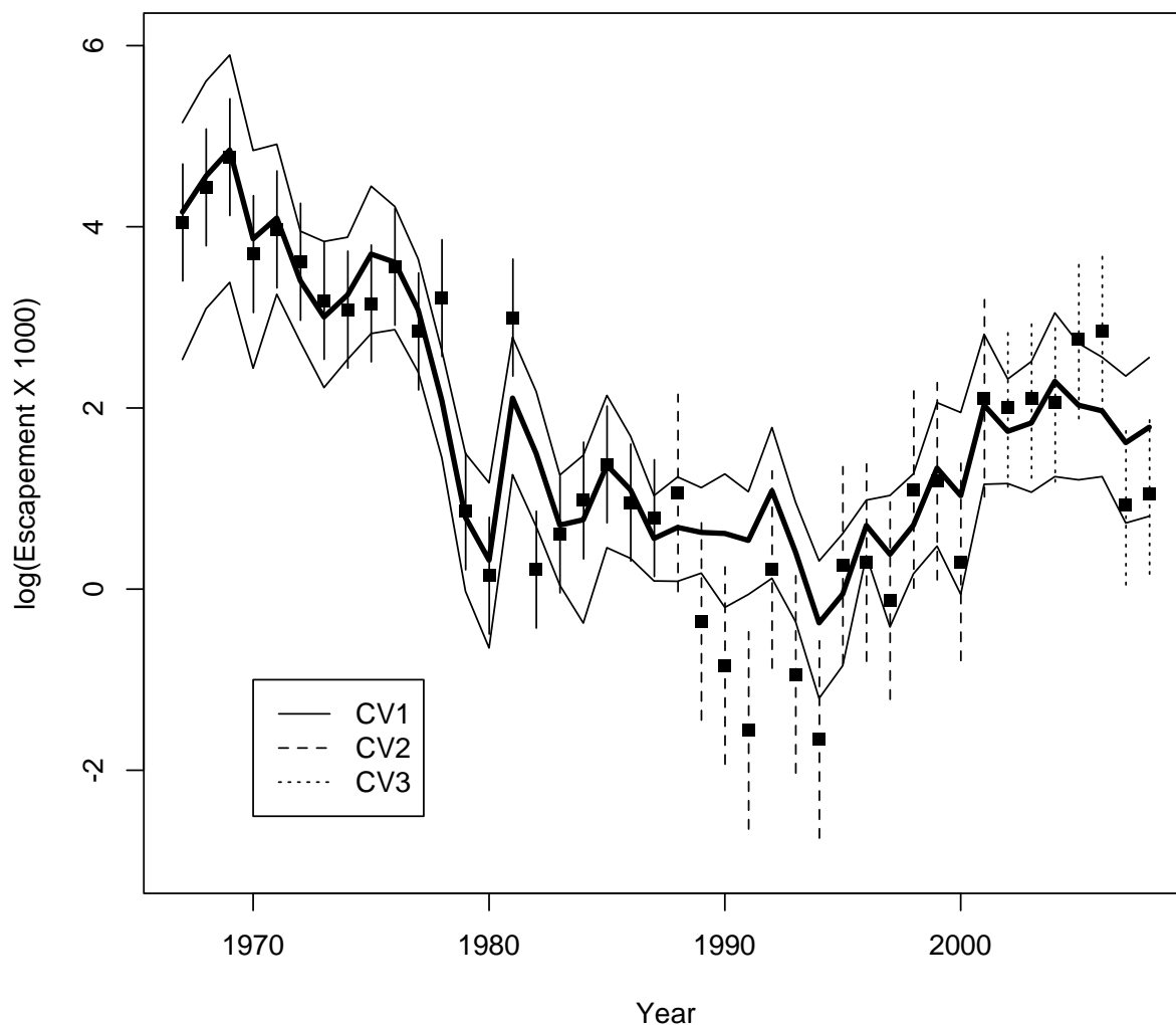
Figure 5.D-156. Mean Prediction (thick line) and 95% probability interval (thin line) of winter-run OBAN 2015 model to winter-run log escapement data (black squares) that were collected via ladder counts (CV1), expansion counts (CV2), and carcass surveys (CV3). Vertical bars represent 1 standard deviation for each of the survey methods.
