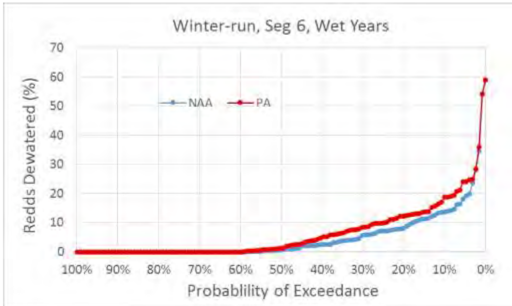
Figure 5.D-101. Exceedance Plot of Winter-Run Chinook Salmon Percent of Redds Dewatered for NAA and PA Model Scenarios in River Segment 6, Wet Water Years
