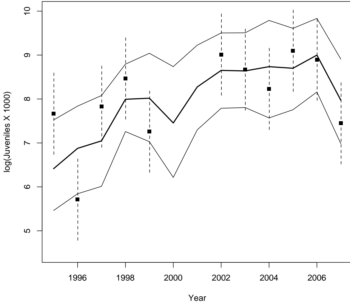
Figure 5.D-157. Mean Prediction (thick line) and 95% probability interval (thin line) of winter-run OBAN 2015 model to winter-run log juvenile count data at Red Bluff Diversion Dam (black squares). Vertical bars represent 1 standard deviation.
