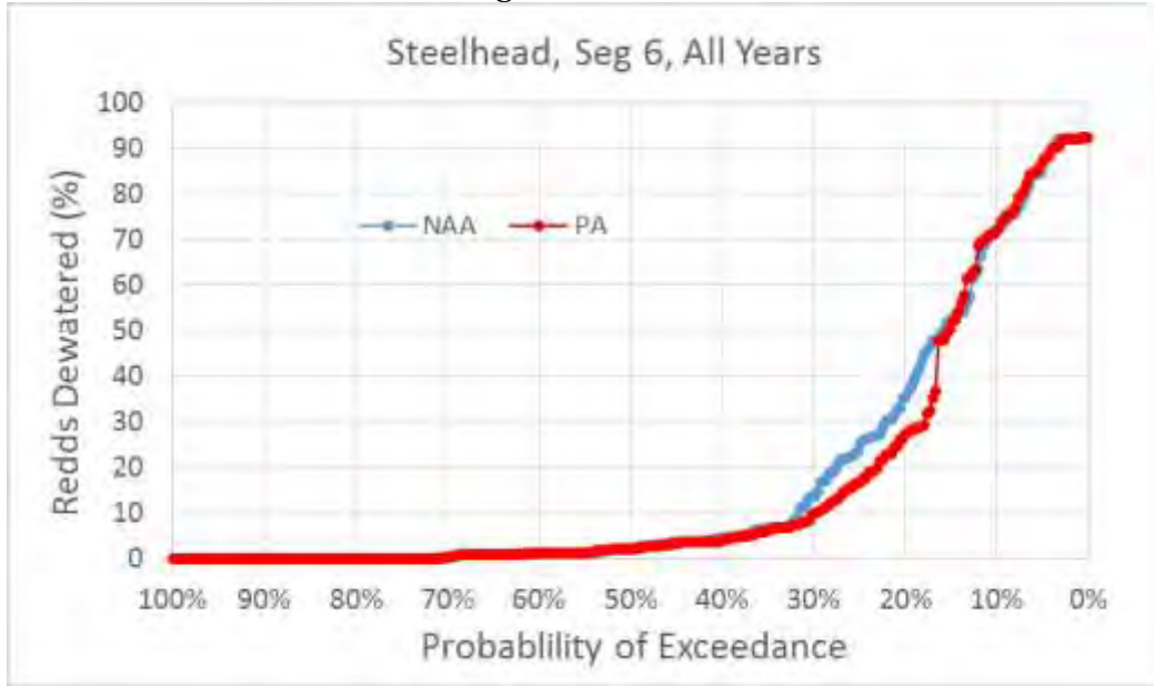
Figure 5.D-123. Exceedance Plot of Central Valley Steelhead Percent of Redds Dewatered for NAA and PA Model Scenarios in River Segment 6, All Water Years
