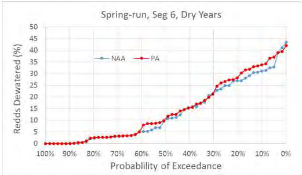
Figure 5.D-116. Exceedance Plot of Spring-Run Chinook Salmon Percent of Redds Dewatered for NAA and PA Model Scenarios in River Segment 6, Dry Water Years
