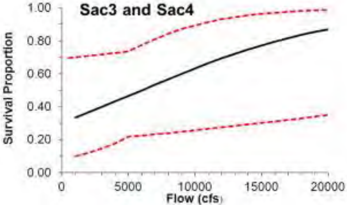
Figure 5.D-65. Juvenile Chinook Salmon Survival in DPM Reaches Sac3 and Sac4 (Sacramento River at Georgiana Slough to Chipps Island) as a Function of Sacramento River Flow Below Georgiana Slough, As Implemented for the Analysis Based on Perry (2010).
