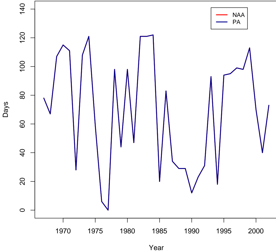
Figure 5.D-158. OBAN Inputs for the Yolo Covariate: Number of days where flow over the Fremont Weir into the Yolo bypass is greater than 100.1 cfs from December thru March.
