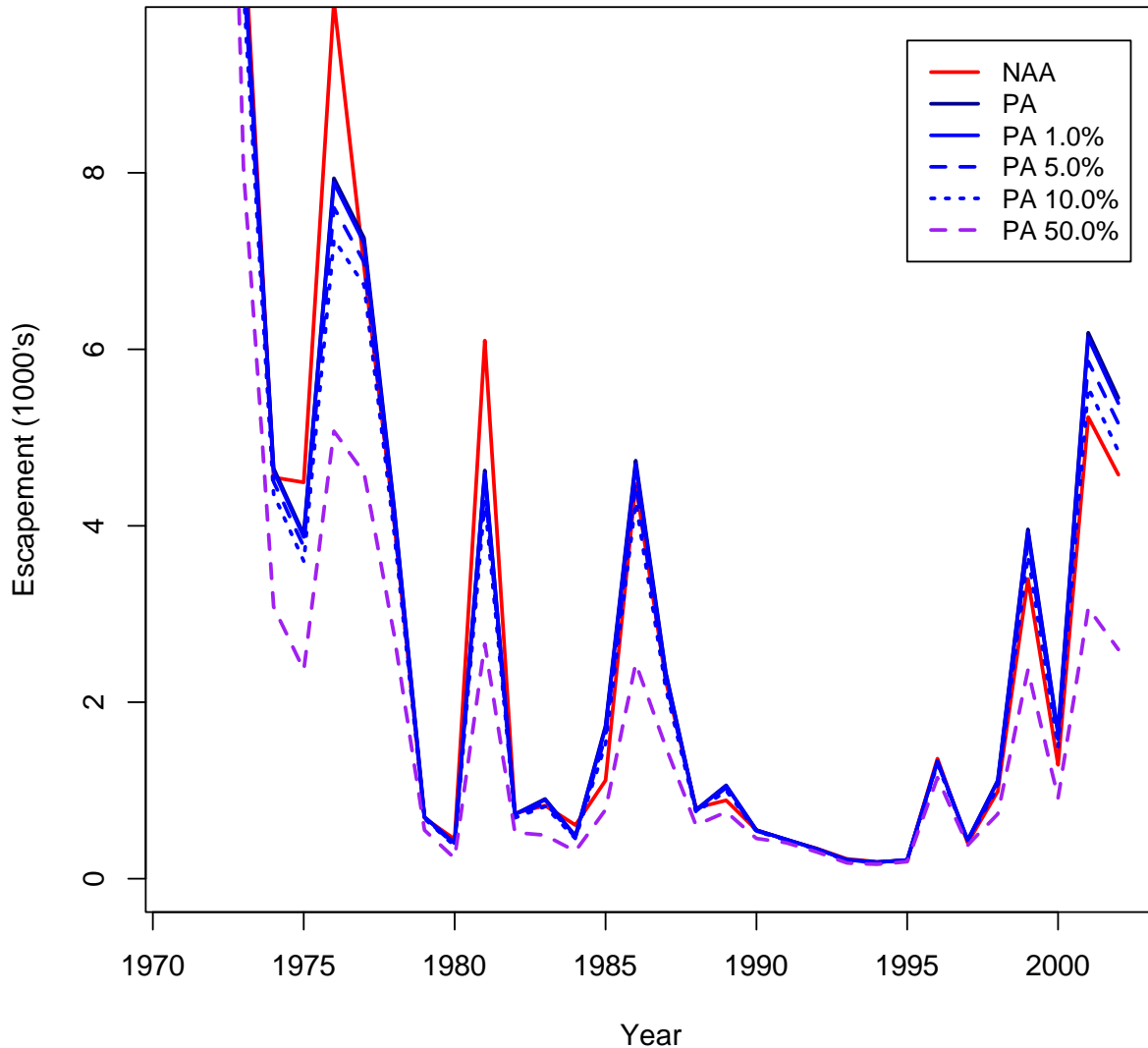
Figure 5.D-162. OBAN: Median escapement for each of the scenarios.
