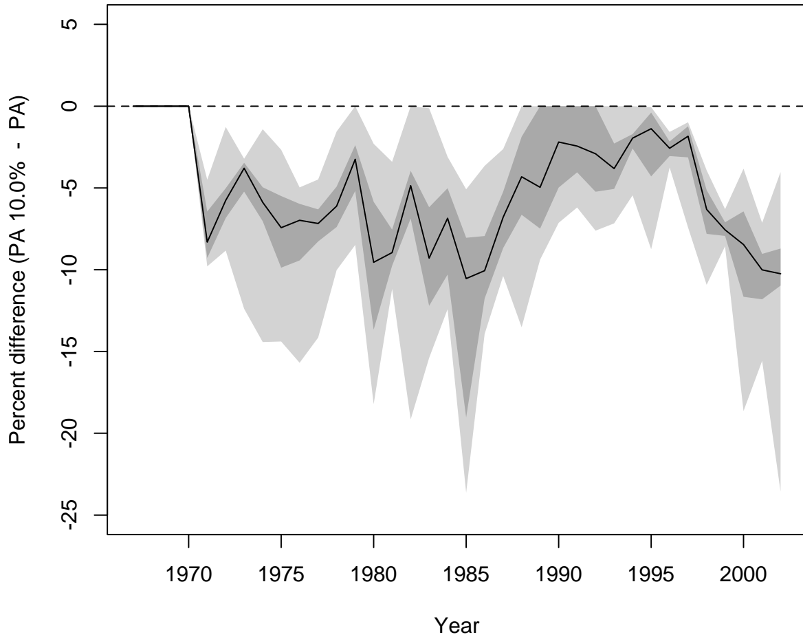
Figure 5.D-175. OBAN: Percent relative difference in escapement of PA 10.0% compared to PA (PA 10.0% – PA)/PA*100%. Median (black line) 50% interval (dark grey) and 90% intervals (light gray) are plotted.
