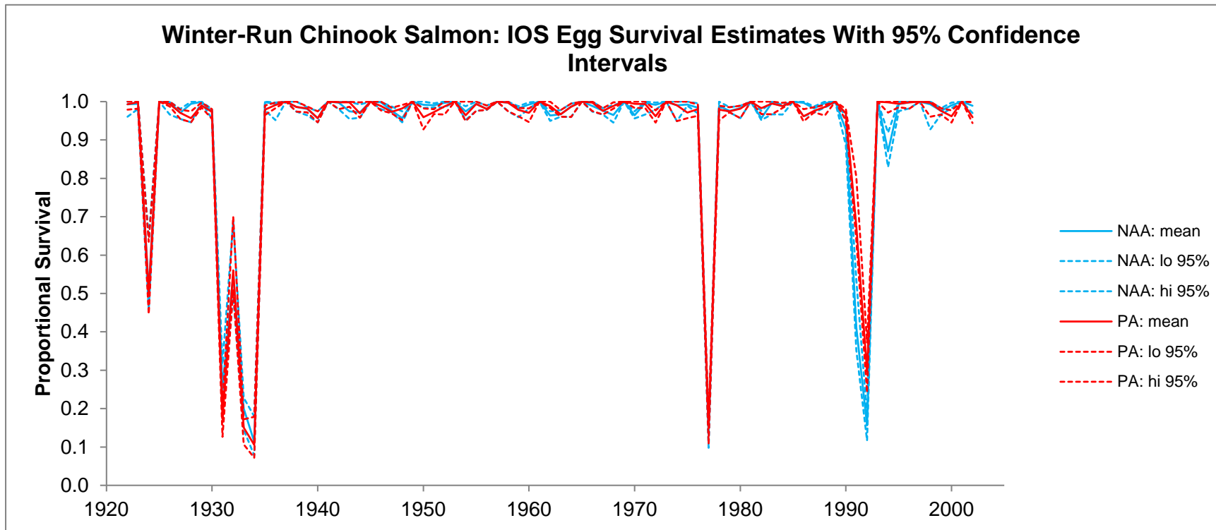
Figure 5.D-142. IOS Annual Winter-Run Chinook Salmon Egg Survival Estimates with 95% Confidence Intervals.
