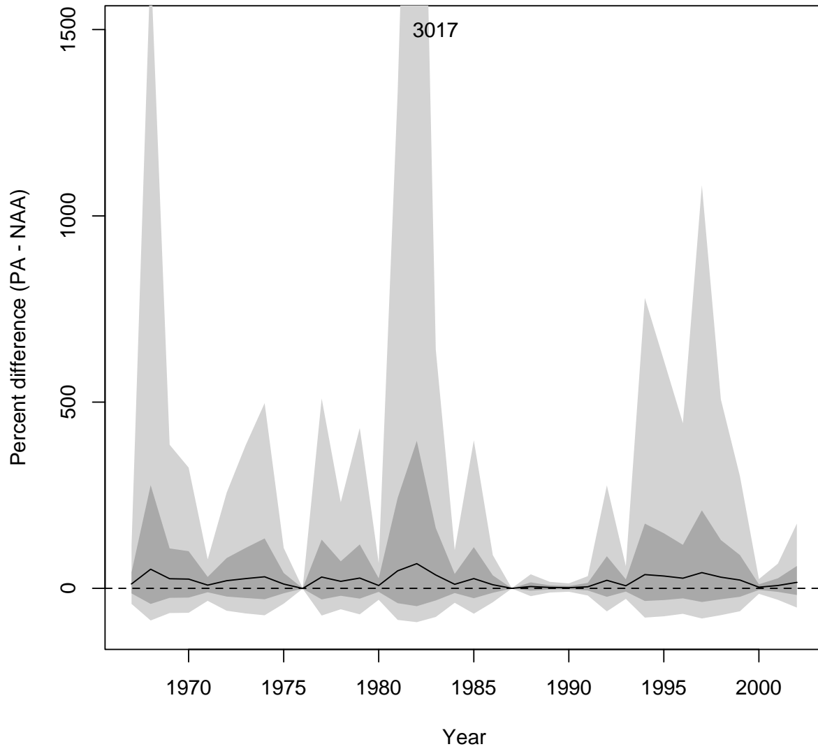
Figure 5.D-178. OBAN: Percent difference in Delta survival of PA compared to NAA ( (PA - NAA)/NAA * 100\% ). Median (black line) 50% interval (dark grey) and 90% intervals (light gray) are plotted.
