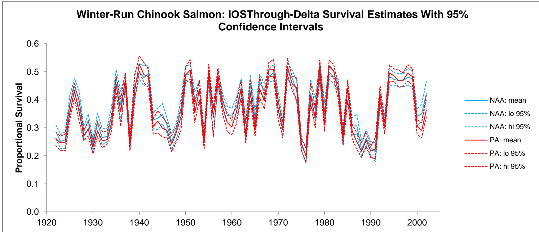
Figure 5.D-148. IOS Annual Winter-Run Chinook Salmon Through-Delta Survival Estimates with 95% Confidence Intervals.
