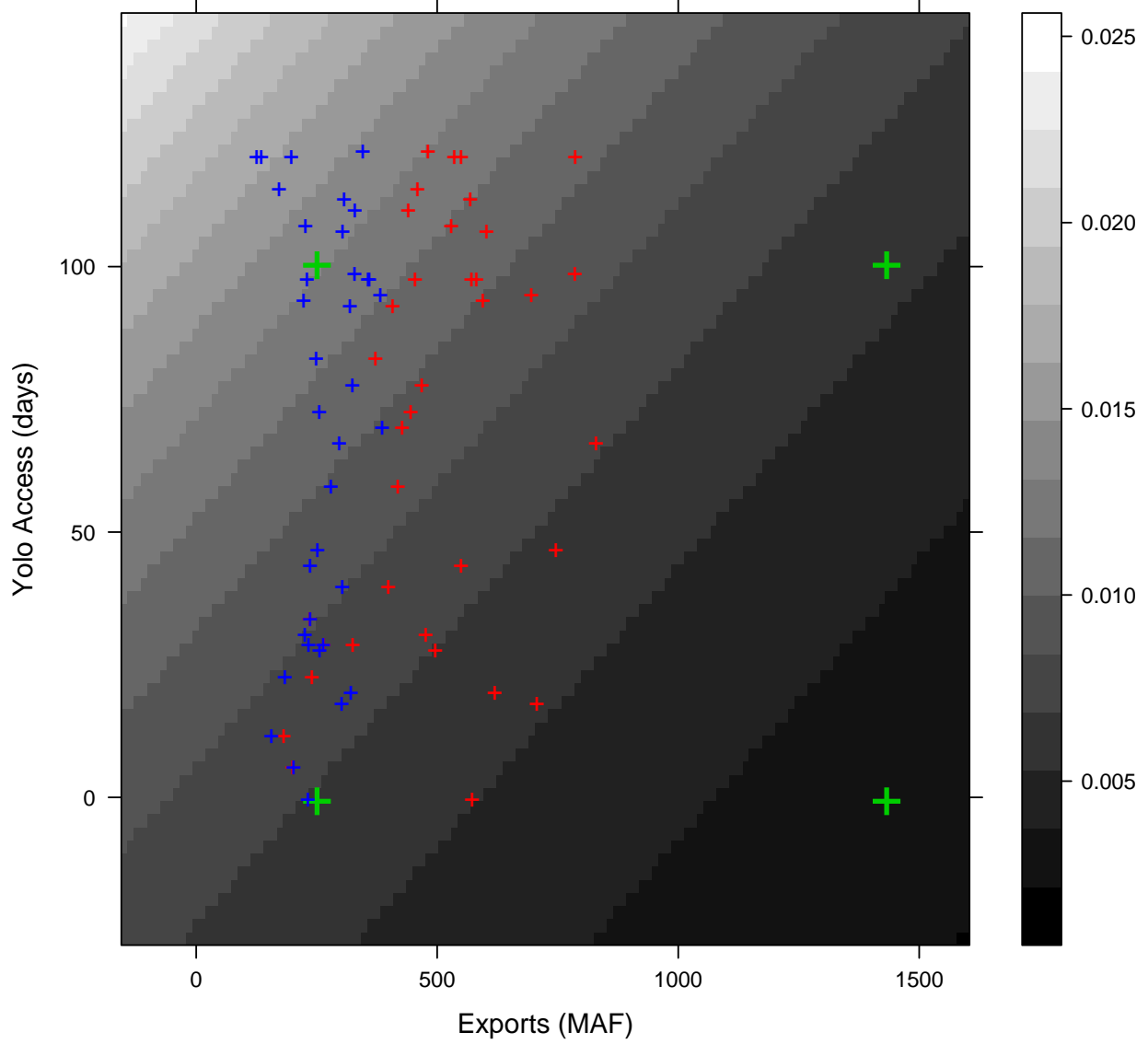
Figure 5.D-166. OBAN: Median survival estimates (surface) in the Delta as a function of Yolo access and south Delta exports. Green crosses indicate bounds of historical data from 1967 to 2010. Annual values of Yolo access and south Delta exports under the NAA (red crosses) and PA (blue crosses).
