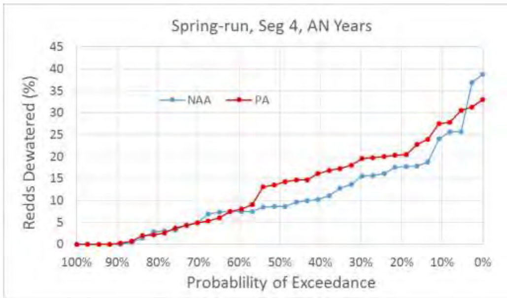
Figure 5.D-119. Exceedance Plot of Spring-Run Chinook Salmon Percent of Redds Dewatered for NAA and PA Model Scenarios in River Segment 4, Above Normal Water Years
