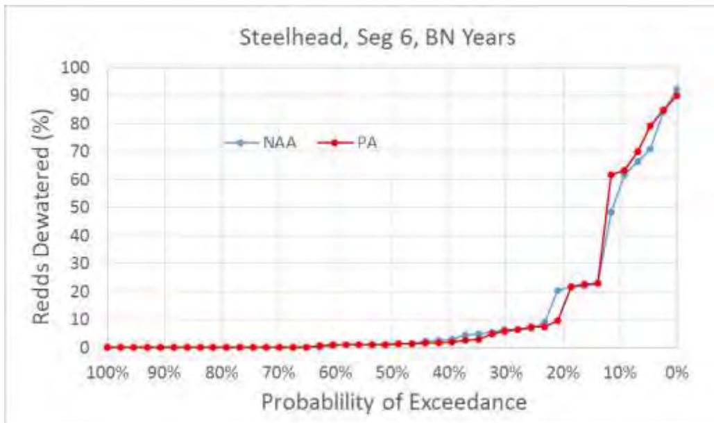
Figure 5.D-126. Exceedance Plot of Central Valley Steelhead Percent of Redds Dewatered for NAA and PA Model Scenarios in River Segment 6, Below Water Years
