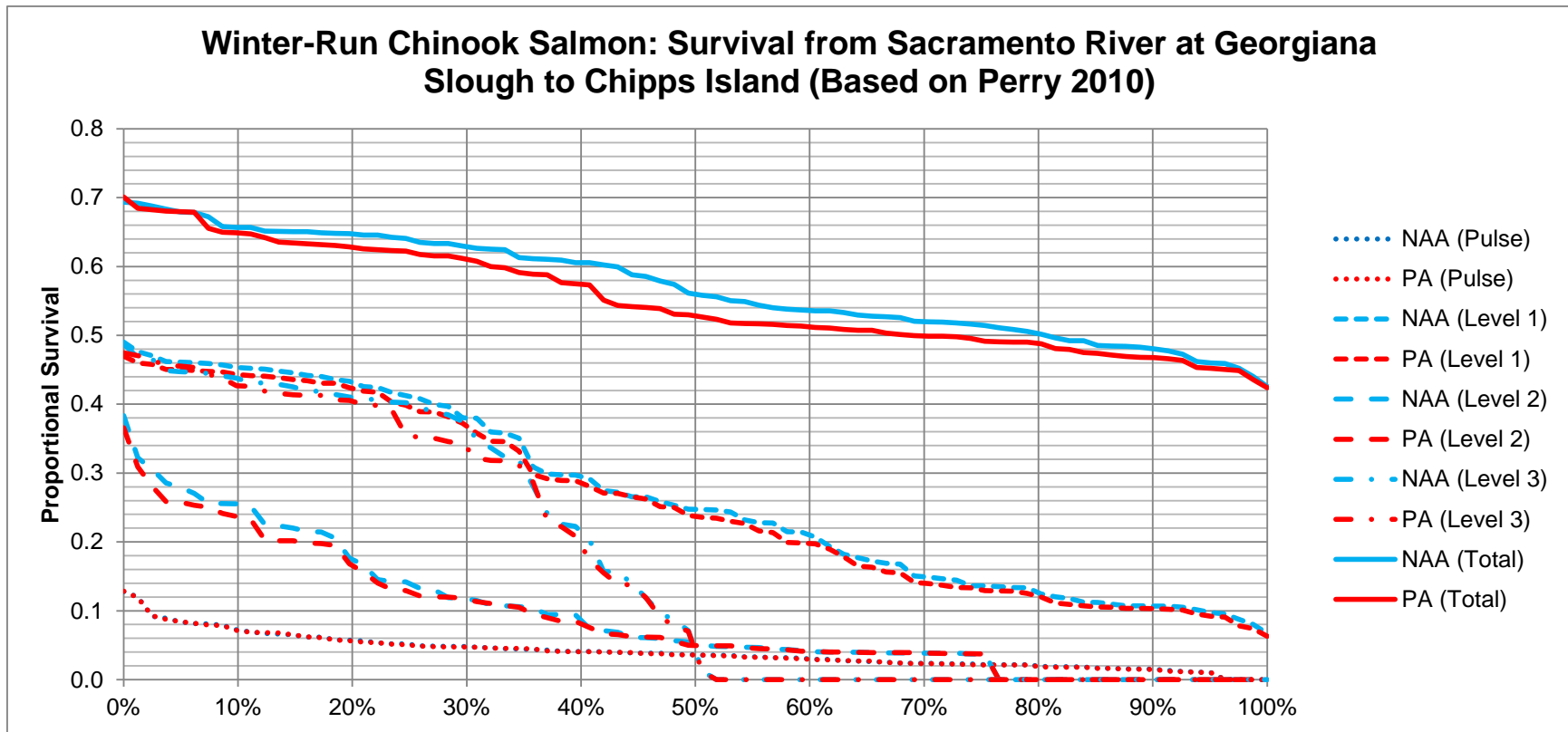
Figure 5.D-71. Exceedance Plot of Annual Juvenile Winter-Run Chinook Salmon Weighted Survival from the Sacramento River at Georgiana Slough to Chipps Island, Estimated from the Analysis Based on Perry (2010), By NDD Bypass Flow Level.
