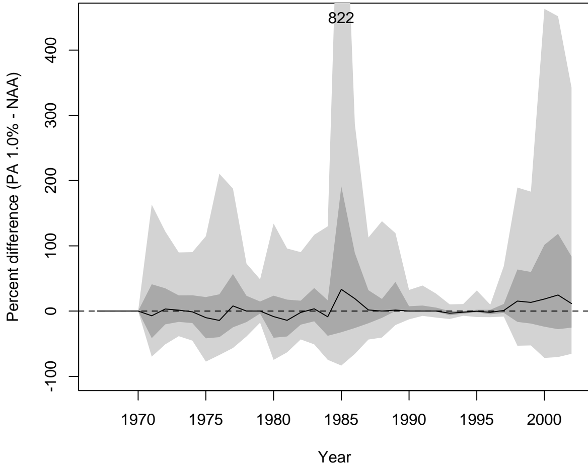
Figure 5.D-169. OBAN: Percent relative difference in escapement of PA 1.0% compared to NAA ( (PA\ 1.0\% - NAA)/NAA * 100\% ). Median (black line) 50% interval (dark grey) and 90% intervals (light gray) are plotted.
