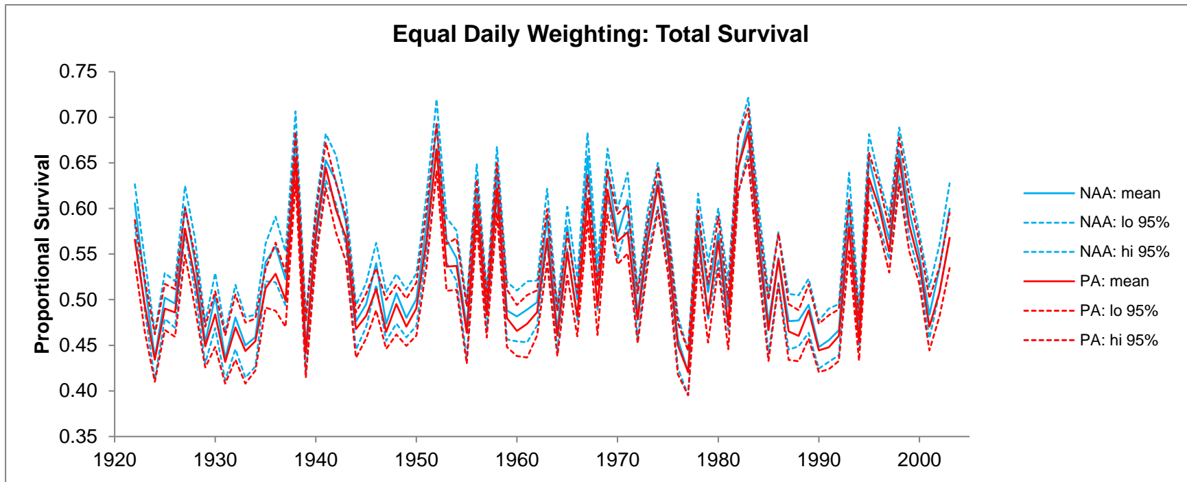
Figure 5.D-82. Time Series of Mean (With 95% Confidence Interval) Annual Juvenile Chinook Salmon Total Weighted Survival from the Sacramento River at Georgiana Slough to Chipps Island, Estimated from the Analysis Based on Perry (2010), Assuming Equal Daily Weighting from December to June.
