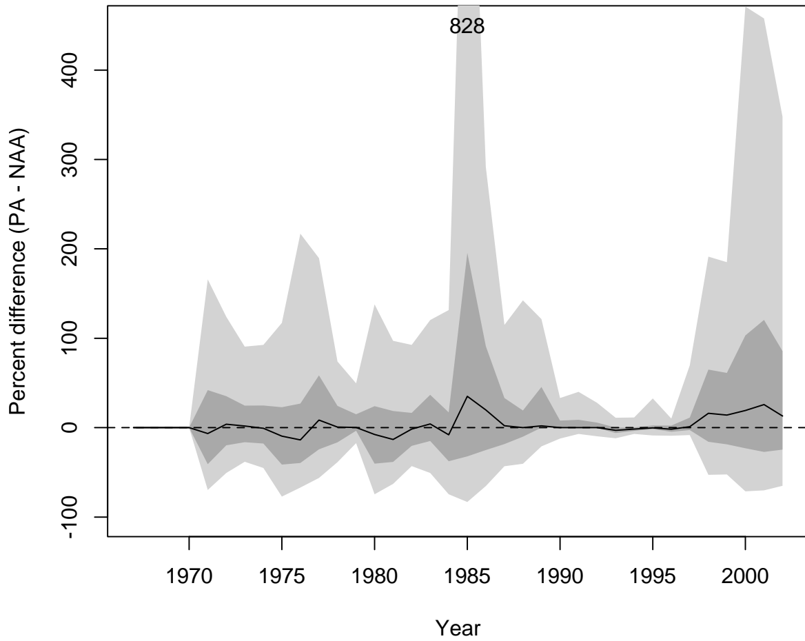
Figure 5.D-168. OBAN: Percent relative difference in escapement of PA compared to NAA ( (PA - NAA)/NAA * 100\% ). Median (black line) 50% interval (dark grey) and 90% intervals (light gray) are plotted.
