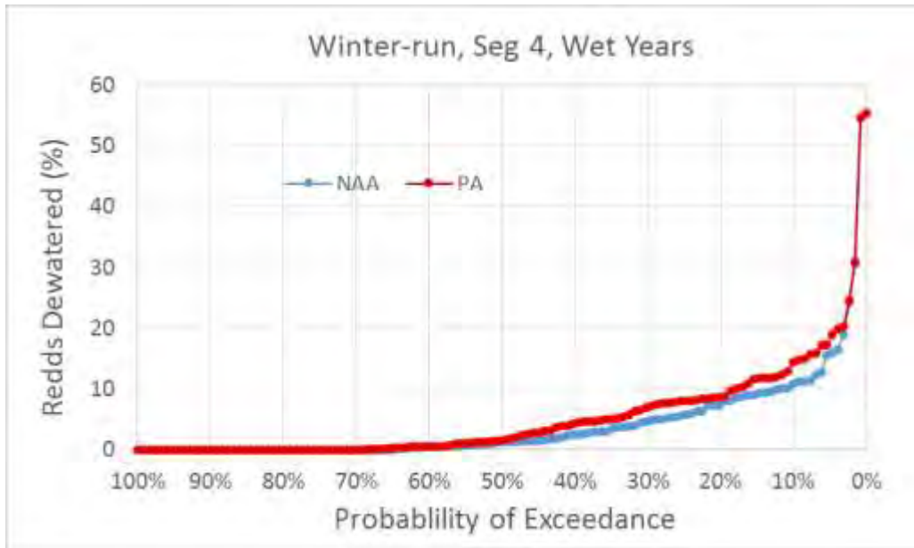
Figure 5.D-107. Exceedance Plot of Winter-Run Chinook Salmon Percent of Redds Dewatered for NAA and PA Model Scenarios in River Segment 4, Wet Water Years
