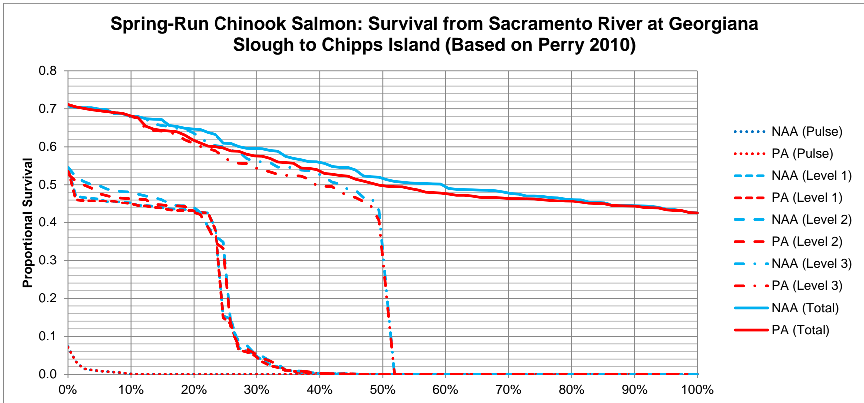
Figure 5.D-77. Exceedance Plot of Annual Juvenile Spring-Run Chinook Salmon Weighted Survival from the Sacramento River at Georgiana Slough to Chipps Island, Estimated from the Analysis Based on Perry (2010), By NDD Bypass Flow Level.
