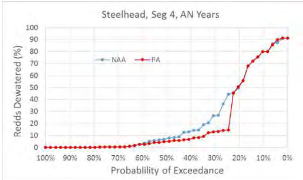
Figure 5.D-131. Exceedance Plot of Central Valley Steelhead Percent of Redds Dewatered for NAA and PA Model Scenarios in River Segment 4, Above Normal Water Years
