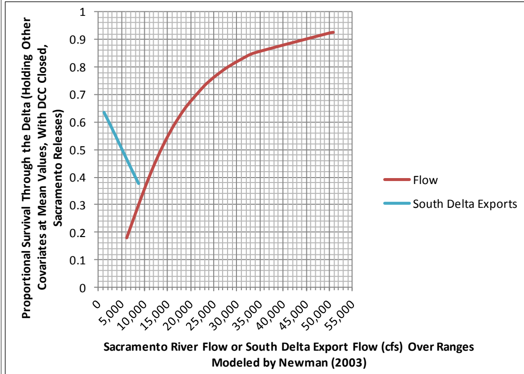
Figure 5.D-61. Effect Varying Sacramento River Flow and South Delta Exports Across the Range of Data Modeled by Newman (2003), Holding Other Covariates at Mean Values, Assuming Closed Delta Cross Channel Gates, and Fish Releases From Sacramento
