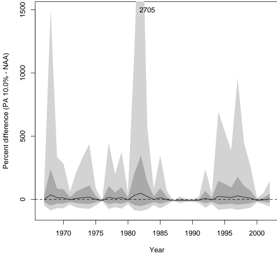
Figure 5.D-181. OBAN: Percent difference in Delta survival of PA 10.0% compared to NAA (PA 10.0% – NAA)/NAA*100%. Median (black line) 50% interval (dark grey) and 90% intervals (light gray) are plotted.
