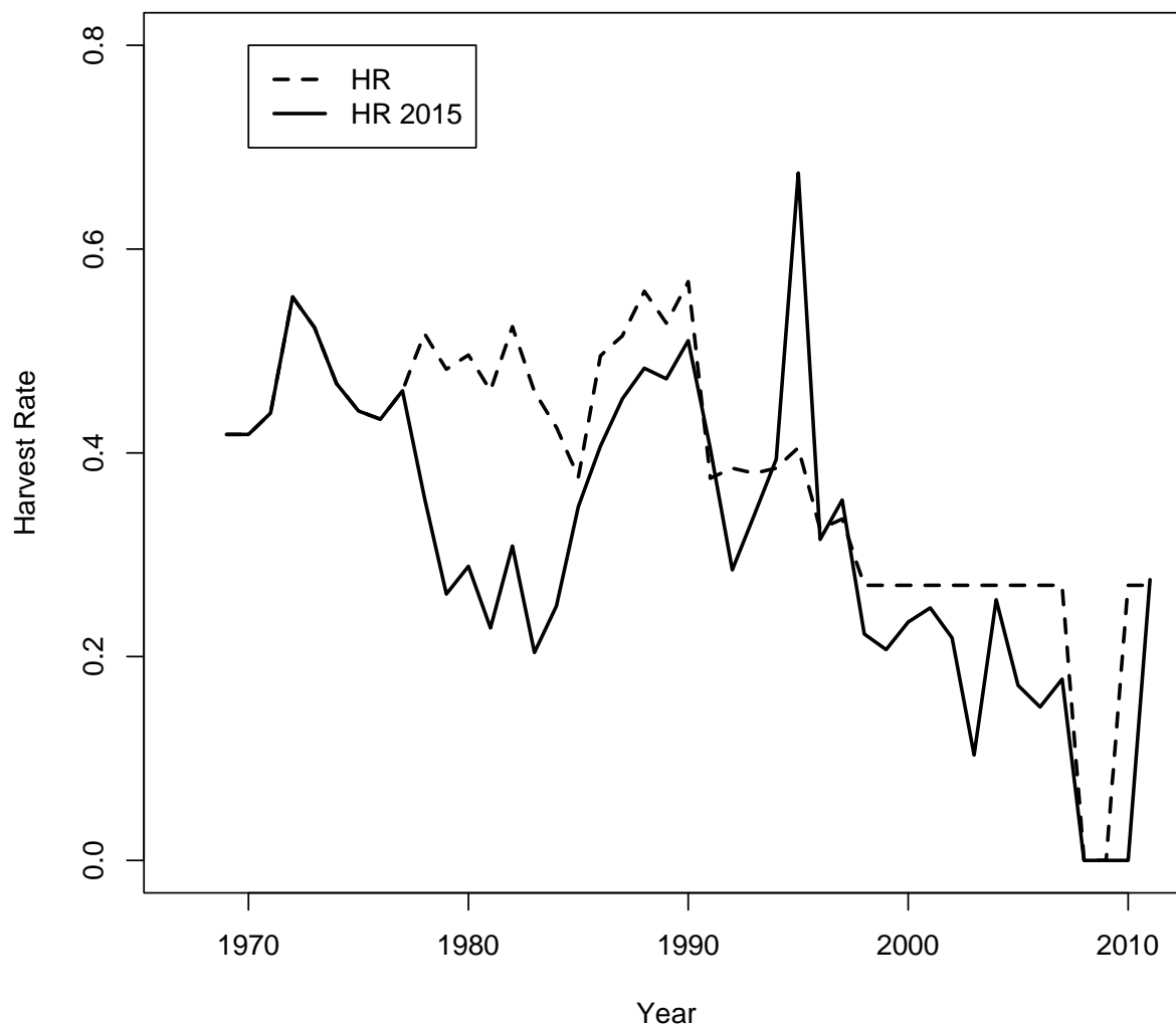
Figure 5.D-155. Estimated harvest rate (HR) using fishing regulations prior to 2015, and the harvest rate in 2015 using the hindcast of O’Farrell et al. (2012).
