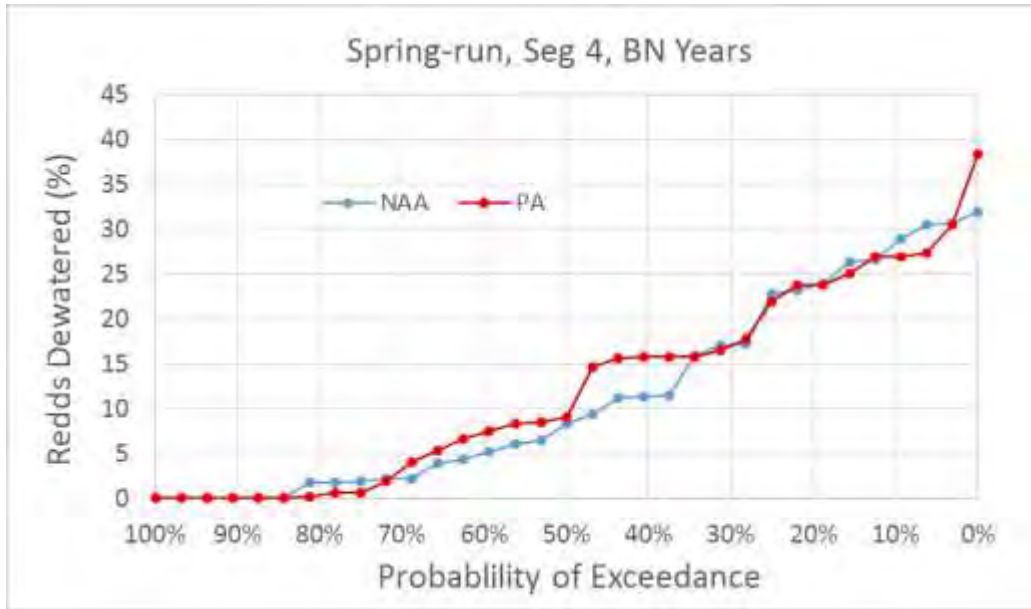
Figure 5.D-120. Exceedance Plot of Spring-Run Chinook Salmon Percent of Redds Dewatered for NAA and PA Model Scenarios in River Segment 4, Below Normal Water Years
