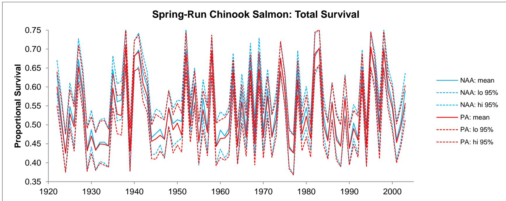
Figure 5.D-76. Time Series of Mean (With 95% Confidence Interval) Annual Juvenile Spring-Run Chinook Salmon Total Weighted Survival from the Sacramento River at Georgiana Slough to Chipps Island, Estimated from the Analysis Based on Perry (2010).
