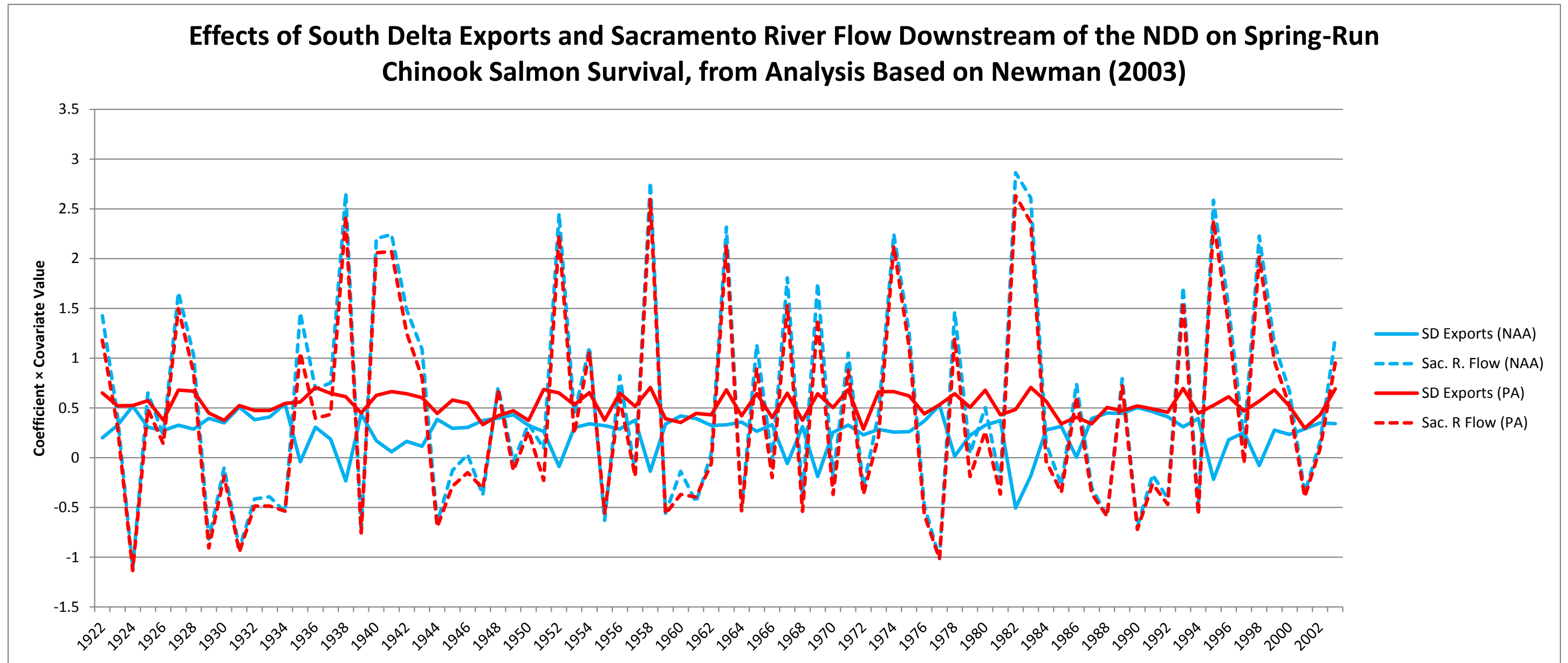
Figure 5.D-64. Relative Effect of South Delta Exports and Sacramento River Flow Downstream of the NDD on Spring-Run Chinook Salmon Survival.
