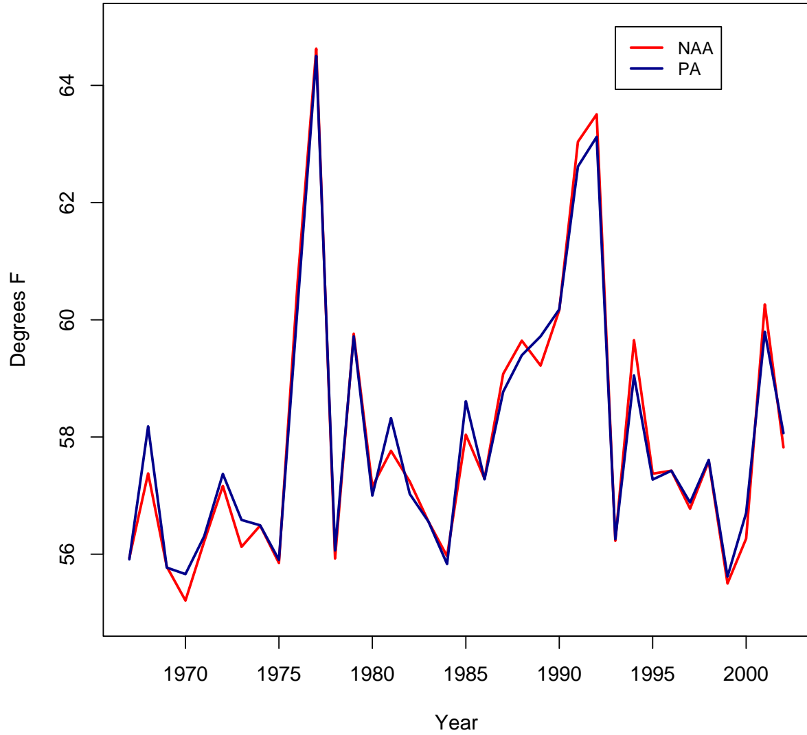
Figure 5.D-159. OBAN STEMP Covariate: Mean temperature from July to September at Bend Bridge.
