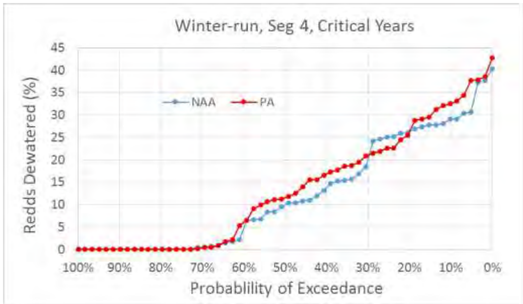
Figure 5.D-111. Exceedance Plot of Winter-Run Chinook Salmon Percent of Redds Dewatered for NAA and PA Model Scenarios in River Segment 4, Critical Water Years
