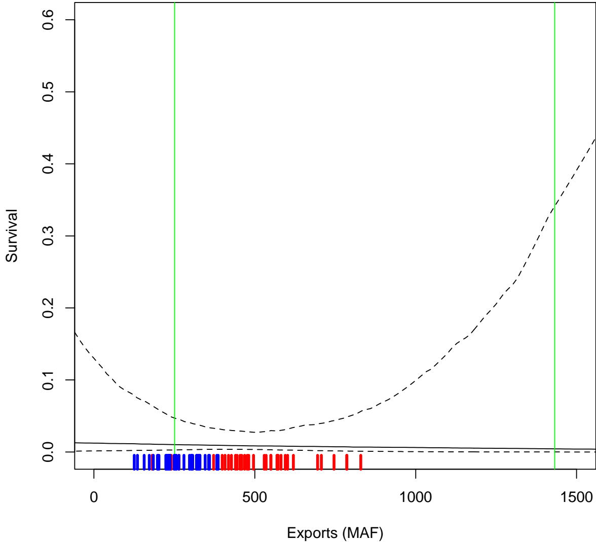
Figure 5.D-167. OBAN: Median relationship (solid black line) and 90% credible intervals (dashed black line) between south Delta exports and survival under 70 days of Yolo access (mean Yolo access under PA). Historical range of export data (vertical green lines) and the export levels under the NAA (red ticks) and PA (blue ticks).
