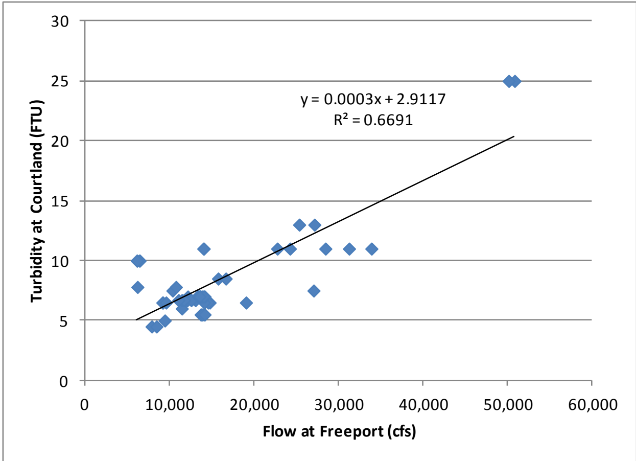
Figure 5.D-63. Relationship between Sacramento River Flow at Freeport and Turbidity at Courtland
