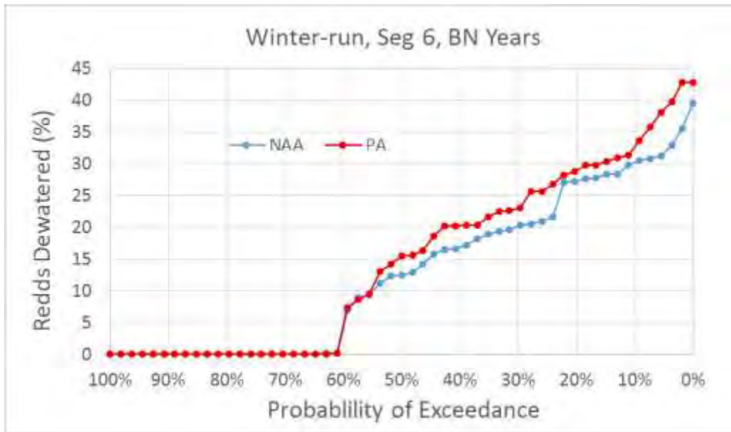
Figure 5.D-103. Exceedance Plot of Winter-Run Chinook Salmon Percent of Redds Dewatered for NAA and PA Model Scenarios in River Segment 6, Below Normal Water Years
