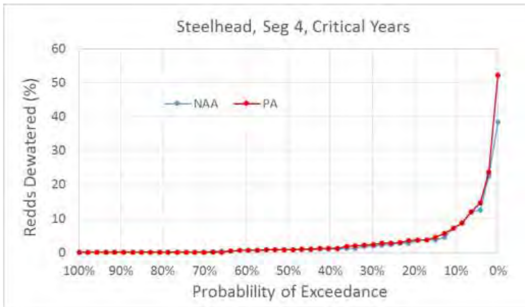
Figure 5.D-134. Exceedance Plot of Central Valley Steelhead Percent of Redds Dewatered for NAA and PA Model Scenarios in River Segment 4, Critical Water Years
