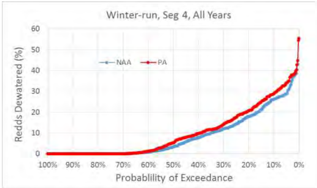
Figure 5.D-106. Exceedance Plot of Winter-Run Chinook Salmon Percent of Redds Dewatered for NAA and PA Model Scenarios in River Segment 4, All Water Years
