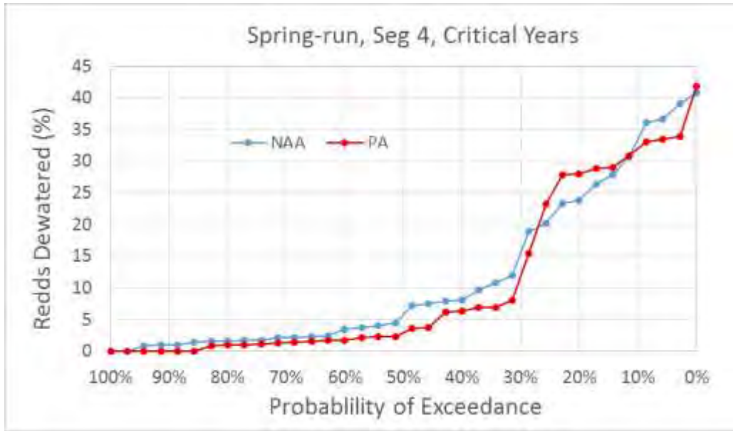
Figure 5.D-122. Exceedance Plot of Spring-Run Chinook Salmon Percent of Redds Dewatered for NAA and PA Model Scenarios in River Segment 4, Critical Water Years
