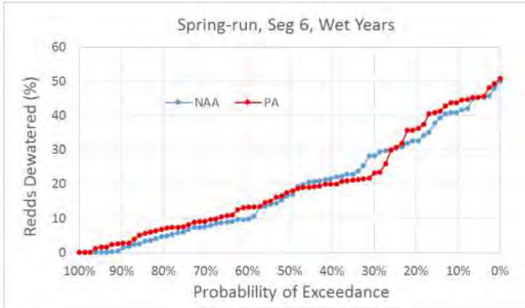
Figure 5.D-113. Exceedance Plot of Spring-Run Chinook Salmon Percent of Redds Dewatered for NAA and PA Model Scenarios in River Segment 6, Wet Water Years
