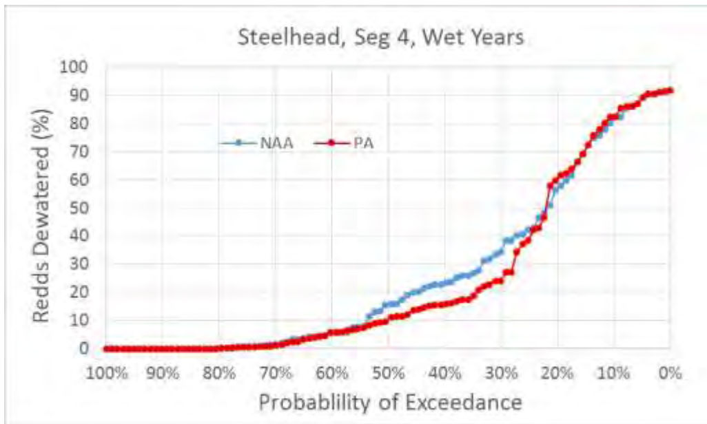
Figure 5.D-130. Exceedance Plot of Central Valley Steelhead Percent of Redds Dewatered for NAA and PA Model Scenarios in River Segment 4, Wet Water Years
