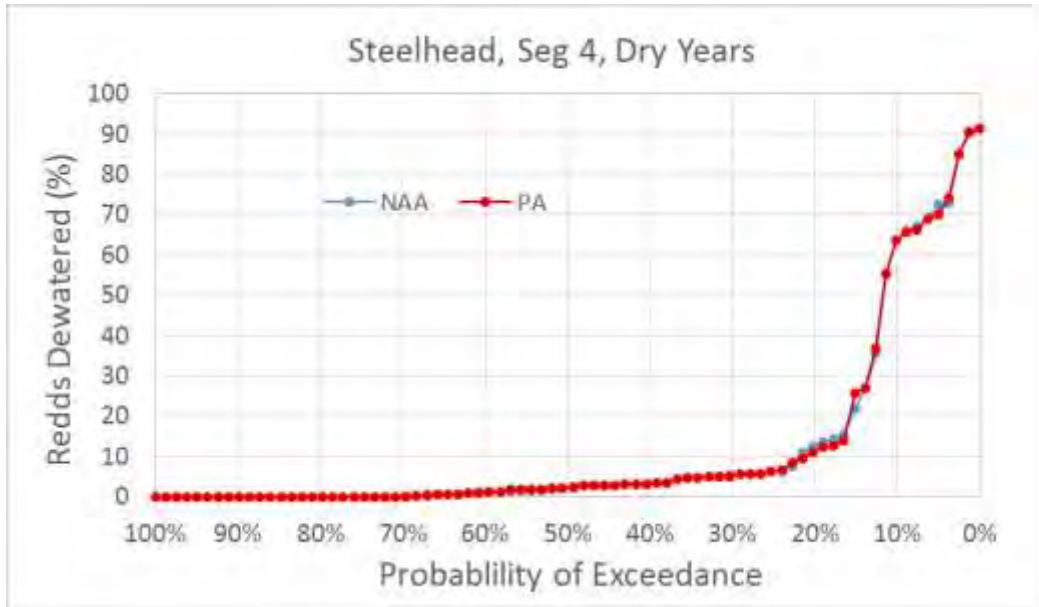
Figure 5.D-133. Exceedance Plot of Central Valley Steelhead Percent of Redds Dewatered for NAA and PA Model Scenarios in River Segment 4, Dry Water Years
