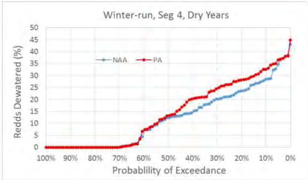
Figure 5.D-110. Exceedance Plot of Winter-Run Chinook Salmon Percent of Redds Dewatered for NAA and PA Model Scenarios in River Segment 4, Dry Water Years
