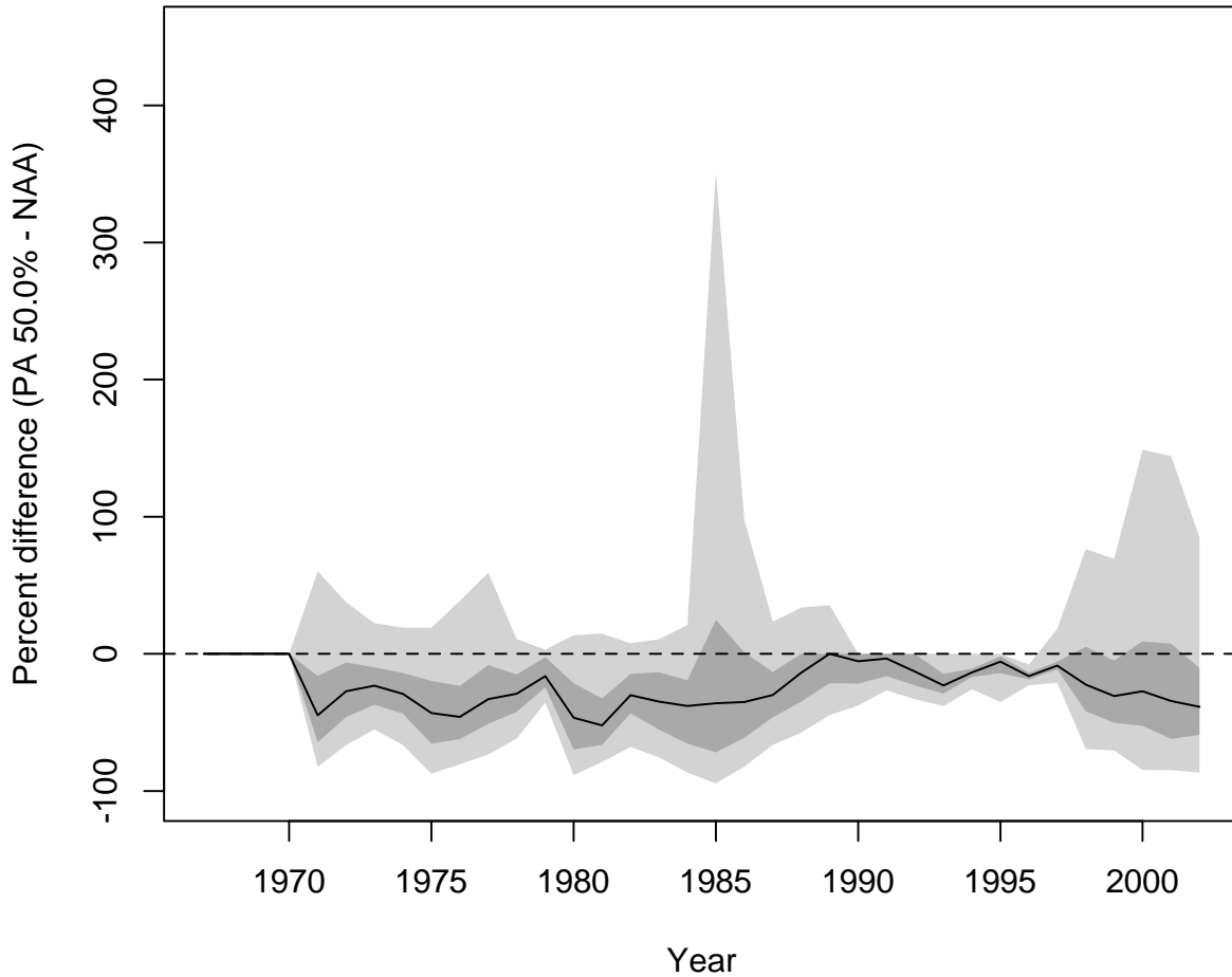
Figure 5.D-172. OBAN: Percent relative difference in escapement of PA 50.0% compared to NAA ( (PA\ 50.0\% - NAA)/NAA * 100\% ). Median (black line) 50% interval (dark grey) and 90% intervals (light gray) are plotted.
