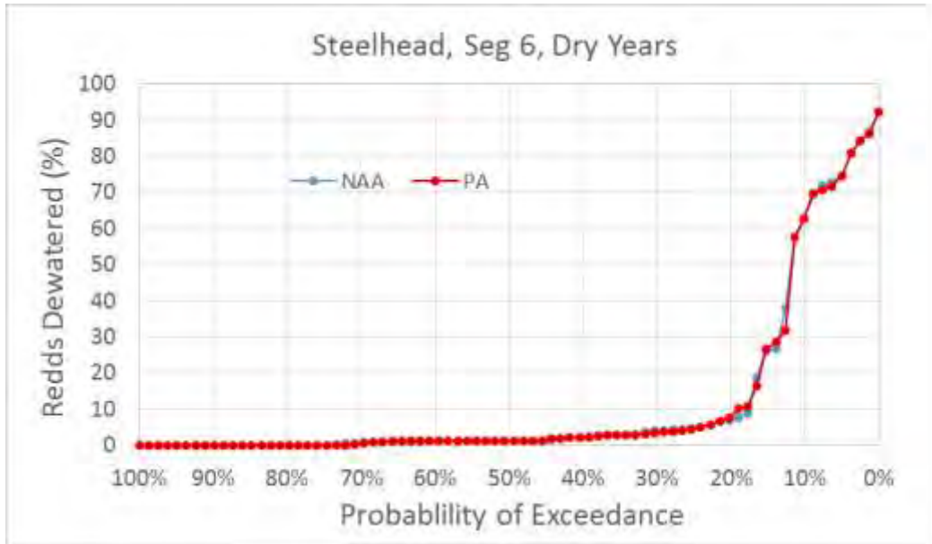
Figure 5.D-127. Exceedance Plot of Central Valley Steelhead Percent of Redds Dewatered for NAA and PA Model Scenarios in River Segment 6, Dry Water Years
