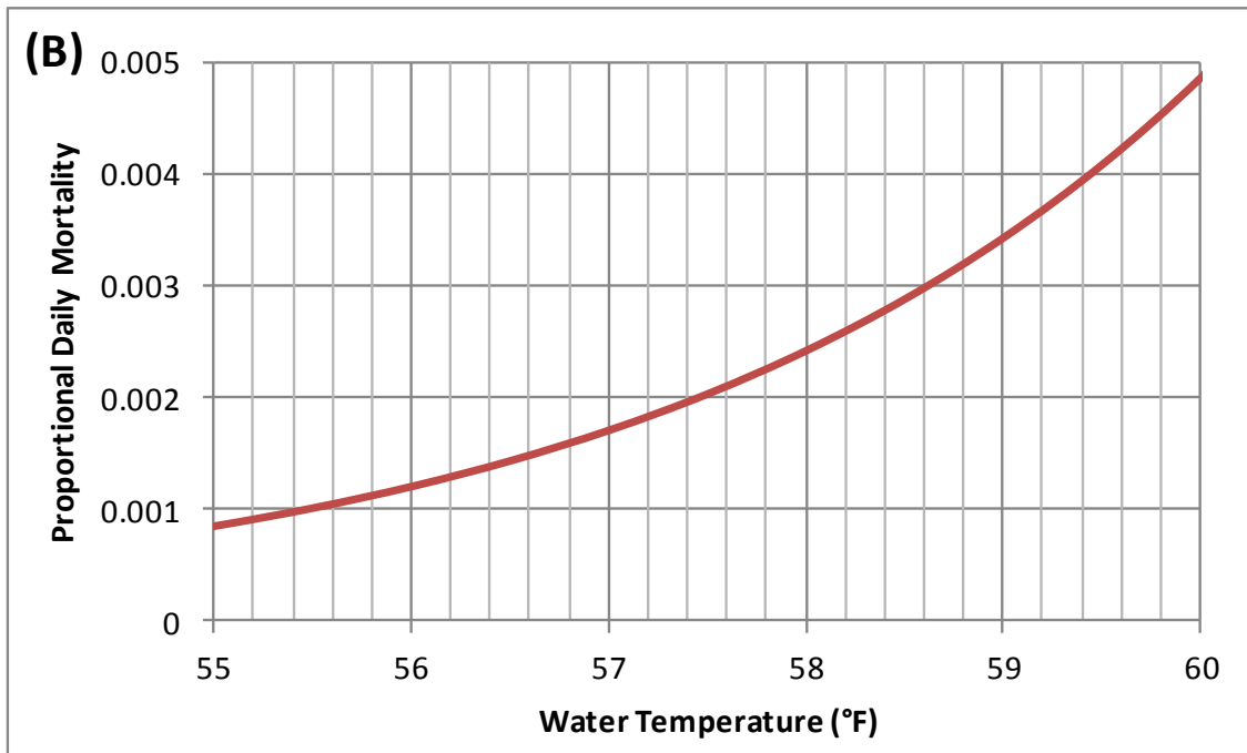
Figure 5.D-137. Relationship between Proportional Daily Mortality of Winter-Run Chinook Salmon Fry and Water Temperature (Equation 8) for (A) the Entire Temperature Range, and (B) the Predominant Range Found in Model Scenarios
