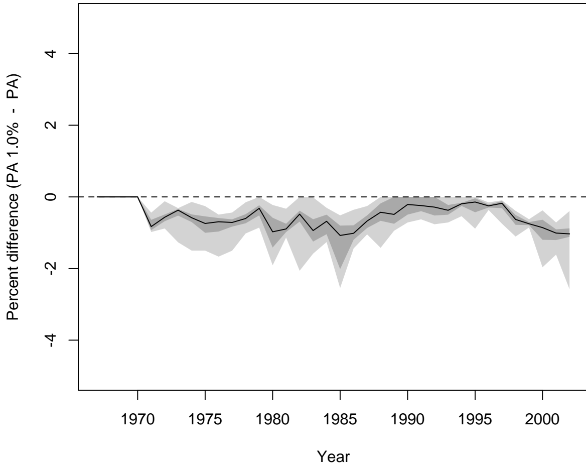
Figure 5.D-173. OBAN: Percent relative difference in escapement of PA 1.0% compared to PA (PA\ 1.0\% - PA)/PA * 100\% . Median (black line) 50% interval (dark grey) and 90% intervals (light gray) are plotted.
