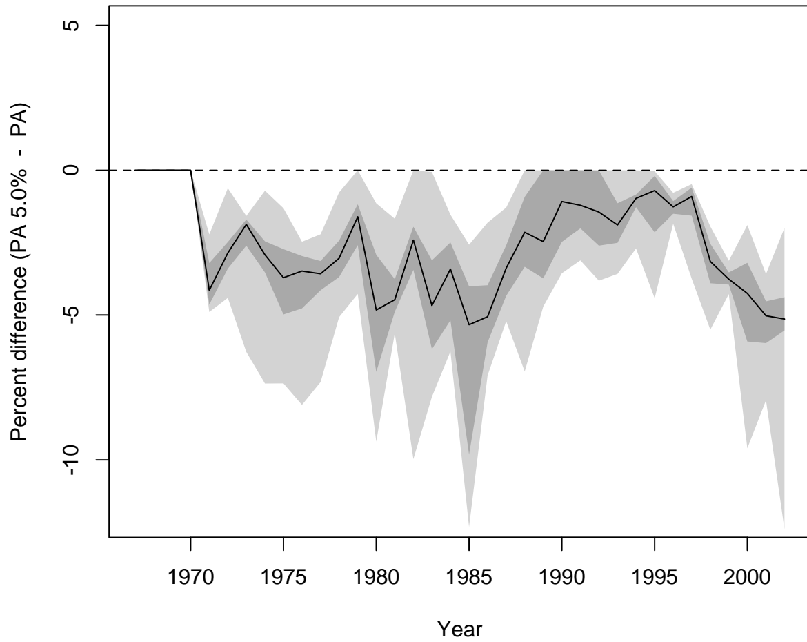
Figure 5.D-174. OBAN: Percent relative difference in escapement of PA 5.0% compared to PA (PA\ 5.0\% - PA)/PA * 100\% . Median (black line) 50% interval (dark grey) and 90% intervals (light gray) are plotted.
