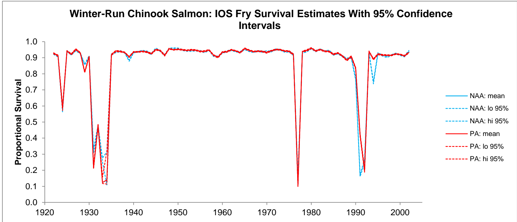
Figure 5.D-145. IOS Annual Winter-Run Chinook Salmon Fry Survival Estimates with 95% Confidence Intervals.
