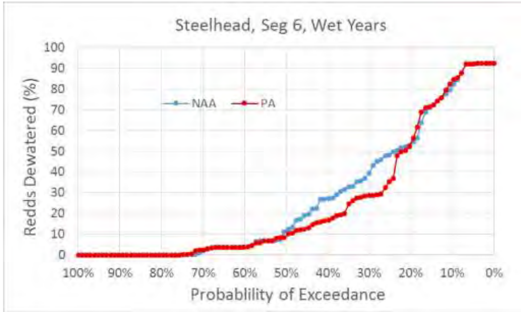
Figure 5.D-124. Exceedance Plot of Central Valley Steelhead Percent of Redds Dewatered for NAA and PA Model Scenarios in River Segment 6, Wet Water Years
