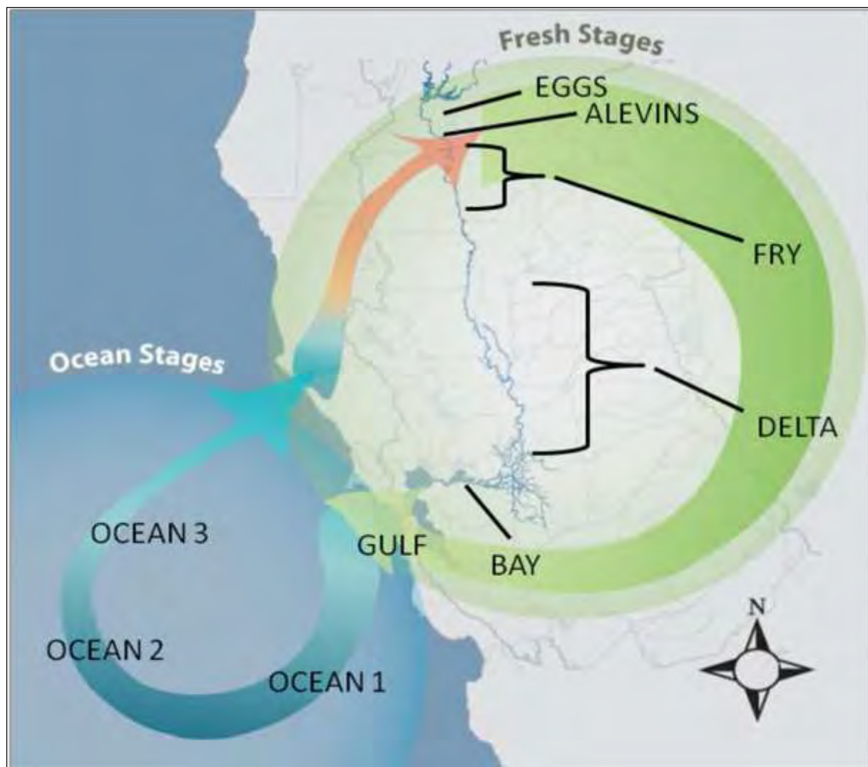
Figure 5.D-152. Winter-Run Chinook Salmon Life History Stages Used in the OBAN Model
