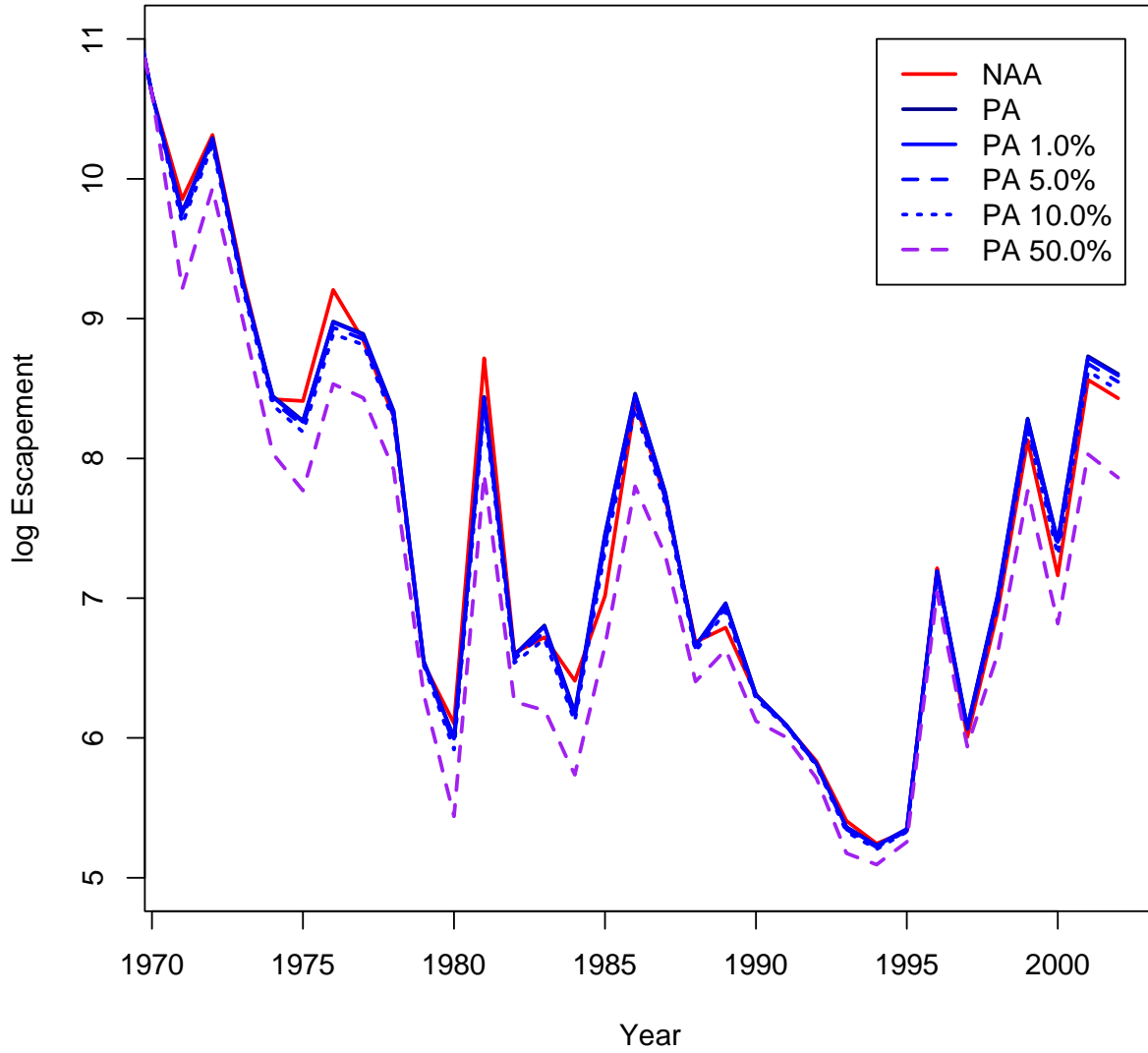
Figure 5.D-163. OBAN: Median log escapement for each of the scenarios.
