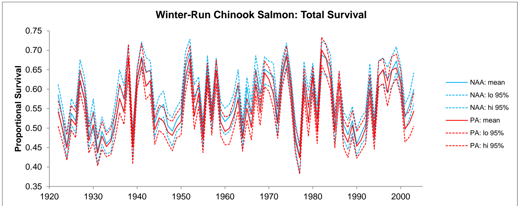
Figure 5.D-70. Time Series of Mean (With 95% Confidence Interval) Annual Juvenile Winter-Run Chinook Salmon Total Weighted Survival from the Sacramento River at Georgiana Slough to Chipps Island, Estimated from the Analysis Based on Perry (2010).
