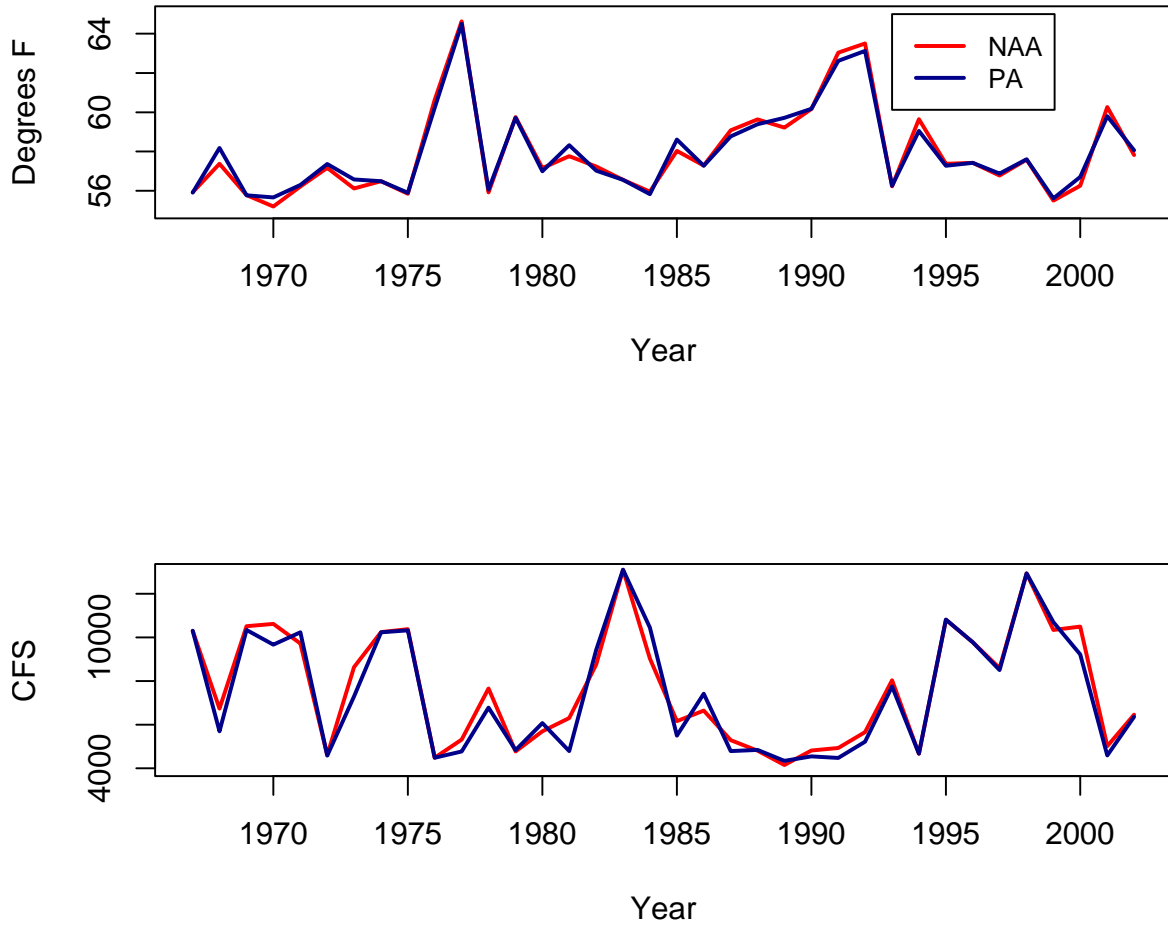
Figure 5.D-164. OBAN: Mean temperature from July to September at Bend Bridge (top) and minimum of monthly average flow between August and November at Bend Bridge in cubic feet per second (CFS) (bottom).
