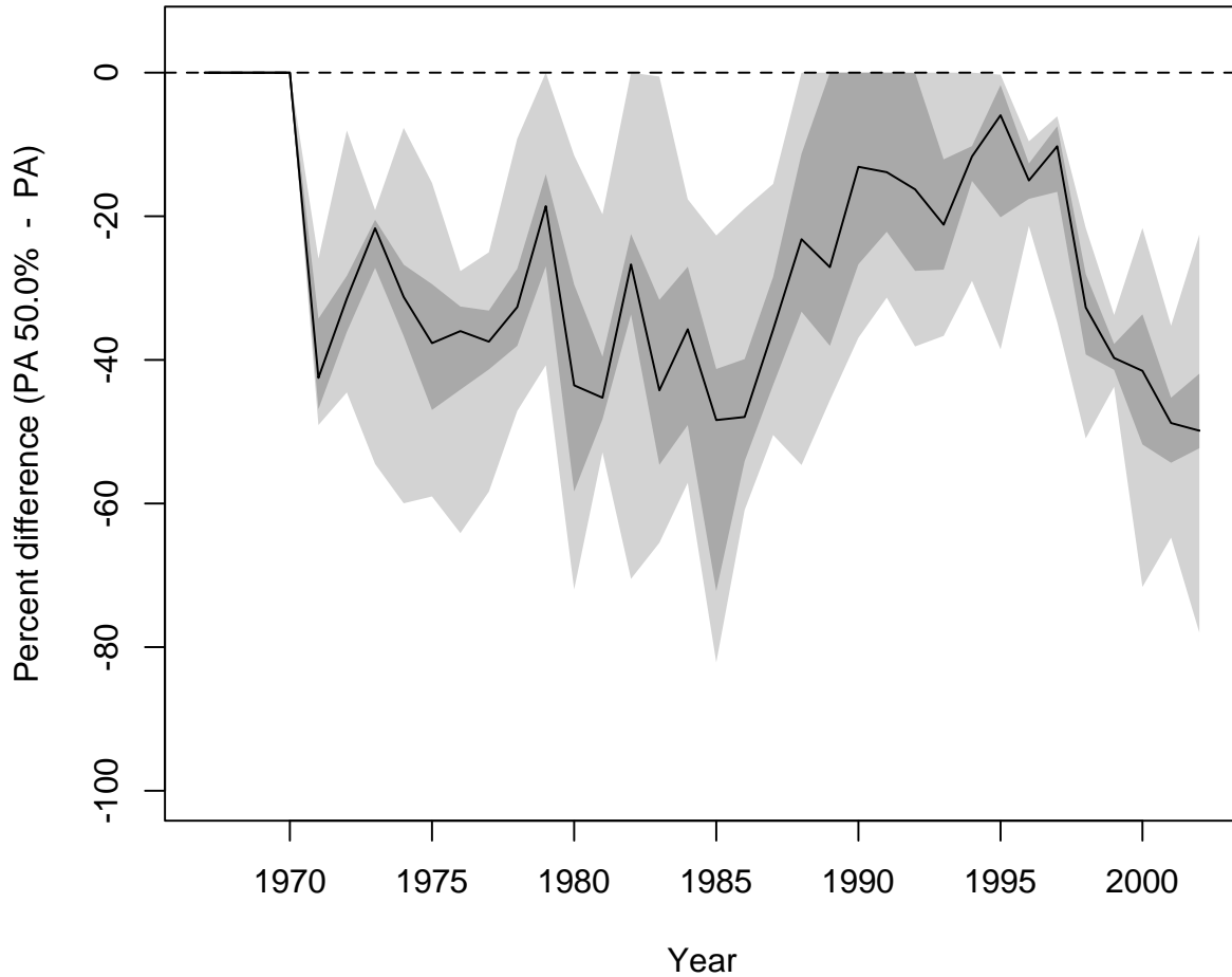
Figure 5.D-176. OBAN: Percent relative difference in escapement of PA 50.0% compared to PA ( (PA\ 50.0\% - PA)/PA * 100\% ). Median (black line) 50% interval (dark grey) and 90% intervals (light gray) are plotted.
