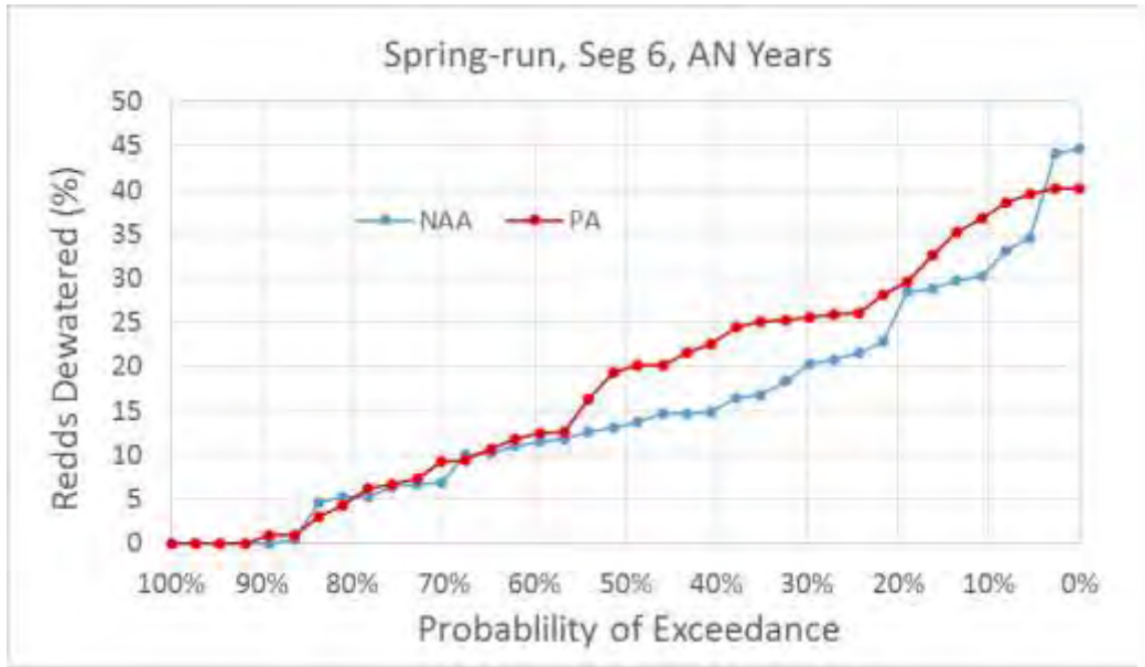
Figure 5.D-114. Exceedance Plot of Spring-Run Chinook Salmon Percent of Redds Dewatered for NAA and PA Model Scenarios in River Segment 6, Above Normal Water Years
