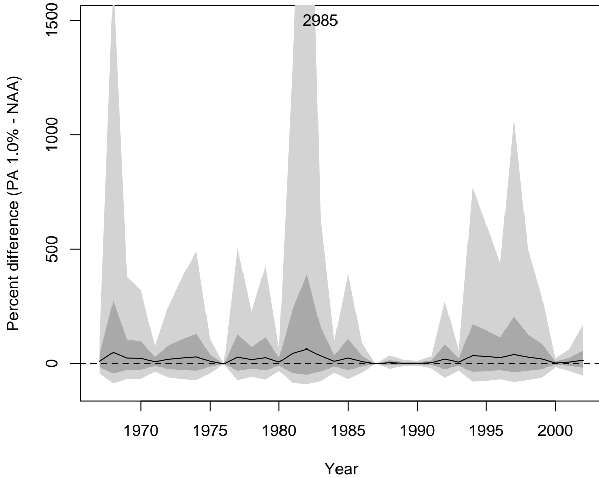
Figure 5.D-179. OBAN: Percent difference in Delta survival of PA 1.0% compared to NAA (PA 1.0% – NAA)/NAA*100%. Median (black line) 50% interval (dark grey) and 90% intervals (light gray) are plotted.
