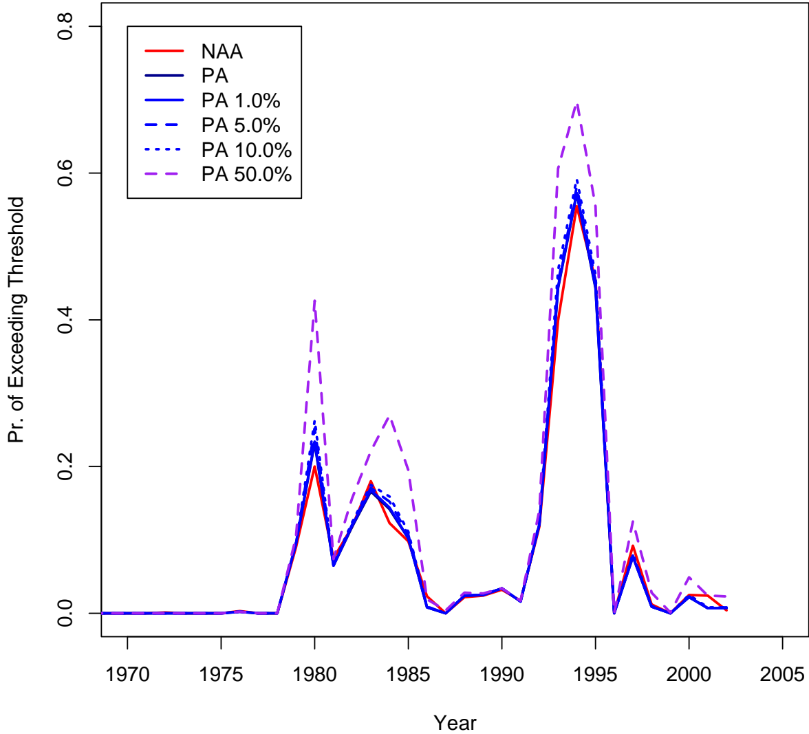
Figure 5.D-165. OBAN: Probability of exceeding quasi-extinction threshold of 200 spawners for each scenario.
