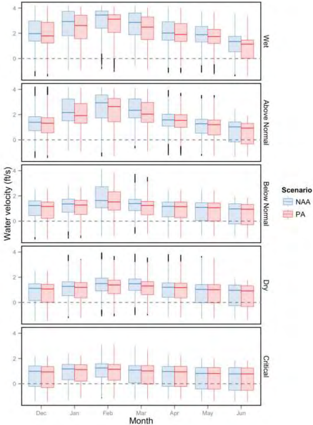
Figure 5.D-7. Velocity of flow entering the interior delta at channel 383, Sutter Slough, during the 82-year CALSIM period. Comparisons between the NAA (NAA) and the PA (PA) were performed for the months of
