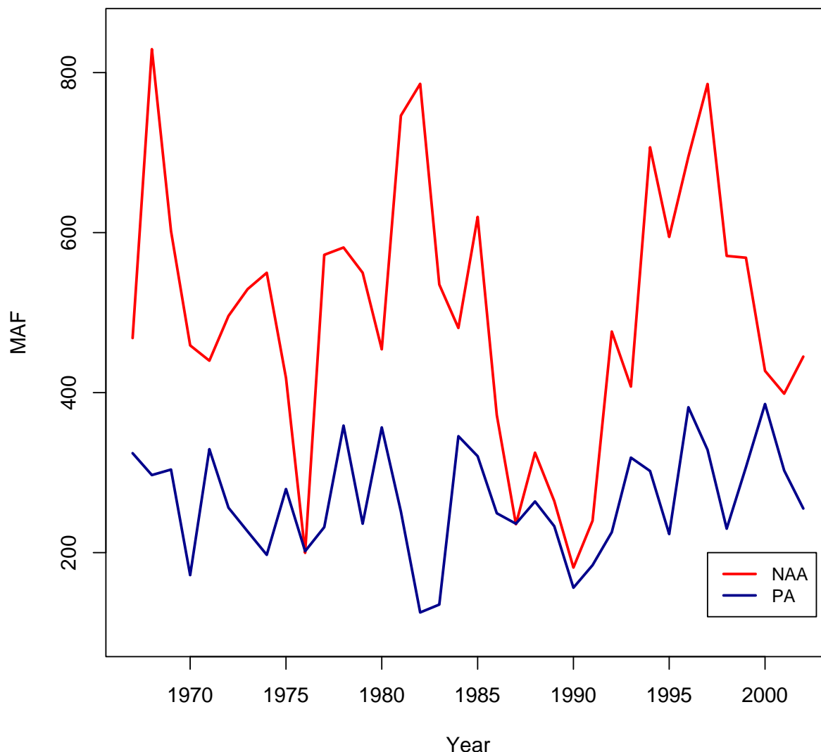
Figure 5.D-161. OBAN EXPT Covariate: Total South Delta exports from December to June in million acre feet (MAF).
