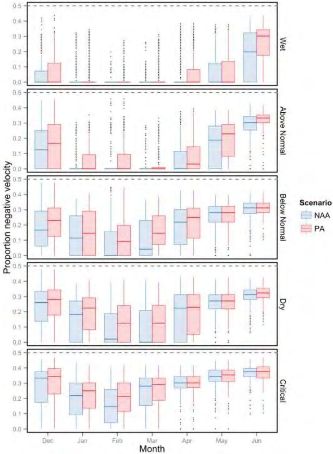
Figure 5.D-27. Daily proportion of negative velocity entering the interior at delta Channel 383, Sutter Slough, during the 82-year CALSIM period. Comparisons between the NAA (NAA) and the PA (PA) were performed
