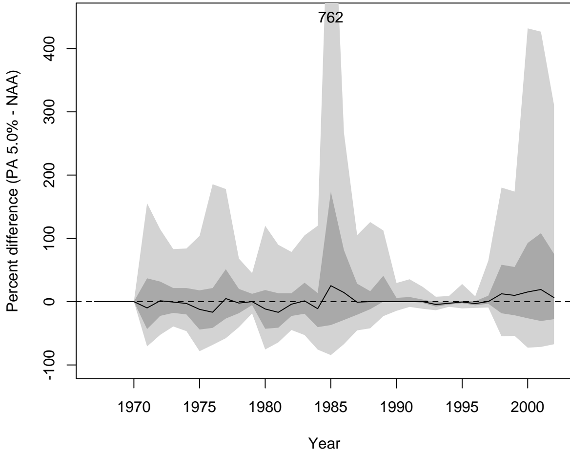
Figure 5.D-170. OBAN: Percent relative difference in escapement of PA 5.0% compared to NAA ( (PA\ 5.0\% - NAA)/NAA * 100\% ). Median (black line) 50% interval (dark grey) and 90% intervals (light gray) are plotted.
