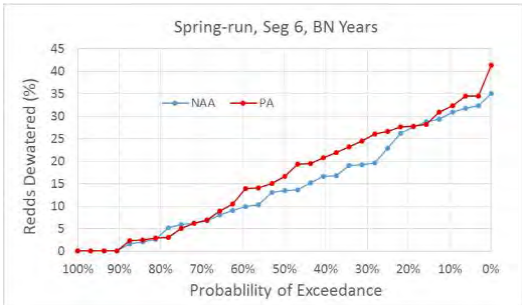
Figure 5.D-115. Exceedance Plot of Spring-Run Chinook Salmon Percent of Redds Dewatered for NAA and PA Model Scenarios in River Segment 6, Below Normal Water Years
