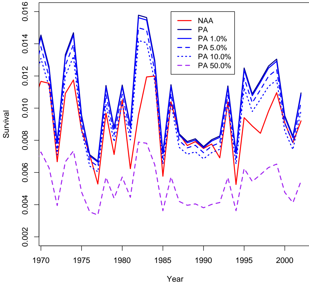
Figure 5.D-177. OBAN: Median Delta survival for each of the scenarios.
