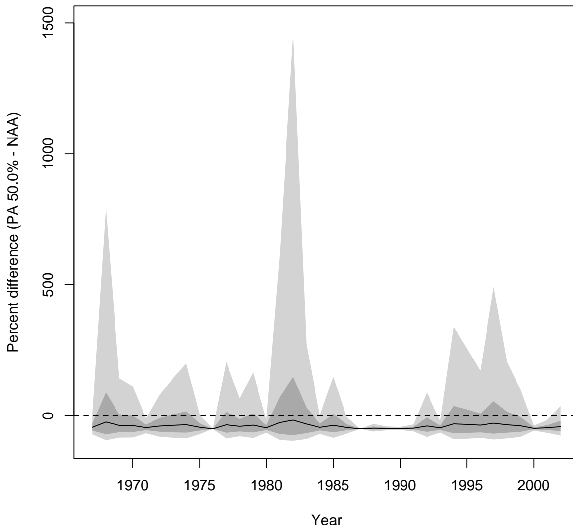
Figure 5.D-182. OBAN: Percent difference in Delta survival of PA 50.0% compared to NAA (PA 50.0% – NAA)/NAA*100%. Median (black line) 50% interval (dark grey) and 90% intervals (light grey) are plotted.
