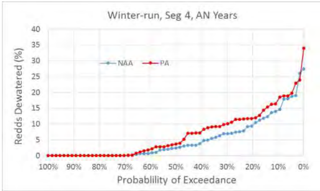
Figure 5.D-108. Exceedance Plot of Winter-Run Chinook Salmon Percent of Redds Dewatered for NAA and PA Model Scenarios in River Segment 4, Above Normal Water Years
