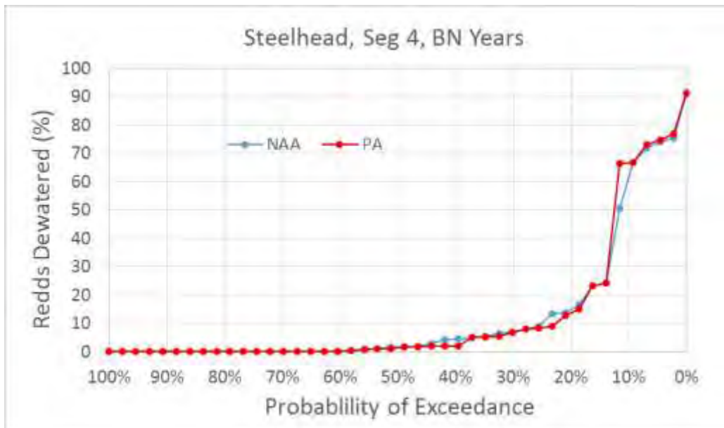
Figure 5.D-132. Exceedance Plot of Central Valley Steelhead Percent of Redds Dewatered for NAA and PA Model Scenarios in River Segment 4, Below Water Years
