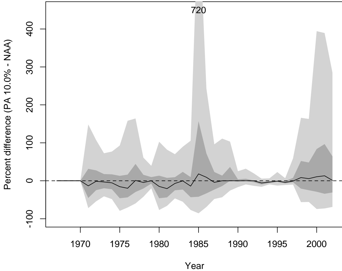
Figure 5.D-171. OBAN: Percent relative difference in escapement of PA 10.0% compared to NAA (PA\ 10.0\% - NAA)/NAA * 100\% . Median (black line) 50% interval (dark grey) and 90% intervals (light gray) are plotted.
