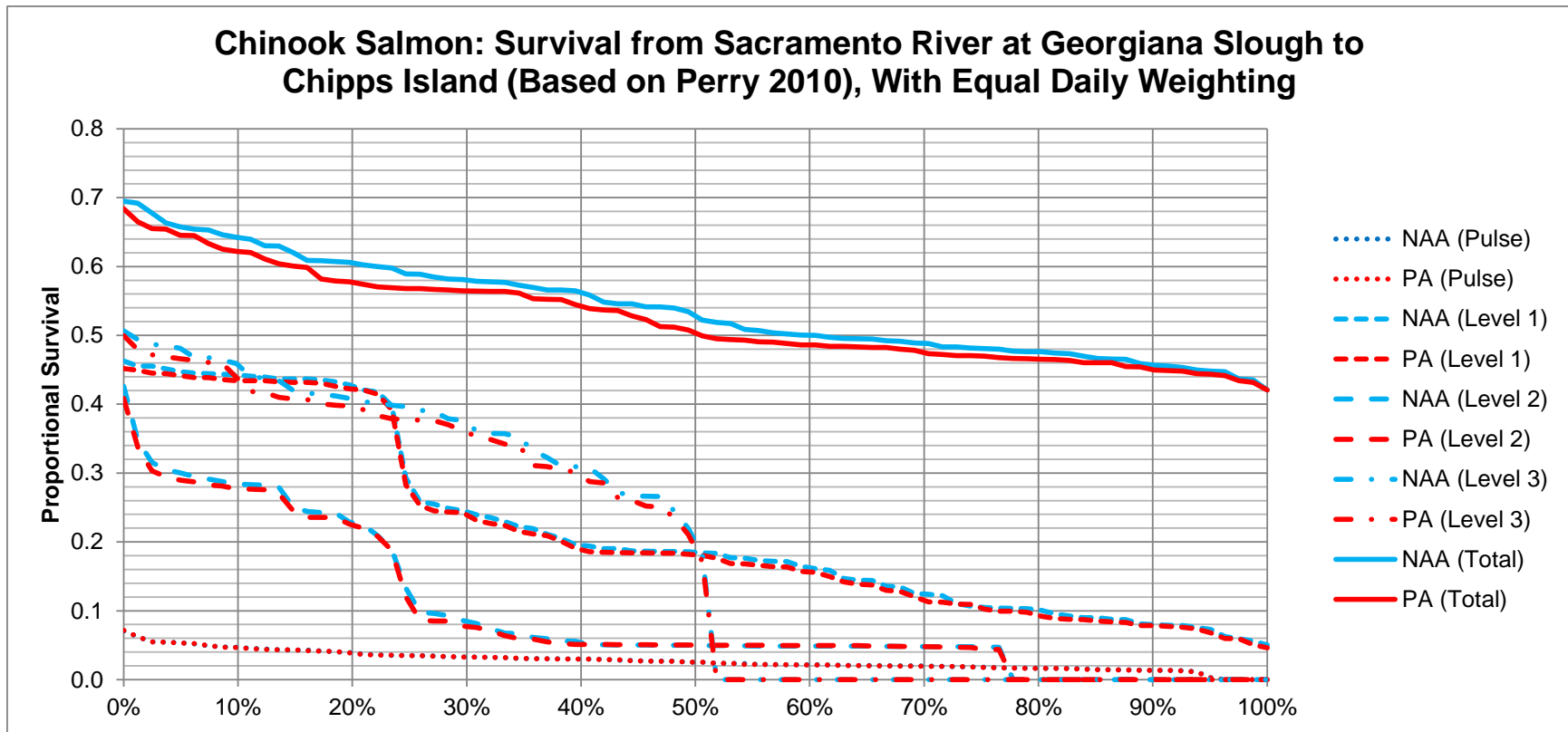
Figure 5.D-83. Exceedance Plot of Annual Juvenile Chinook Salmon Weighted Survival from the Sacramento River at Georgiana Slough to Chipps Island, Estimated from the Analysis Based on Perry (2010), By NDD Bypass Flow Level and Assuming Equal Daily Weighting from December to June.
