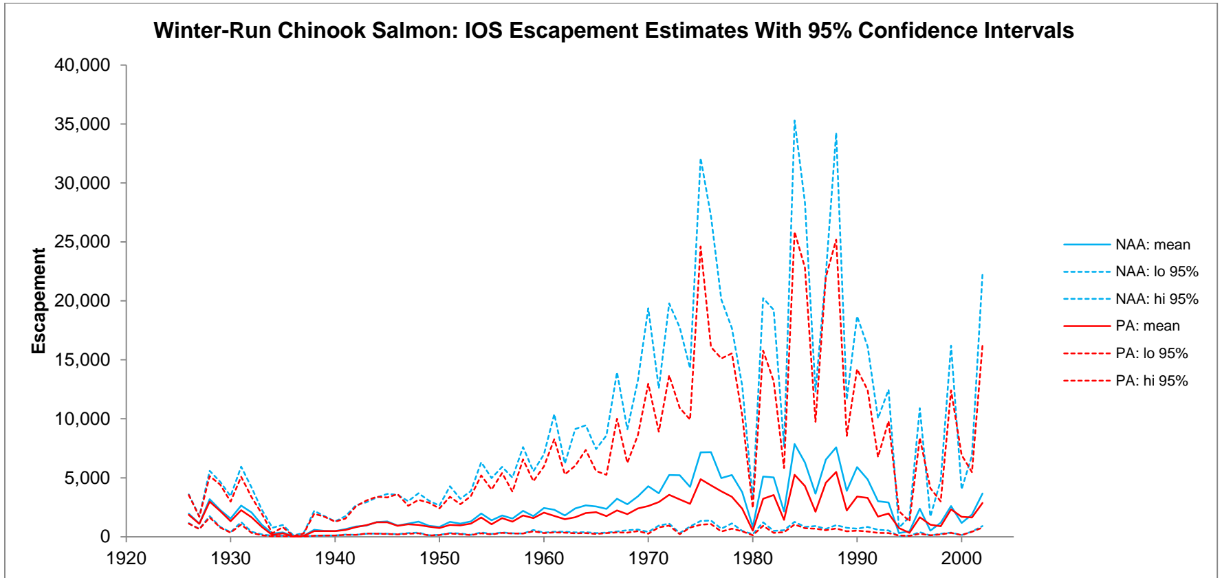
Figure 5.D-151. IOS Annual Winter-Run Chinook Salmon Escapement Estimates with 95% Confidence Intervals.
