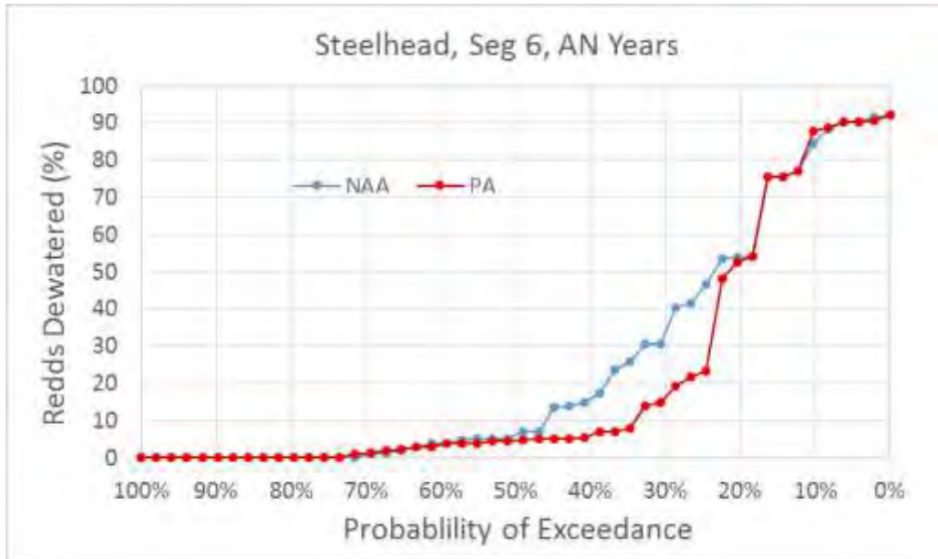
Figure 5.D-125. Exceedance Plot of Central Valley Steelhead Percent of Redds Dewatered for NAA and PA Model Scenarios in River Segment 6, Above Normal Water Years
