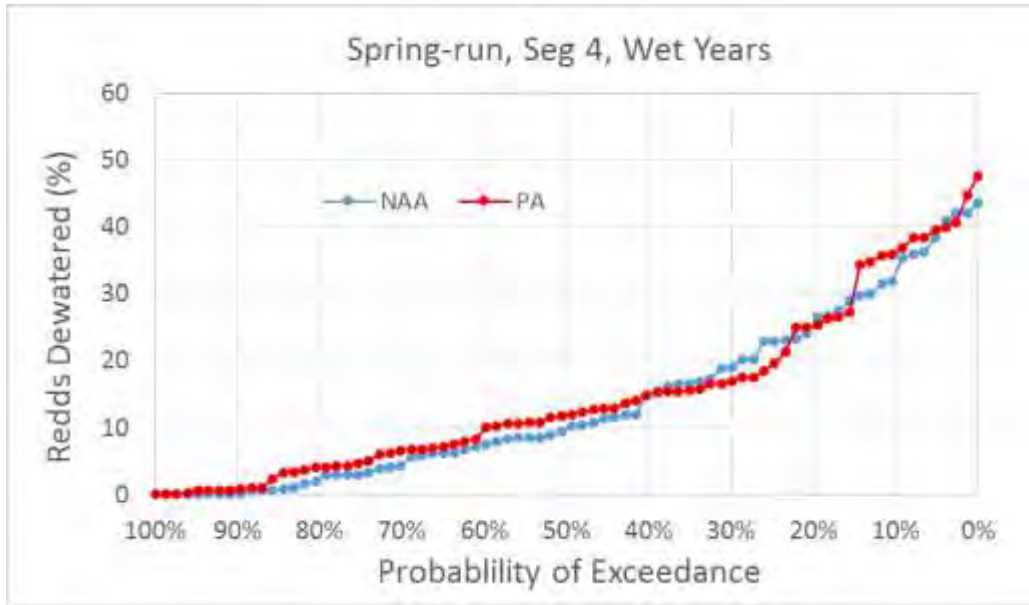
Figure 5.D-118. Exceedance Plot of Spring-Run Chinook Salmon Percent of Redds Dewatered for NAA and PA Model Scenarios in River Segment 4, Wet Water Years
