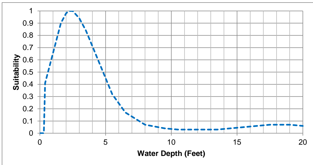
Figure 5.D-85. Habitat Suitability Curve for Juvenile Chinook Salmon.
