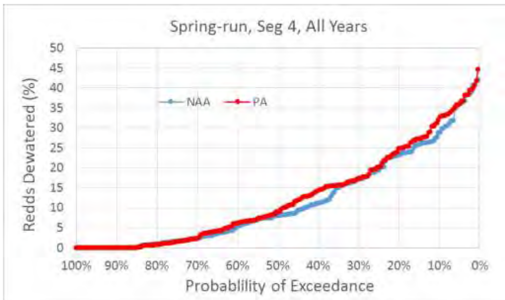
Figure 5.D-117. Exceedance Plot of Spring-Run Chinook Salmon Percent of Redds Dewatered for NAA and PA Model Scenarios in River Segment 4, All Water Years
