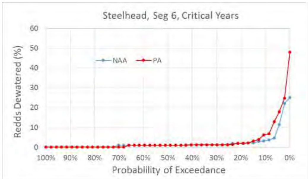
Figure 5.D-128. Exceedance Plot of Central Valley Steelhead Percent of Redds Dewatered for NAA and PA Model Scenarios in River Segment 6, Critical Water Years
