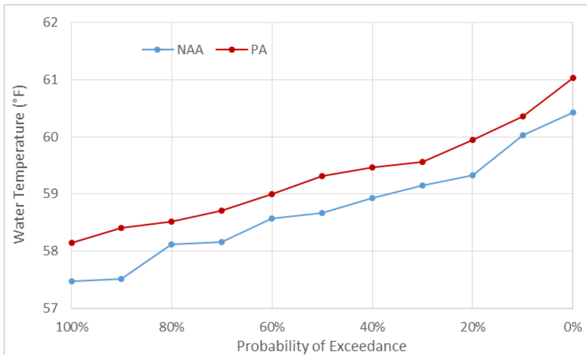
Figure 5.4-107. Exceedance Plot of Mean Monthly Water Temperatures (°F) in the Sacramento River at Red Bluff in August of Below Normal Water Years
