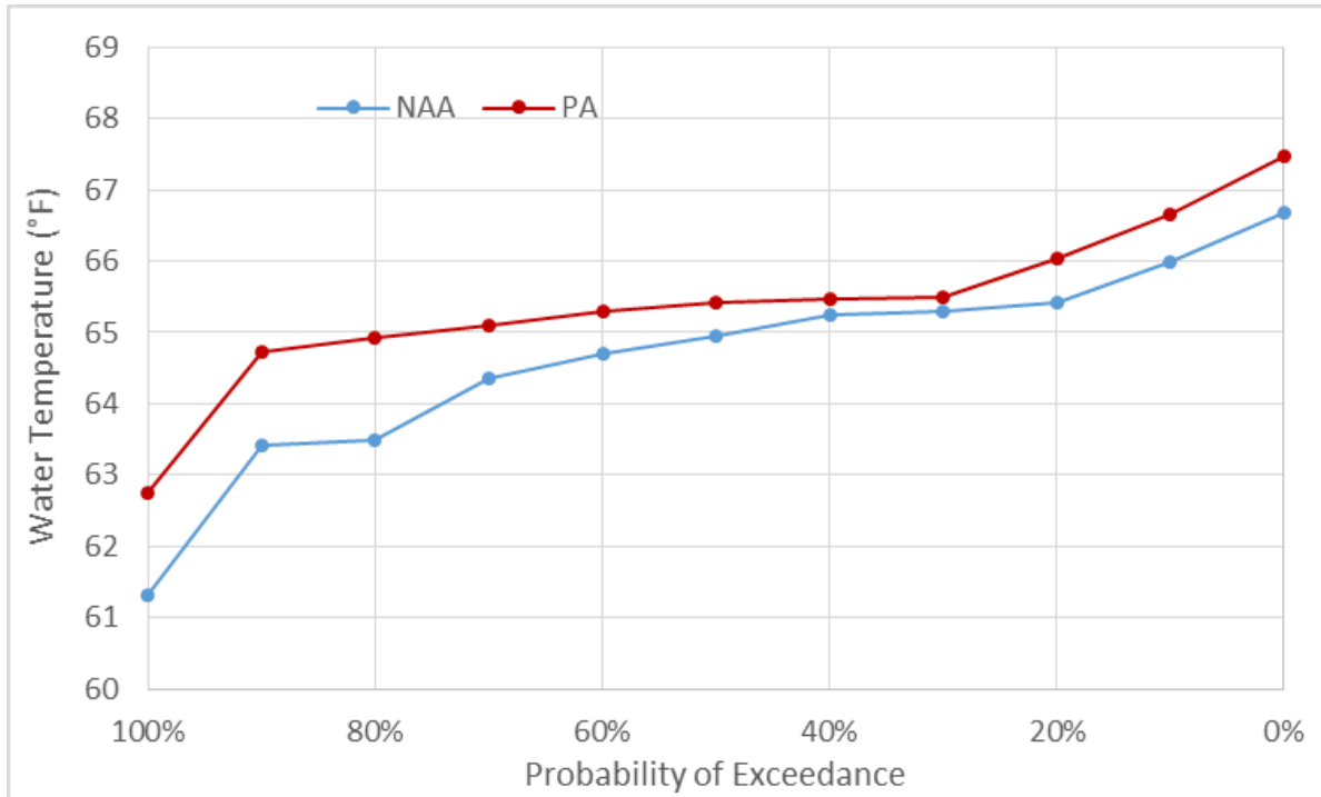
Figure 5.4-247. Exceedance Plot of Mean Monthly Water Temperatures (°F) in the Sacramento River at Hamilton City in September of Below Normal Water Years
