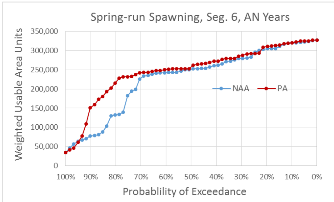
Figure 5.4-111. Exceedance Plot of Spring-Run Chinook Salmon Spawning Weighted Usable Area (WUA) for NAA and PA Model Scenarios in River Segment 6, Above Normal Water Years
