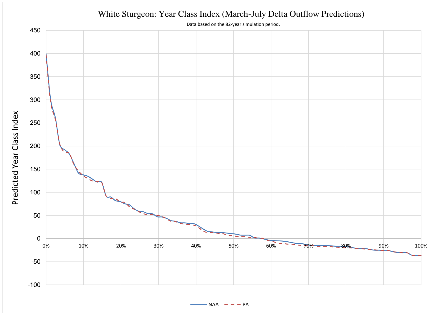
Figure 5.4-27. Exceedance Plot of White Sturgeon Year Class Index from the Mean March-July Delta Outflow Regression.
