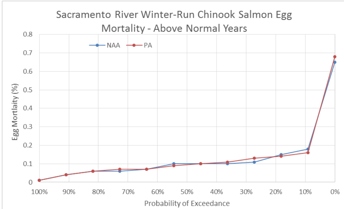
Figure 5.4-63. Exceedance Plot of Winter-Run Chinook Salmon Egg Mortality for NAA and PA Model Scenarios, Reclamation Egg Mortality Model, Above Normal Water Years
