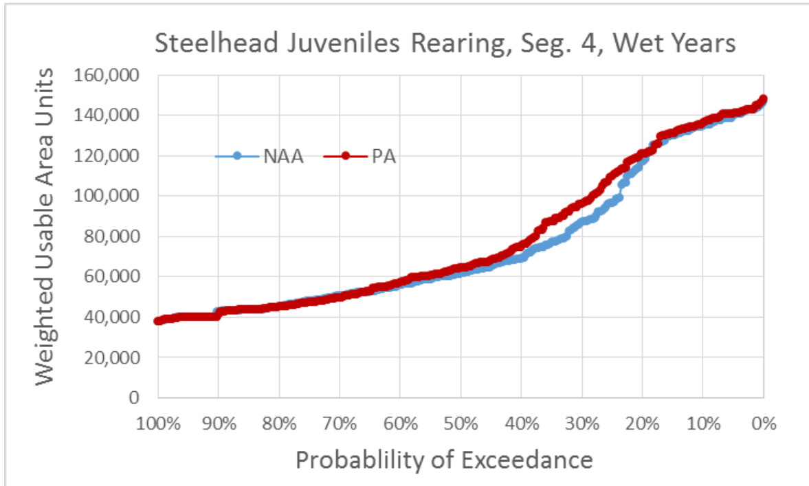
Figure 5.4-237. Exceedance Plot of CCV Steelhead Juvenile Rearing Weighted Usable Area (WUA) for NAA and PA Model Scenarios in River Segment 4, Wet Water Years
