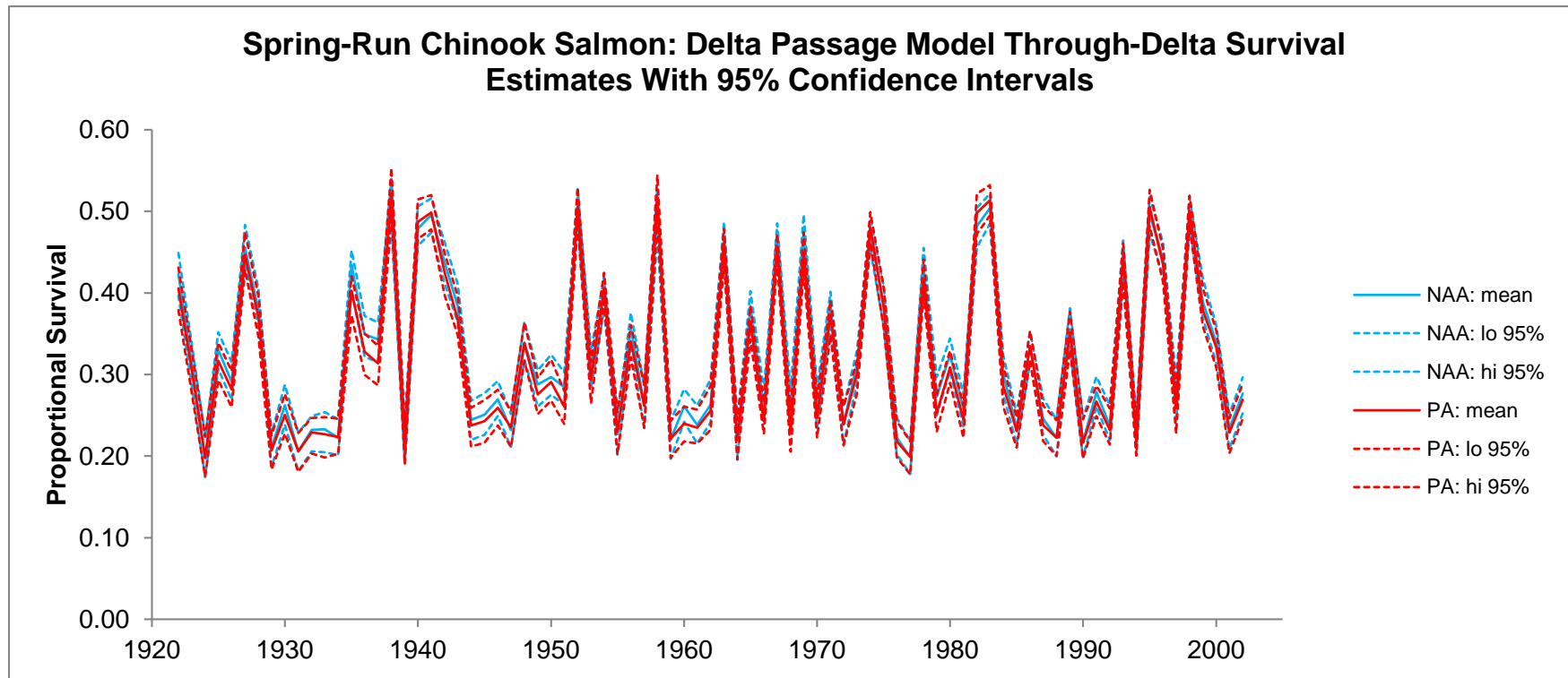
Figure 5.4-13. Time Series of Mean (With 95% Confidence Interval) Annual Juvenile Spring-Run Chinook Salmon Through-Delta Estimated from the Delta Passage Model.
