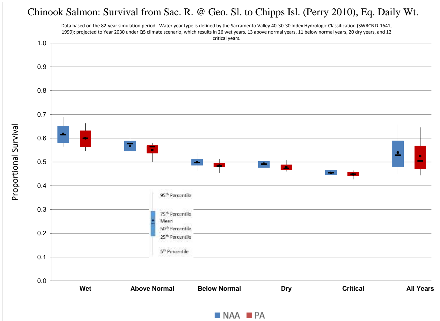
Figure 5.4-21. Box Plots of Juvenile Chinook Salmon Annual Total Survival from the Sacramento River at Georgiana Slough to Chipps Island, Estimated from the Analysis Based on Perry (2010), Grouped by Water Year Type, Assuming Equal Daily Weighting from December to June.
