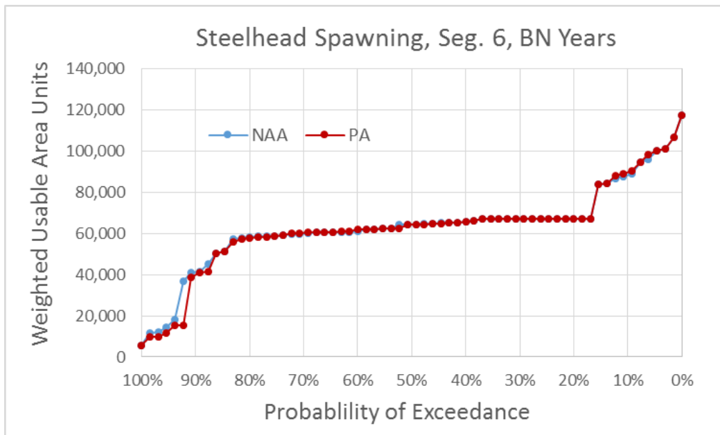
Figure 5.4-183. Exceedance Plot of Central Valley Steelhead Spawning Weighted Usable Area (WUA) for NAA and PA Model Scenarios in River Segment 6, Below Normal Water Years
