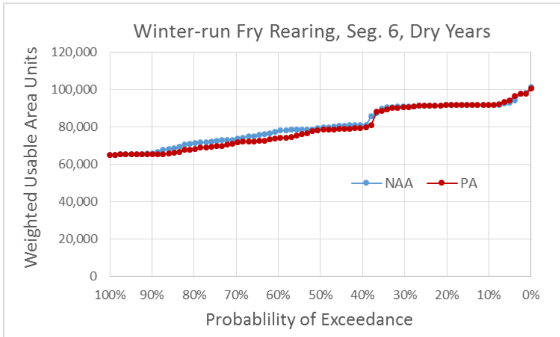
Figure 5.4-72. Exceedance Plot of Winter-Run Chinook Salmon Fry Rearing Weighted Usable Area (WUA) for NAA and PA Model Scenarios in River Segment 6, Dry Water Years
