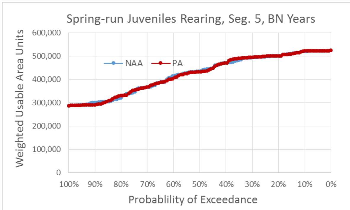
Figure 5.4-168. Exceedance Plot of Spring-Run Chinook Salmon Juvenile Rearing Weighted Usable Area (WUA) for NAA and PA Model Scenarios in River Segment 5, Below Normal Water Years
