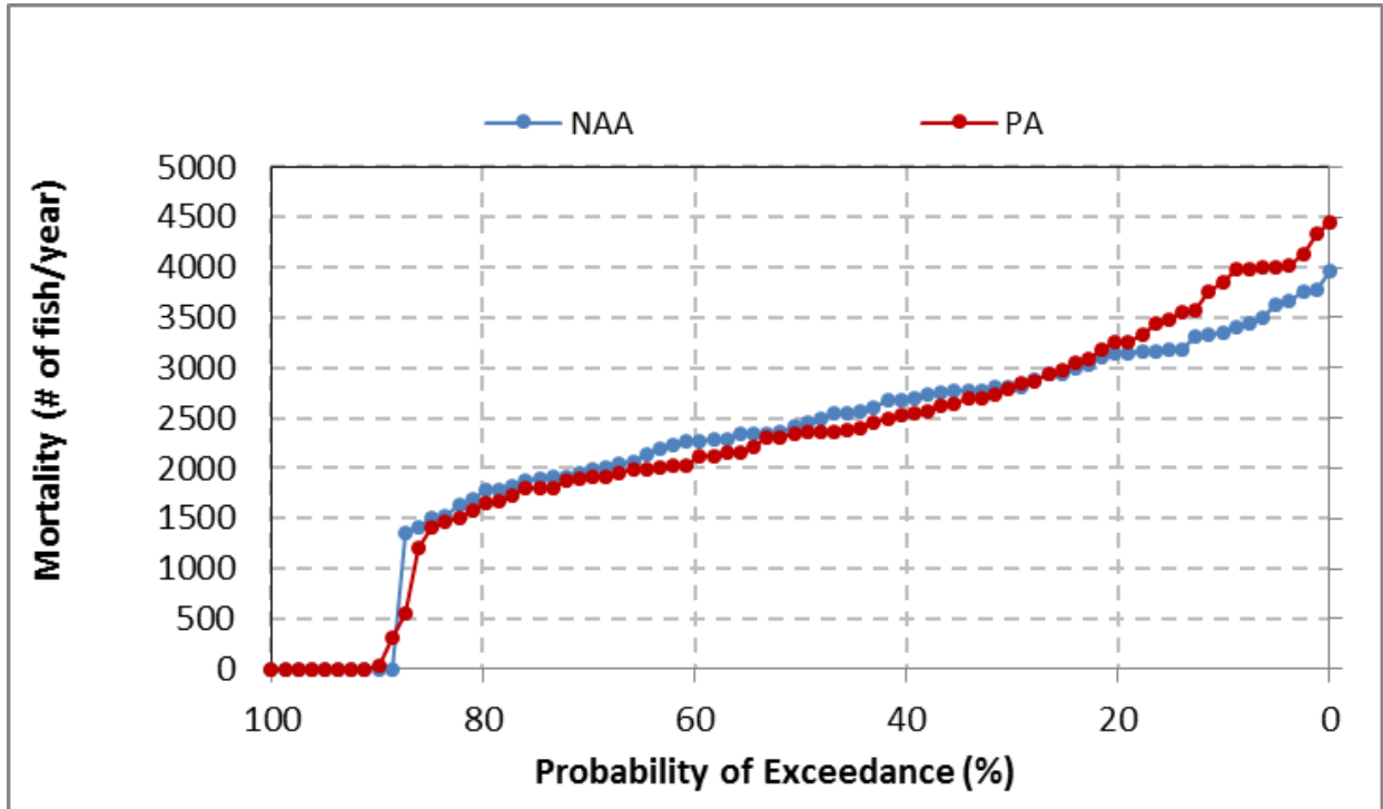
Figure 5.4-177. Exceedance Plot of Annual Flow-Based Mortality (# of Fish/Year) of Spring-Run Chinook Salmon Fry and Juveniles, SALMOD
