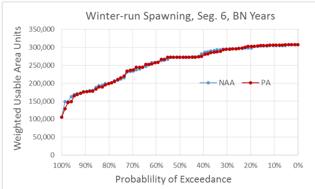
Figure 5.4-33. Exceedance Plot of Winter-Run Chinook Salmon Spawning Weighted Usable Area (WUA) for NAA and PA Model Scenarios in River Segment 6, Below Normal Water Years
