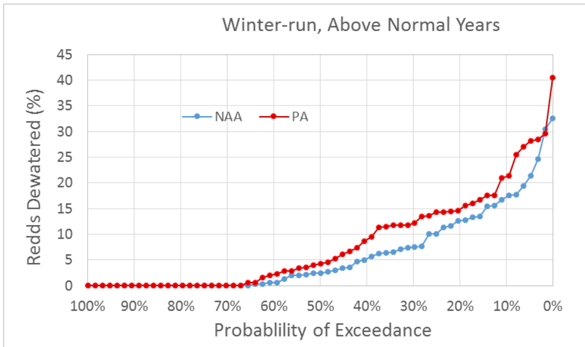
Figure 5.4-50. Exceedance Plot of Winter-Run Chinook Salmon Percent of Redds Dewatered for NAA and PA Model Scenarios, Above Normal Water Years
