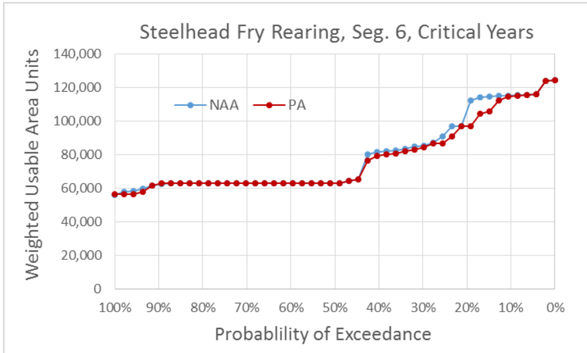
Figure 5.4-211. Exceedance Plot of CCV Steelhead Fry Rearing Weighted Usable Area (WUA) for NAA and PA Model Scenarios in River Segment 6, Critical Water Years
