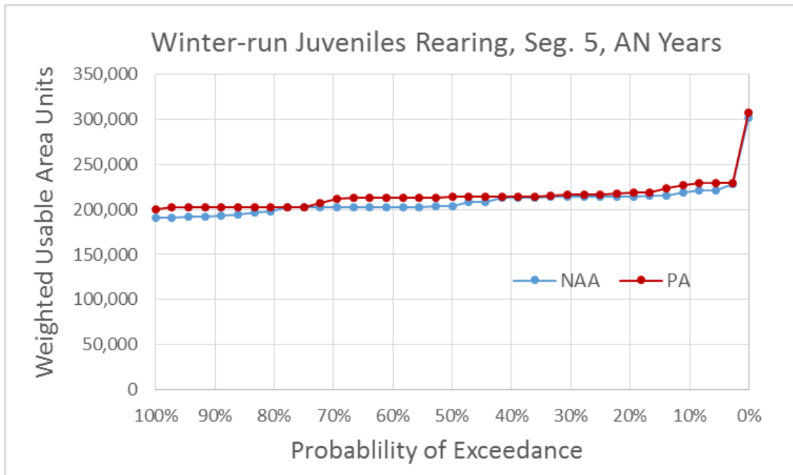
Figure 5.4-94. Exceedance Plot of Winter-Run Chinook Salmon Juvenile Rearing Weighted Usable Area (WUA) for NAA and PA Model Scenarios in River Segment 5, Above Normal Water Years
