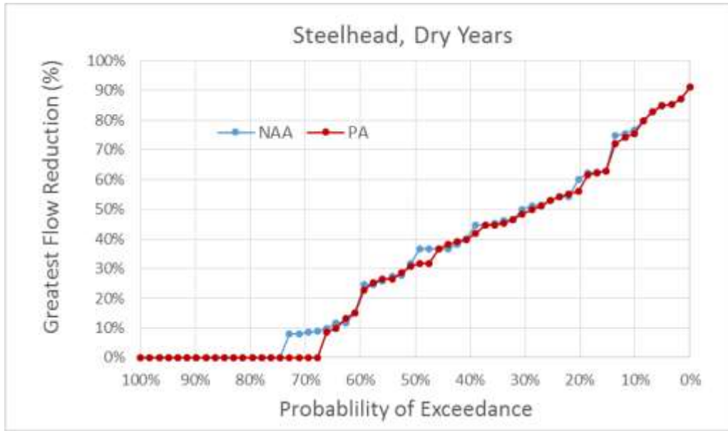
Figure 5.4-258. Exceedance Plot of Maximum Flow Reductions for 3-Month Period after Central Valley Steelhead Spawning for NAA and PA Model Scenarios, Dry Water Years
