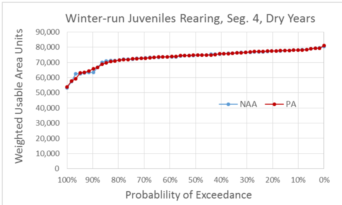
Figure 5.4-102. Exceedance Plot of Winter-Run Chinook Salmon Juvenile Rearing Weighted Usable Area (WUA) for NAA and PA Model Scenarios in River Segment 4, Dry Water Years
