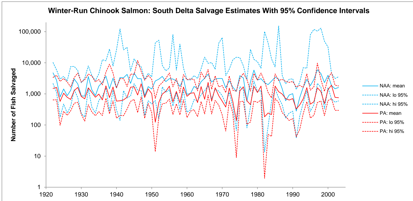
Figure 5.4-6. Annual Number of Winter-Run Chinook Salmon Salvaged (From 1,000,000 Released), With 95% Confidence Intervals, from the Analysis Based on Zeug and Cavallo (2014).
