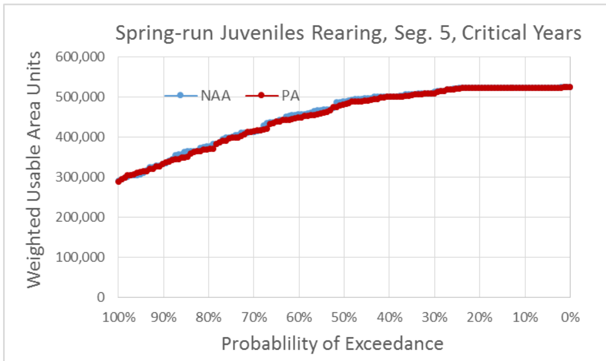
Figure 5.4-170. Exceedance Plot of Spring-Run Chinook Salmon Juvenile Rearing Weighted Usable Area (WUA) for NAA and PA Model Scenarios in River Segment 5, Critical Water Years
