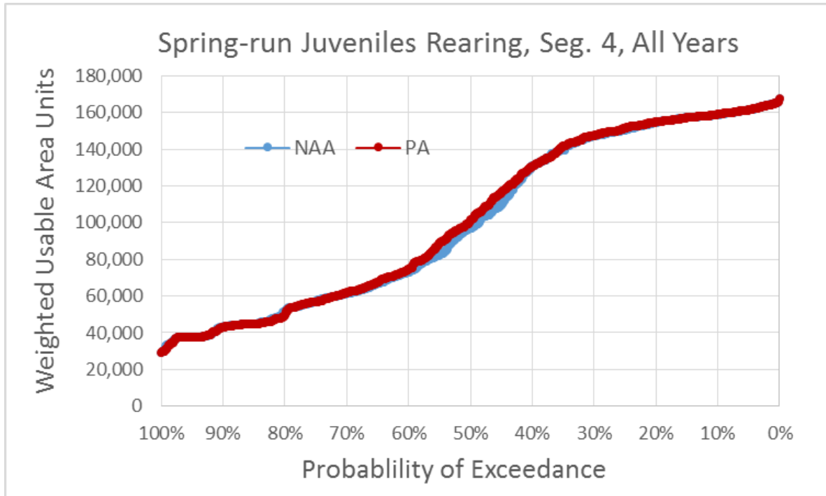
Figure 5.4-171. Exceedance Plot of Spring-Run Chinook Salmon Juvenile Rearing Weighted Usable Area (WUA) for NAA and PA Model Scenarios in River Segment 4, All Water Years
