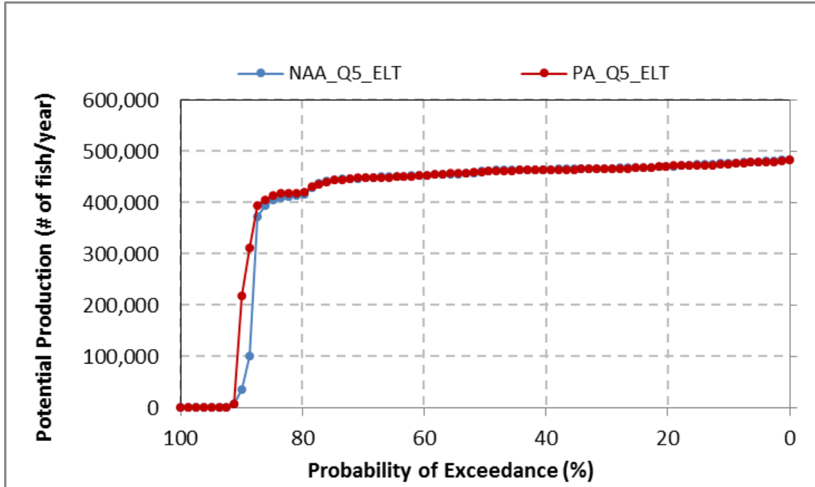
Figure 5.4-179. Exceedance Plot for Annual Potential Production (# of Fish/Year) of Spring-Run Chinook Salmon, SALMOD
