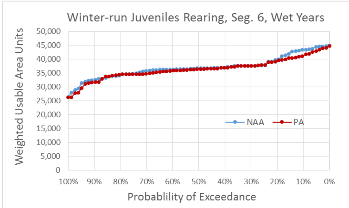
Figure 5.4-87. Exceedance Plot of Winter-Run Chinook Salmon Juvenile Rearing Weighted Usable Area (WUA) for NAA and PA Model Scenarios in River Segment 6, Wet Water Years
