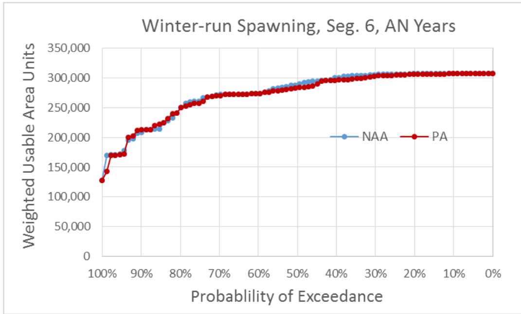
Figure 5.4-32. Exceedance Plot of Winter-Run Chinook Salmon Spawning Weighted Usable Area (WUA) for NAA and PA Model Scenarios in River Segment 6, Above Normal Water Years
