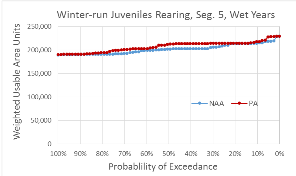
Figure 5.4-93. Exceedance Plot of Winter-Run Chinook Salmon Juvenile Rearing Weighted Usable Area (WUA) for NAA and PA Model Scenarios in River Segment 5, Wet Water Years
