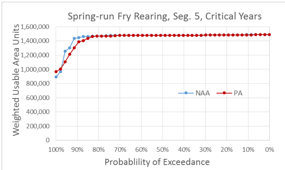
Figure 5.4-152. Exceedance Plot of Spring-Run Chinook Salmon Fry Rearing Weighted Usable Area (WUA) for NAA and PA Model Scenarios in River Segment 5, Critical Water Years
