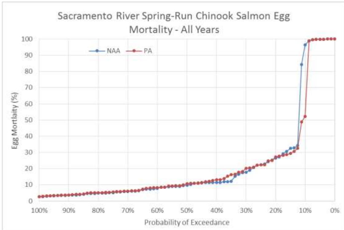
Figure 5.4-134. Exceedance Plot of Spring-Run Chinook Salmon Egg Mortality for NAA and PA Model Scenarios, Reclamation Egg Mortality Model, All Water Years
