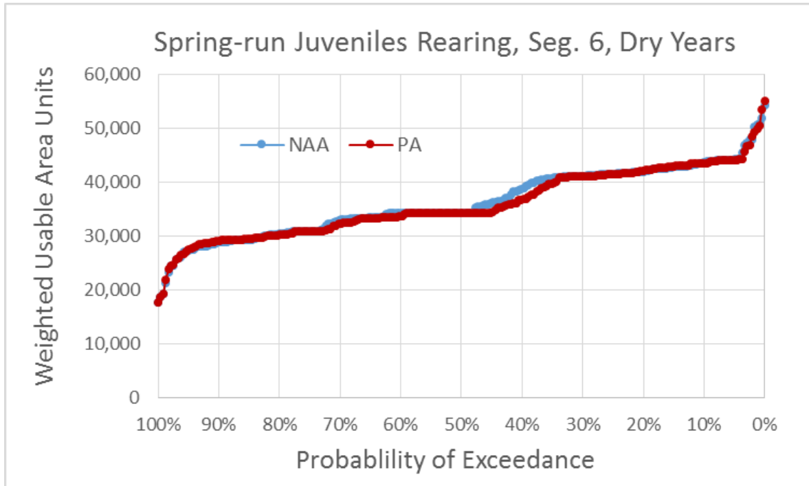
Figure 5.4-163. Exceedance Plot of Spring-Run Chinook Salmon Juvenile Rearing Weighted Usable Area (WUA) for NAA and PA Model Scenarios in River Segment 6, Dry Water Years
