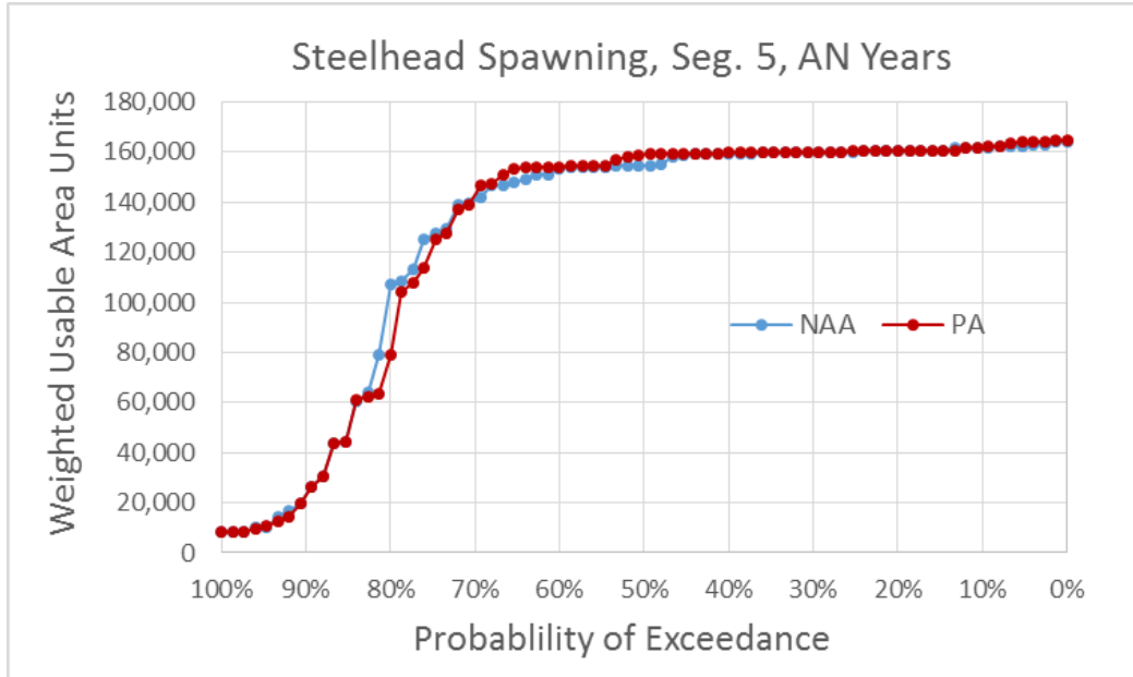
Figure 5.4-188. Exceedance Plot of Central Valley Steelhead Spawning Weighted Usable Area (WUA) for NAA and PA Model Scenarios in River Segment 5, Above Normal Water Years
