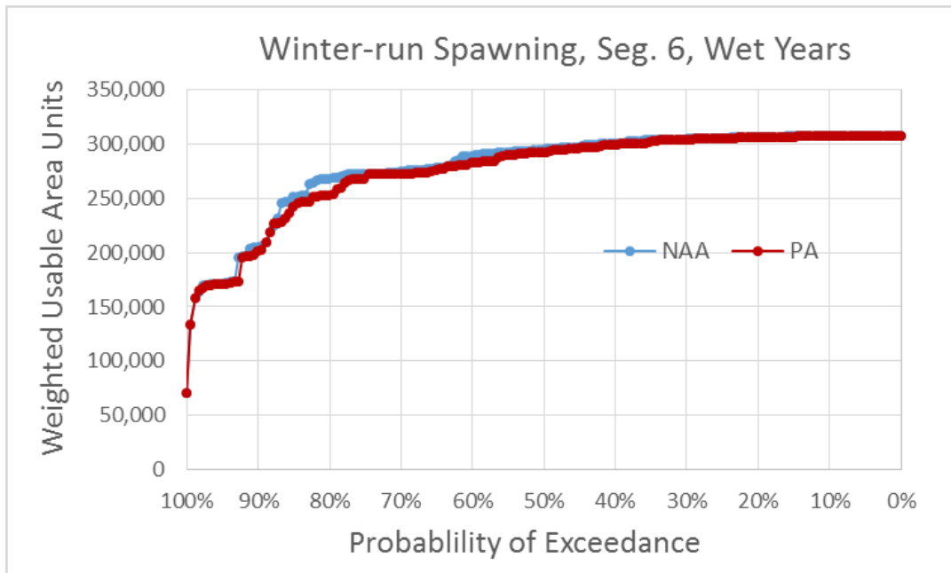
Figure 5.4-31. Exceedance Plot of Winter-Run Chinook Salmon Spawning Weighted Usable Area (WUA) for NAA and PA Model Scenarios in River Segment 6, Wet Water Years
