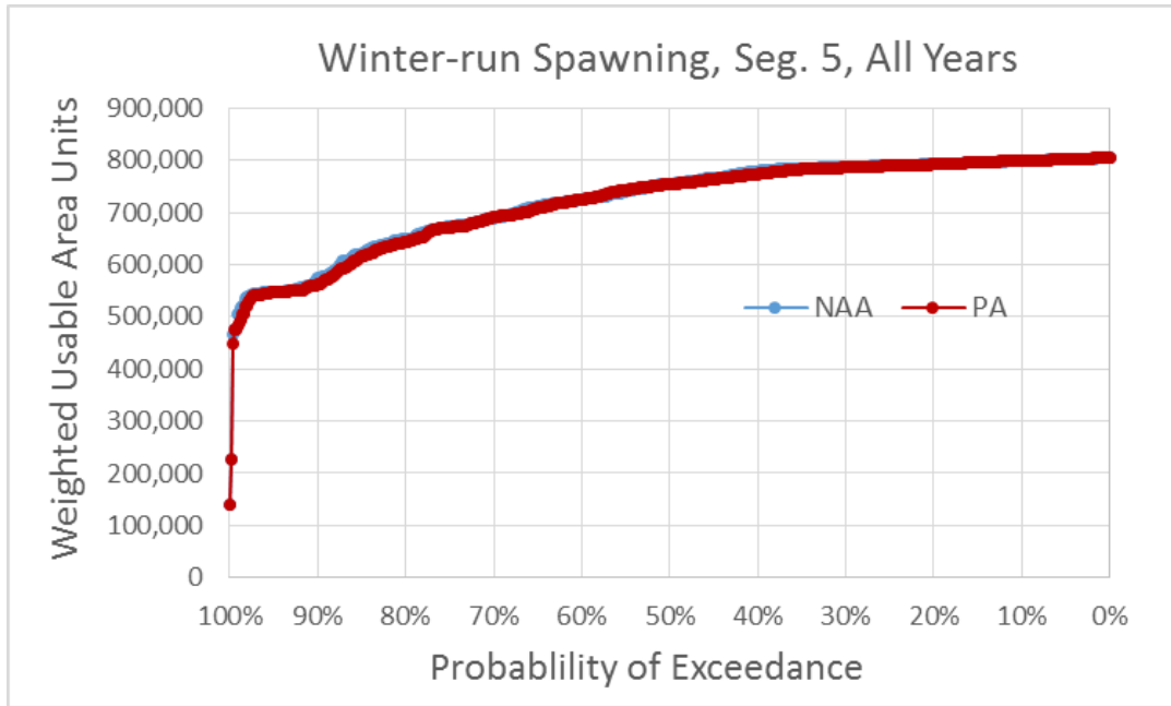
Figure 5.4-36. Exceedance Plot of Winter-Run Chinook Salmon Spawning Weighted Usable Area (WUA) for NAA and PA Model Scenarios in River Segment 5, All Water Years
