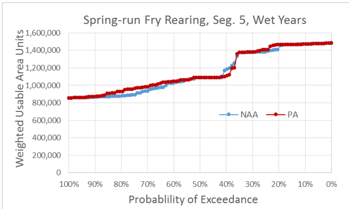
Figure 5.4-148. Exceedance Plot of Spring-Run Chinook Salmon Fry Rearing Weighted Usable Area (WUA) for NAA and PA Model Scenarios in River Segment 5, Wet Water Years
