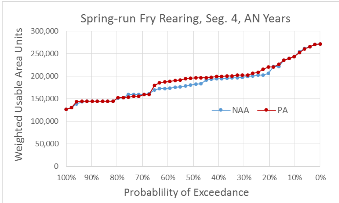
Figure 5.4-155. Exceedance Plot of Spring-Run Chinook Salmon Fry Rearing Weighted Usable Area (WUA) for NAA and PA Model Scenarios in River Segment 4, Above Normal Water Years
