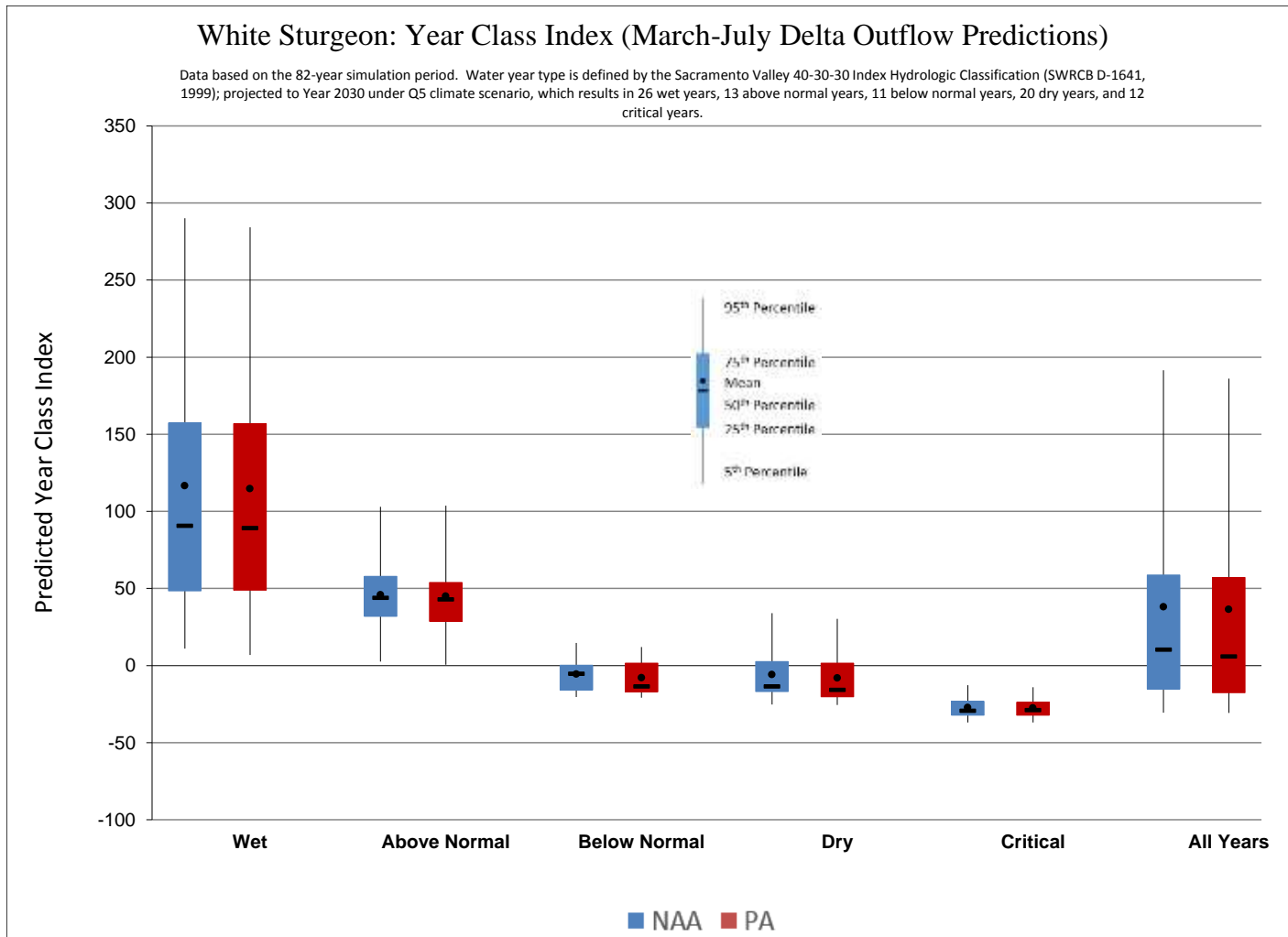
Figure 5.4-26. Box Plots of White Sturgeon Year Class Index from the Mean March-July Delta Outflow Regression, Grouped by Water Year Type.
