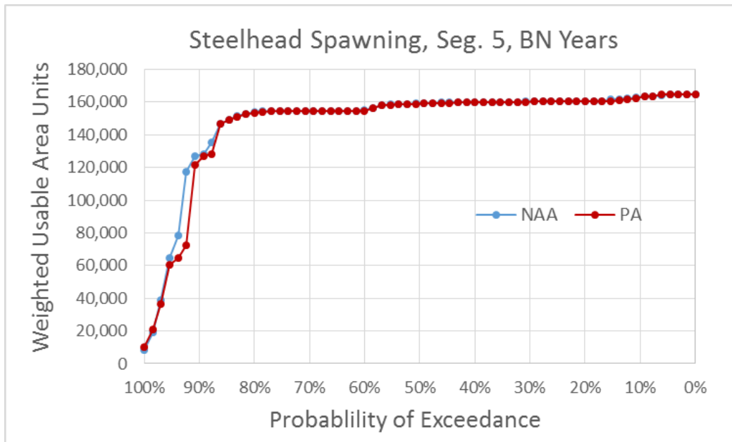
Figure 5.4-189. Exceedance Plot of Central Valley Steelhead Spawning Weighted Usable Area (WUA) for NAA and PA Model Scenarios in River Segment 5, Below Normal Water Years
