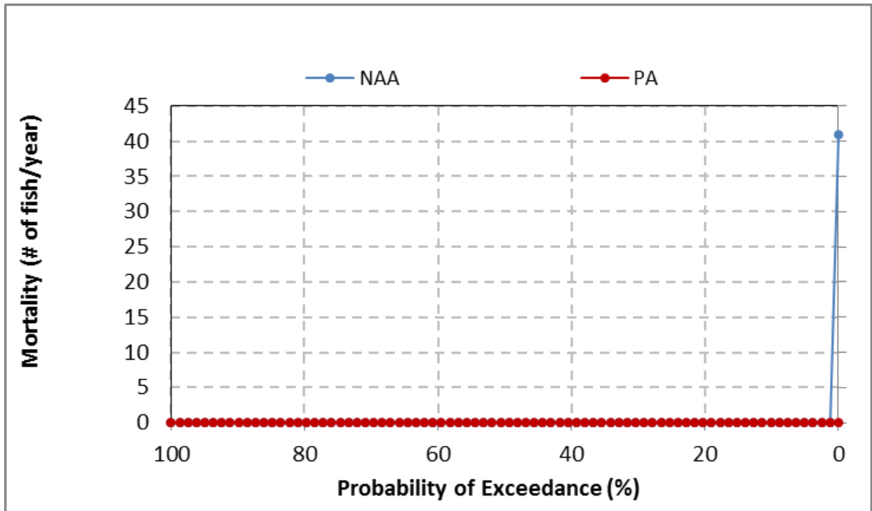
Figure 5.4-178. Exceedance Plot of Annual Water Temperature-Based Mortality (# of Fish/Year) of Spring-Run Chinook Salmon Fry and Juveniles, SALMOD
