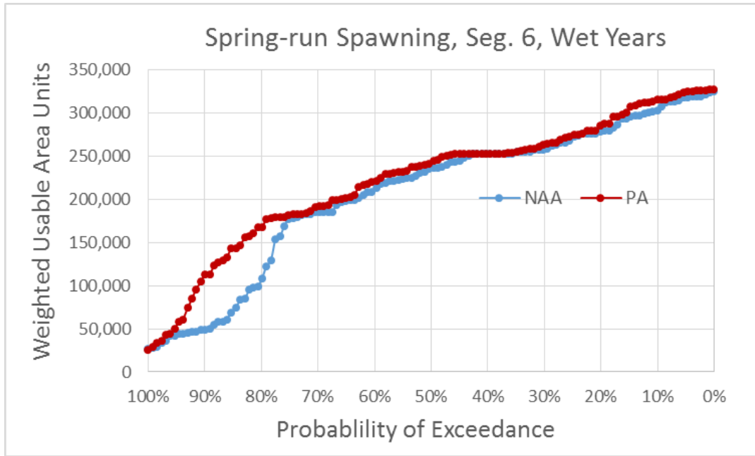
Figure 5.4-110. Exceedance Plot of Spring-Run Chinook Salmon Spawning Weighted Usable Area (WUA) for NAA and PA Model Scenarios in River Segment 6, Wet Water Years
