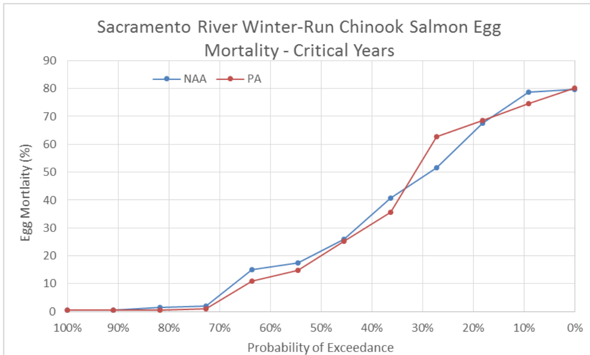
Figure 5.4-66. Exceedance Plot of Winter-Run Chinook Salmon Egg Mortality for NAA and PA Model Scenarios, Reclamation Egg Mortality Model, Critical Water Years
