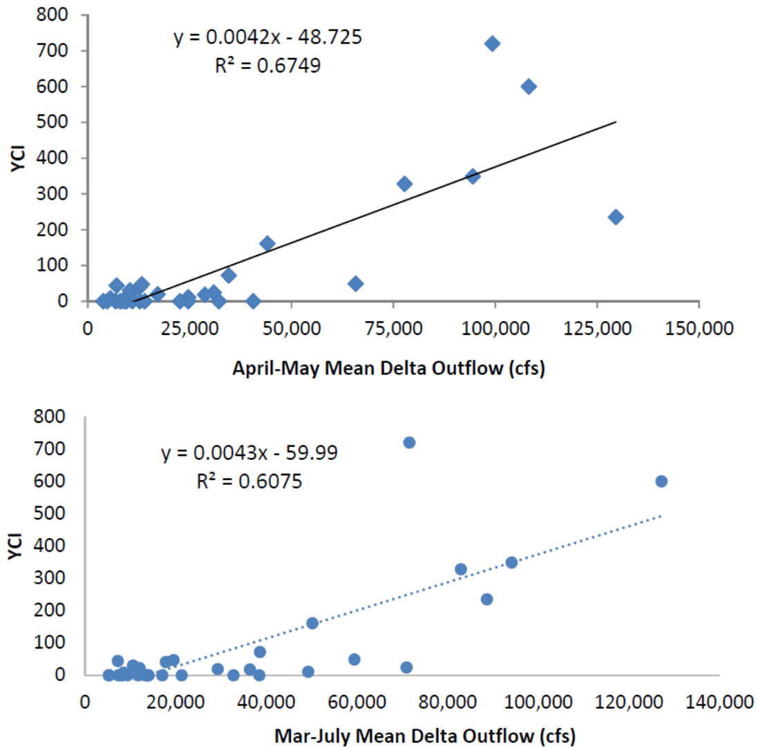
Figure 5.4-23. White Sturgeon Year-Class Index (YCI) for 1980-2011 as function of Mean April-May Delta Outflow (Upper Panel) and Mean March-July Delta Outflow (Lower Panel).
