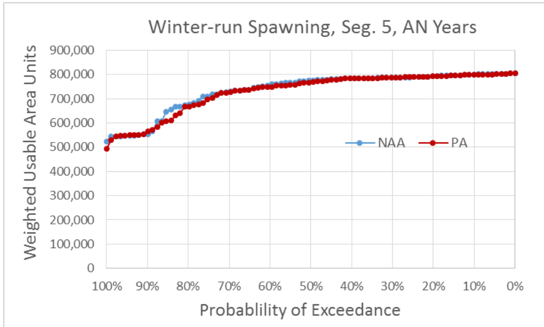
Figure 5.4-38. Exceedance Plot of Winter-Run Chinook Salmon Spawning Weighted Usable Area (WUA) for NAA and PA Model Scenarios in River Segment 5, Above Normal Water Years
