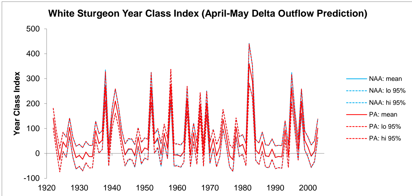
Figure 5.4-28. Time Series of Mean (With 95% Confidence Interval) Annual White Sturgeon Year Class Index, Estimated from the Mean April-May Delta Outflow Regression.
