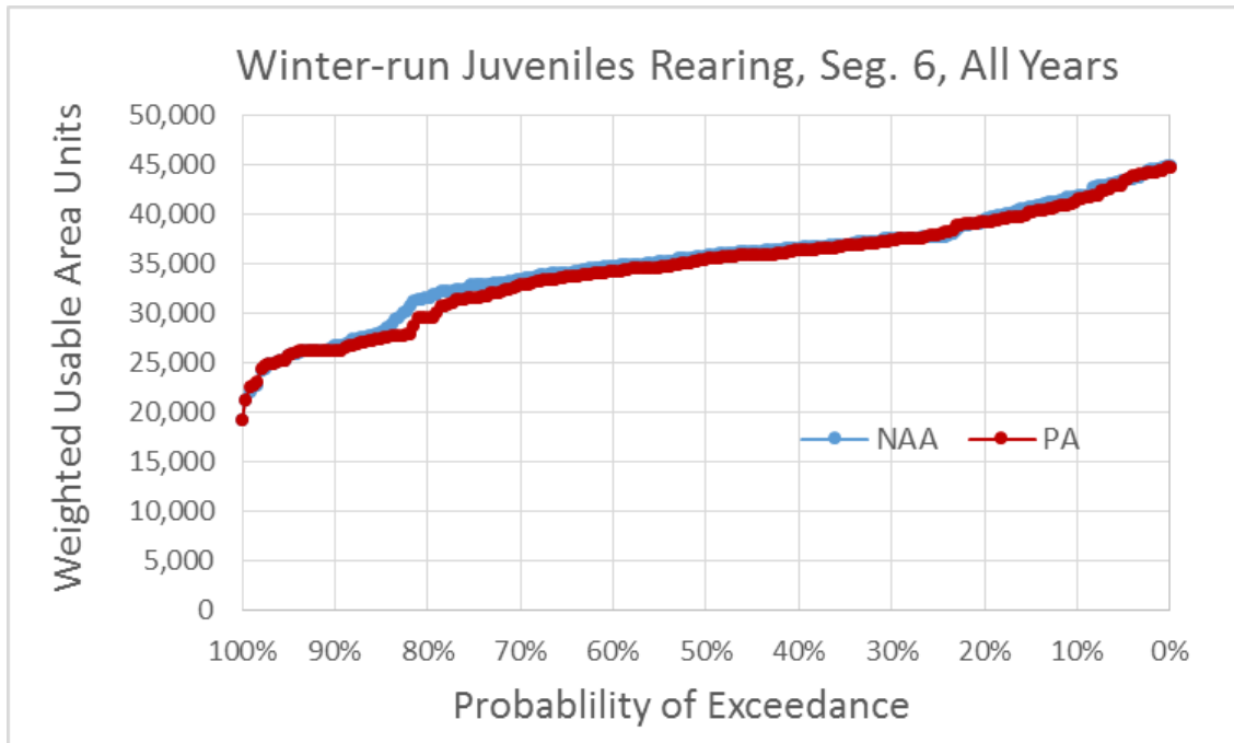
Figure 5.4-86. Exceedance Plot of Winter-Run Chinook Salmon Juvenile Rearing Weighted Usable Area (WUA) for NAA and PA Model Scenarios in River Segment 6, All Water Years
