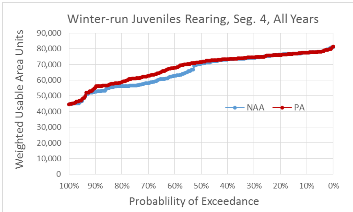
Figure 5.4-98. Exceedance Plot of Winter-Run Chinook Salmon Juvenile Rearing Weighted Usable Area (WUA) for NAA and PA Model Scenarios in River Segment 4, All Water Years
