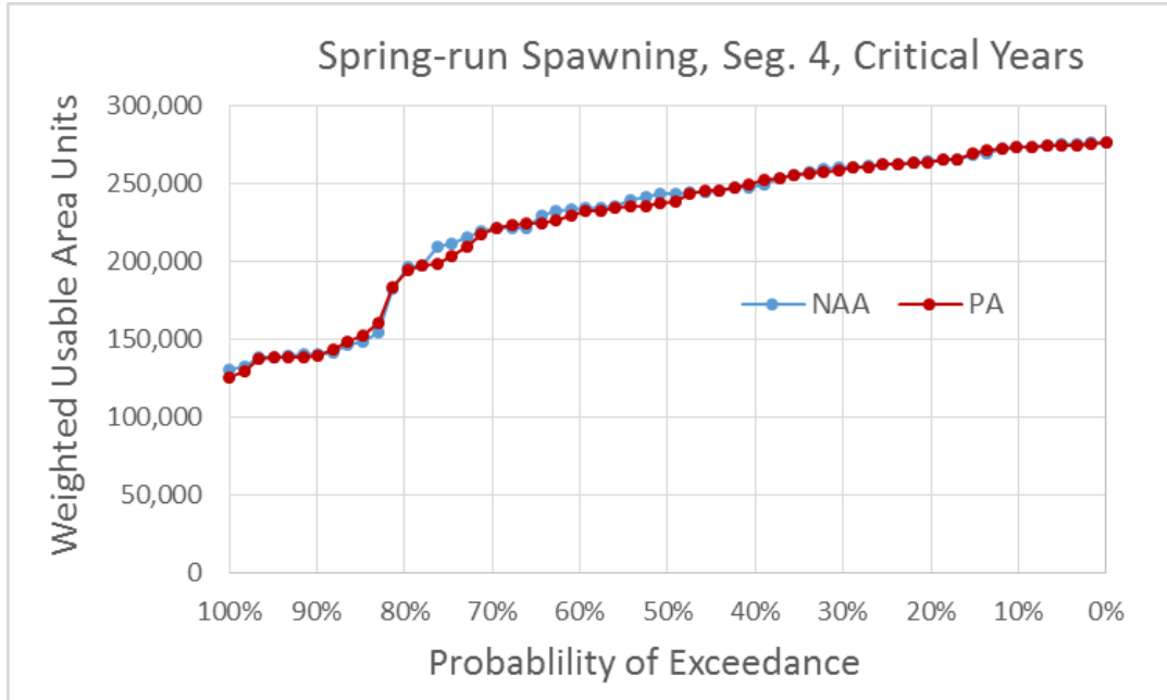
Figure 5.4-126. Exceedance Plot of Spring-Run Chinook Salmon Spawning Weighted Usable Area (WUA) for NAA and PA Model Scenarios in River Segment 4, Critical Water Years
