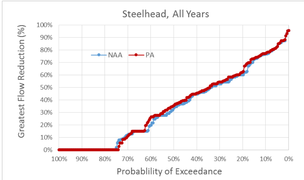
Figure 5.4-254. Exceedance Plot of Maximum Flow Reductions (%) for 3-Month Period after Central Valley Steelhead Spawning for NAA and PA Model Scenarios, All Water Years
