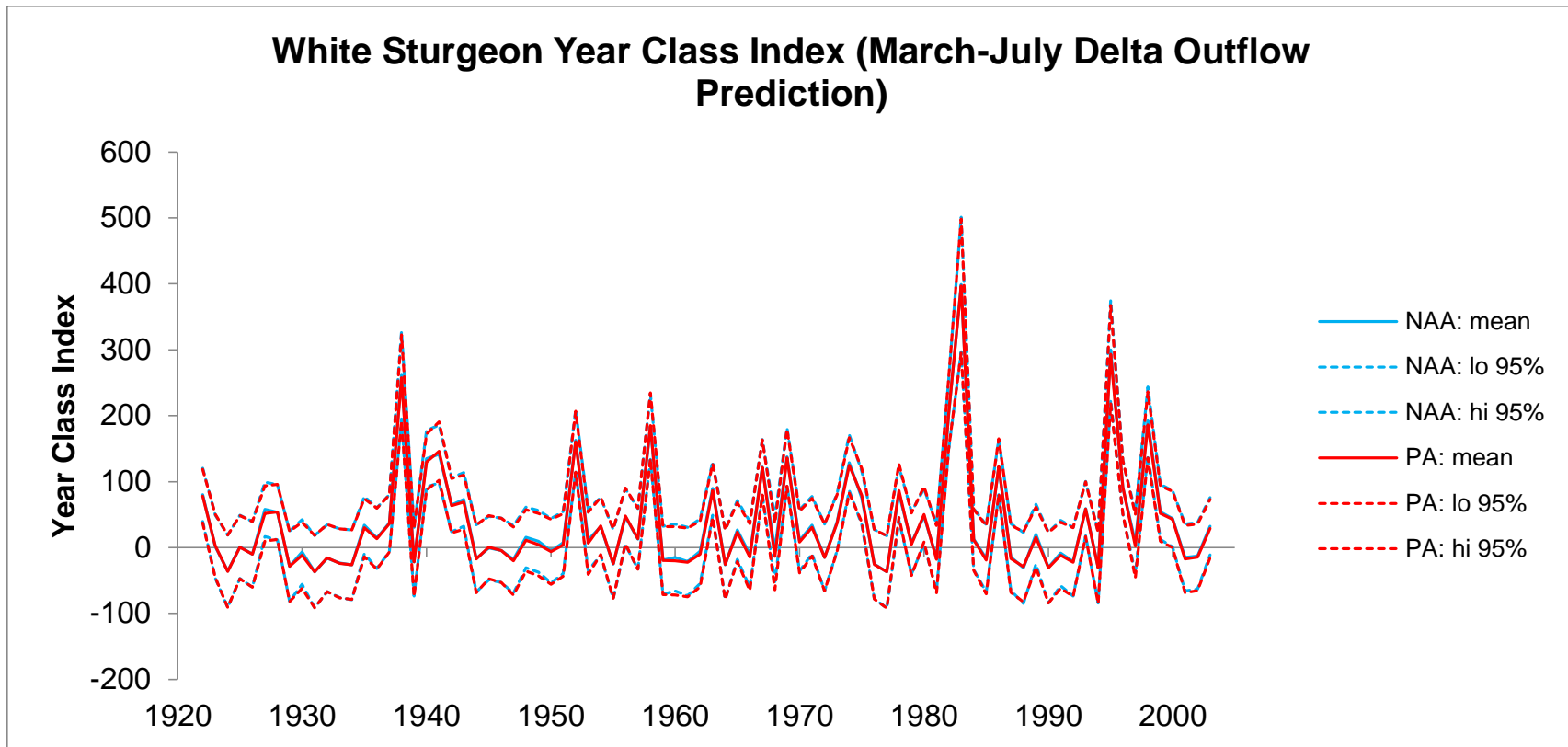
Figure 5.4-29. Time Series of Mean (With 95% Confidence Interval) Annual White Sturgeon Year Class Index, Estimated from the Mean March-July Delta Outflow Regression.
