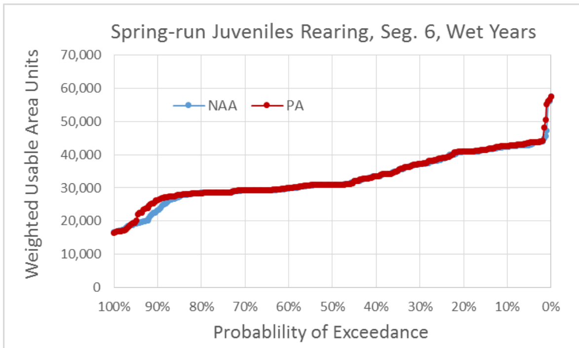
Figure 5.4-160. Exceedance Plot of Spring-Run Chinook Salmon Juvenile Rearing Weighted Usable Area (WUA) for NAA and PA Model Scenarios in River Segment 6, Wet Water Years
