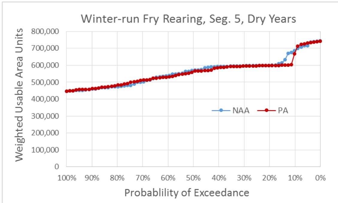
Figure 5.4-78. Exceedance Plot of Winter-Run Chinook Salmon Fry Rearing Weighted Usable Area (WUA) for NAA and PA Model Scenarios in River Segment 5, Dry Water Years
