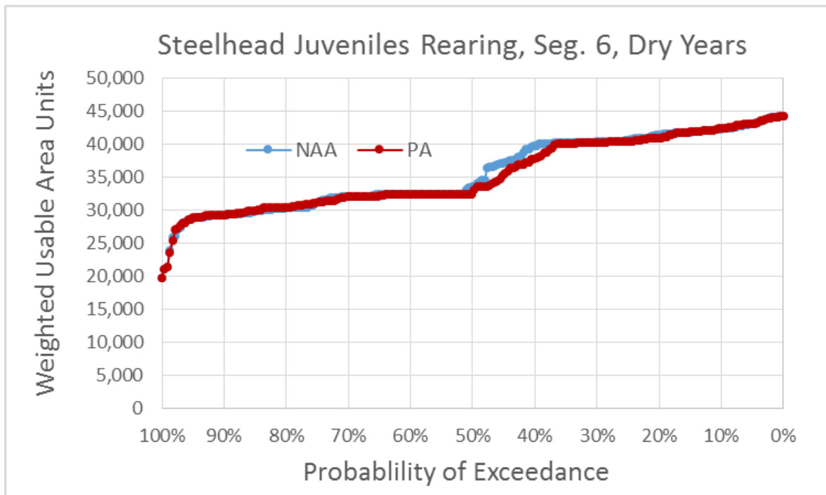
Figure 5.4-228. Exceedance Plot of CCV Steelhead Juvenile Rearing Weighted Usable Area (WUA) for NAA and PA Model Scenarios in River Segment 6, Dry Water Years
