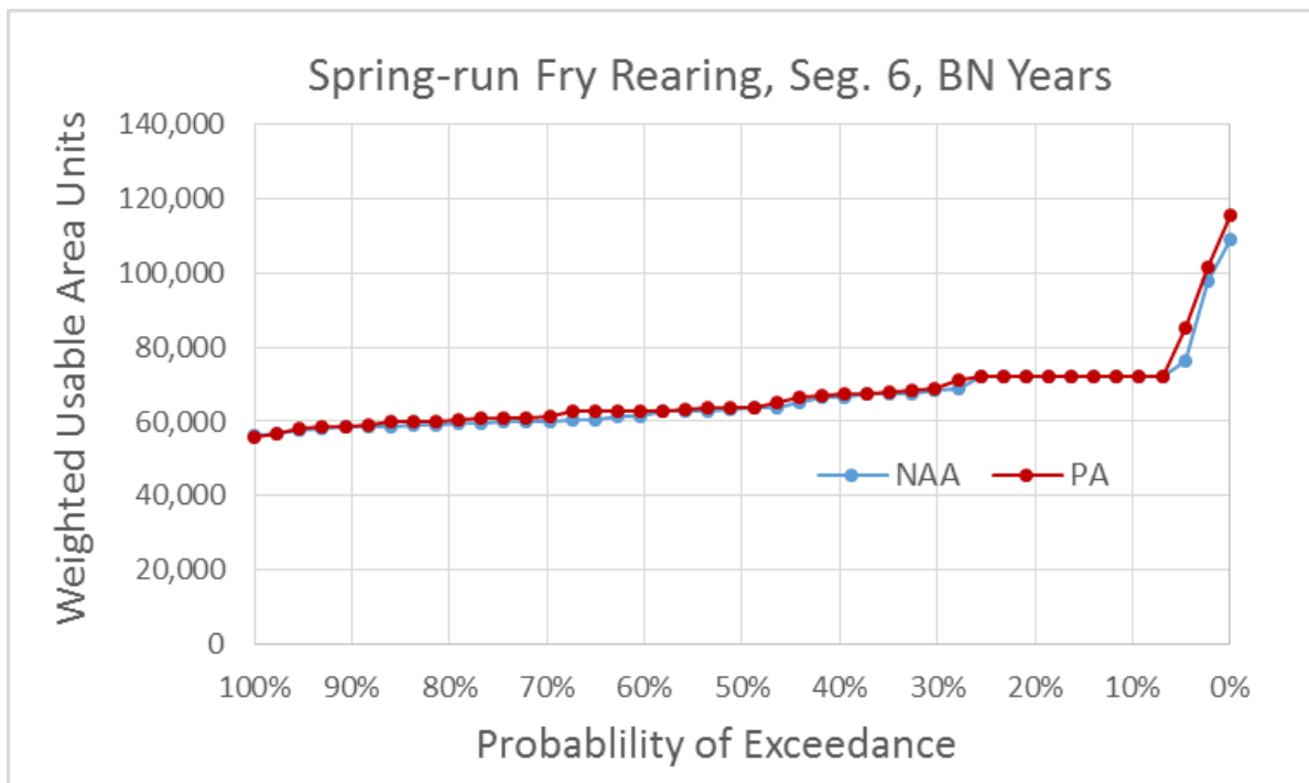
Figure 5.4-144. Exceedance Plot of Spring-Run Chinook Salmon Fry Rearing Weighted Usable Area (WUA) for NAA and PA Model Scenarios in River Segment 6, Below Normal Water Years
