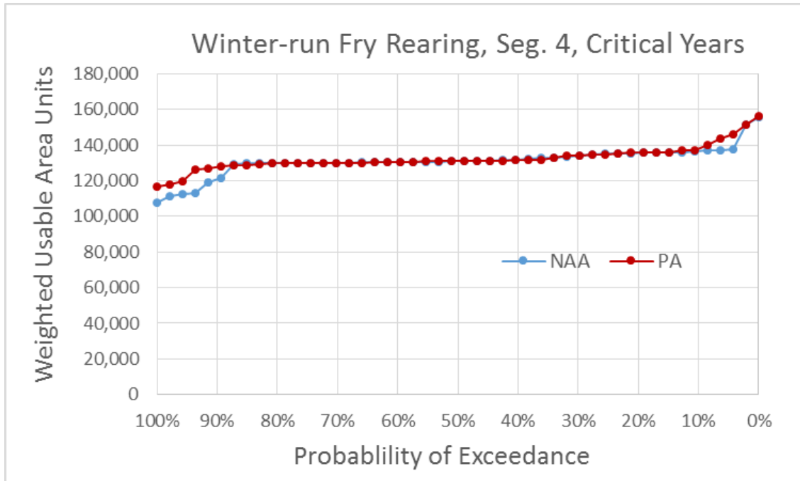
Figure 5.4-85. Exceedance Plot of Winter-Run Chinook Salmon Fry Rearing Weighted Usable Area (WUA) for NAA and PA Model Scenarios in River Segment 4, Critical Water Years
