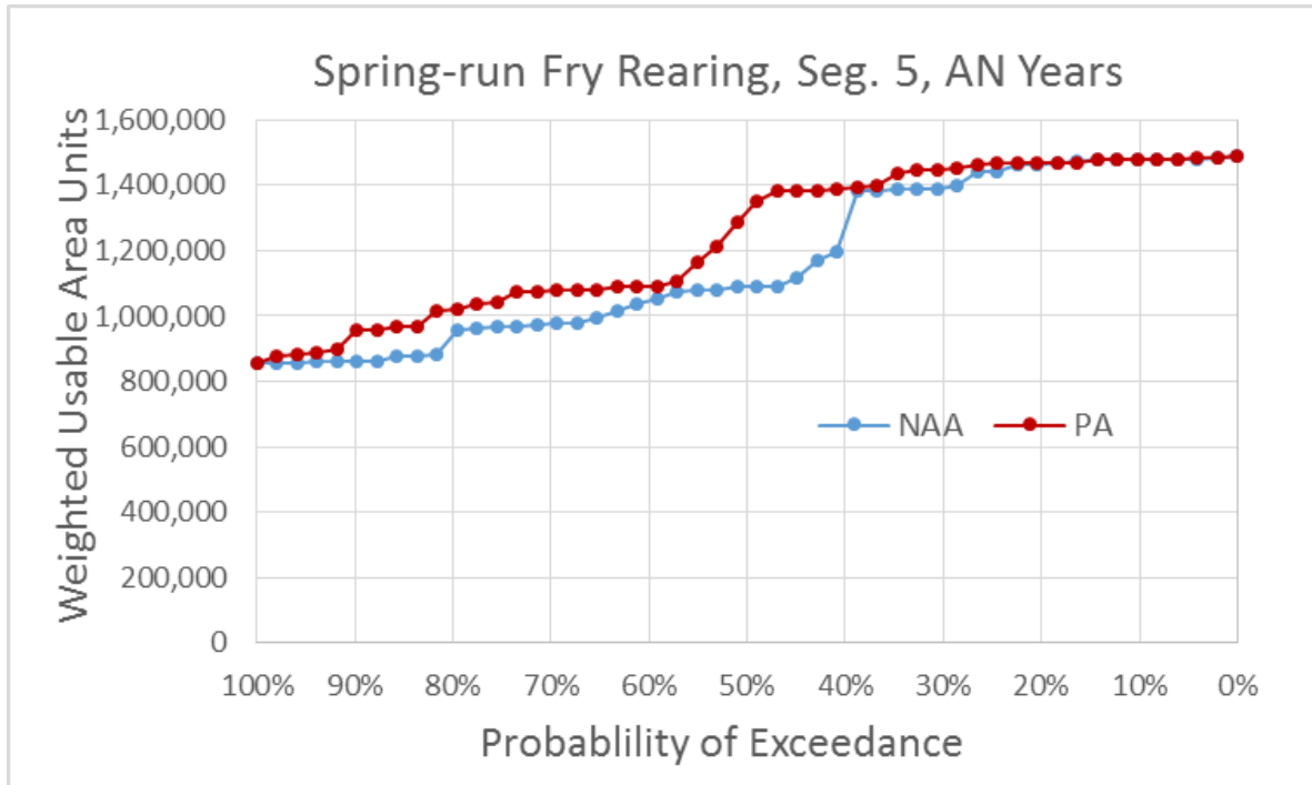
Figure 5.4-149. Exceedance Plot of Spring-Run Chinook Salmon Fry Rearing Weighted Usable Area (WUA) for NAA and PA Model Scenarios in River Segment 5, Above Normal Water Years
