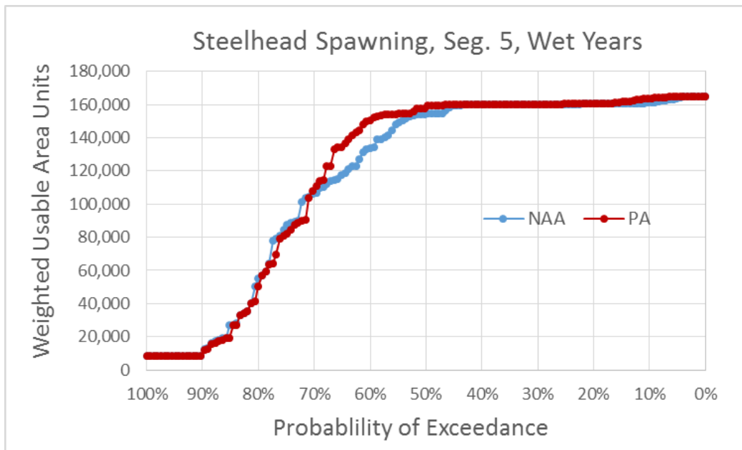
Figure 5.4-187. Exceedance Plot of Central Valley Steelhead Spawning Weighted Usable Area (WUA) for NAA and PA Model Scenarios in River Segment 5, Wet Water Years
