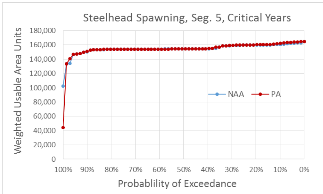
Figure 5.4-191. Exceedance Plot of Central Valley Steelhead Spawning Weighted Usable Area (WUA) for NAA and PA Model Scenarios in River Segment 5, Critical Water Years
