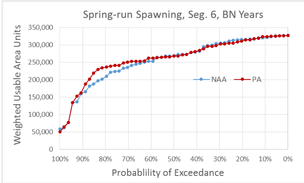
Figure 5.4-112. Exceedance Plot of Spring-Run Chinook Salmon Spawning Weighted Usable Area (WUA) for NAA and PA Model Scenarios in River Segment 6, Below Normal Water Years
