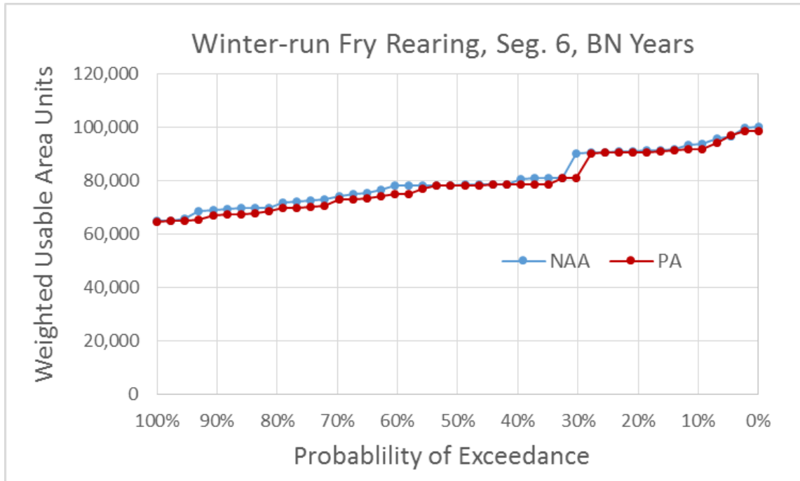
Figure 5.4-71. Exceedance Plot of Winter-Run Chinook Salmon Fry Rearing Weighted Usable Area (WUA) for NAA and PA Model Scenarios in River Segment 6, Below Normal Water Years
