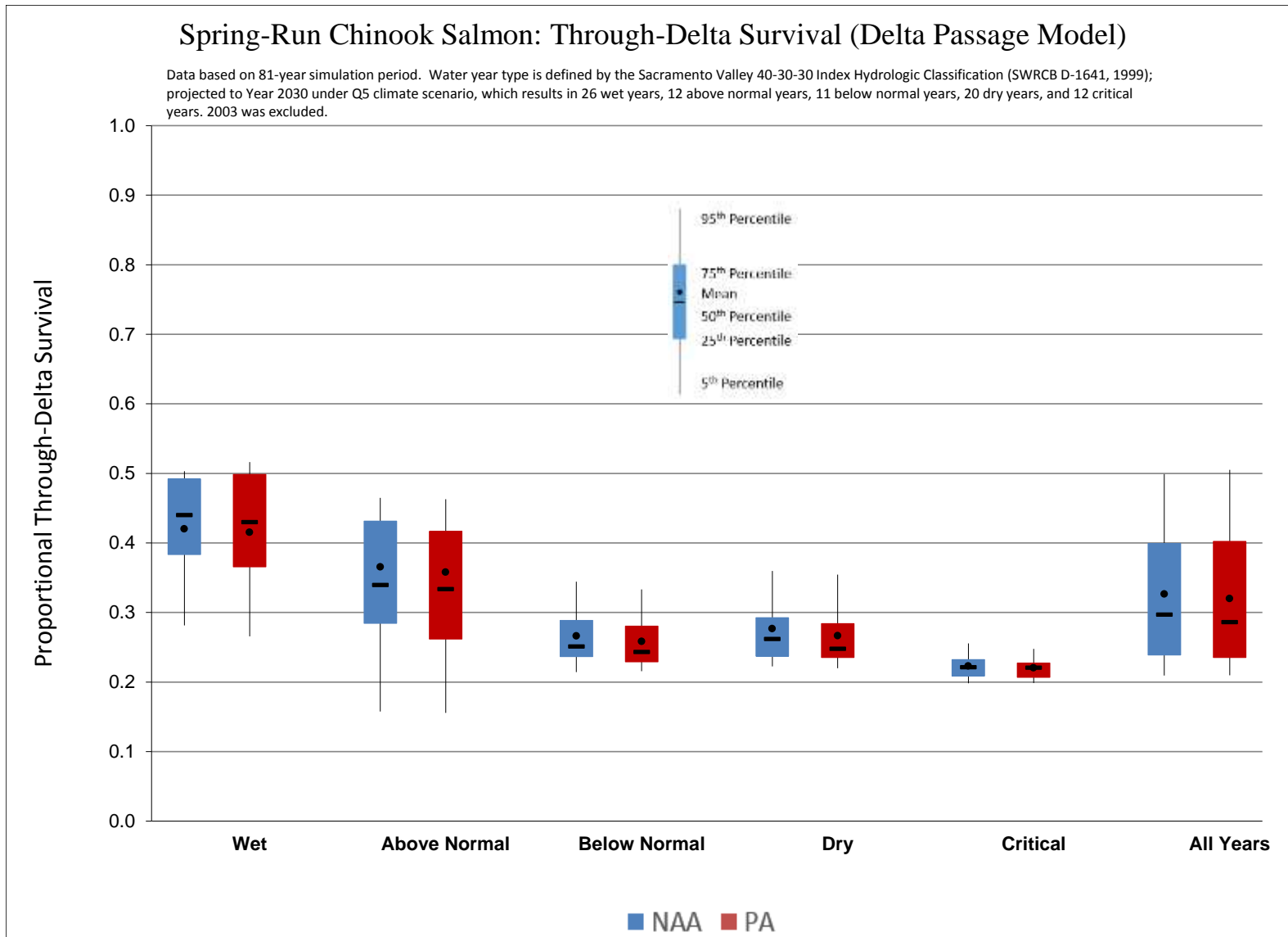
Figure 5.4-11. Box Plots of Spring-Run Chinook Salmon Annual Through-Delta Survival Estimated from the Delta Passage Model, Grouped by Water Year Type.
