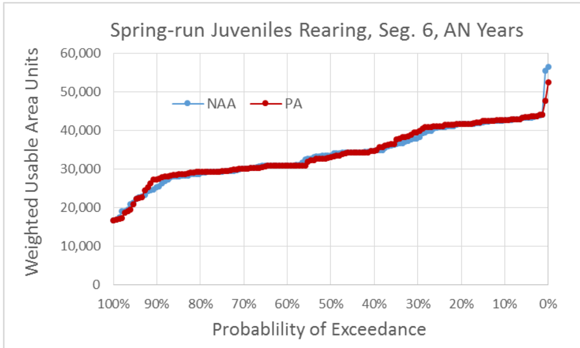
Figure 5.4-161. Exceedance Plot of Spring-Run Chinook Salmon Juvenile Rearing Weighted Usable Area (WUA) for NAA and PA Model Scenarios in River Segment 6, Above Normal Water Years
