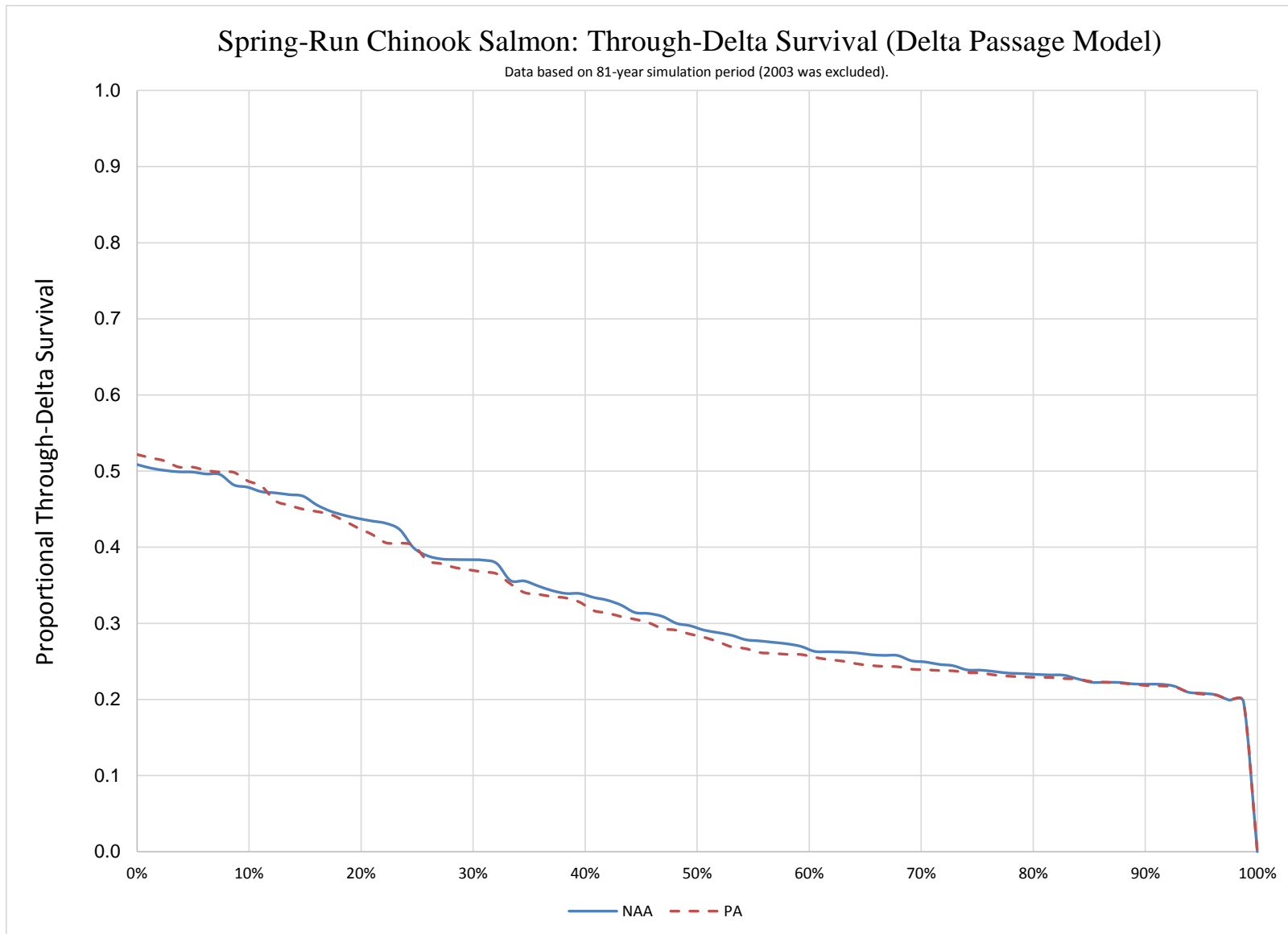
Figure 5.4-12. Exceedance Plot of Spring-Run Chinook Salmon Annual Through-Delta Survival Estimated from the Delta Passage Model.
