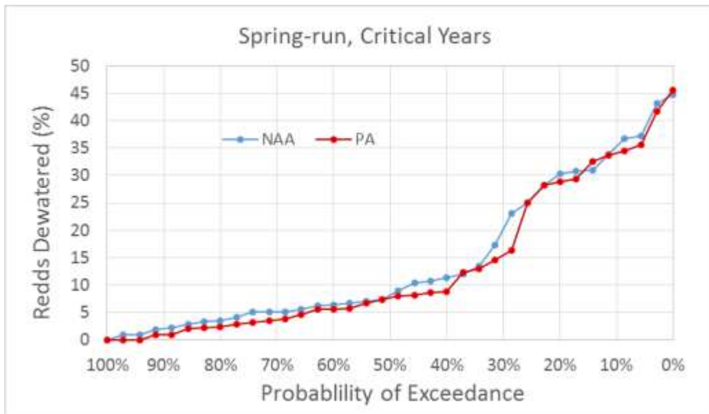
Figure 5.4-132. Exceedance Plot of Spring-Run Chinook Salmon Percent of Redds Dewatered for NAA and PA Model Scenarios, Critical Water Years
