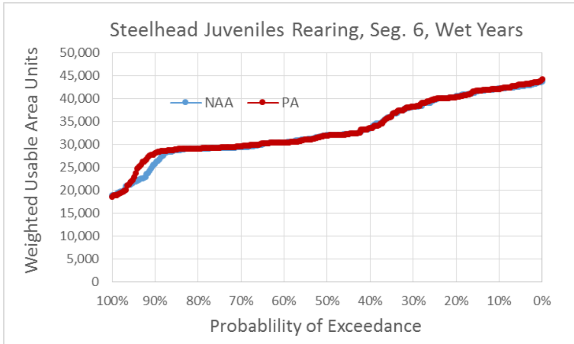
Figure 5.4-225. Exceedance Plot of CCV Steelhead Juvenile Rearing Weighted Usable Area (WUA) for NAA and PA Model Scenarios in River Segment 6, Wet Water Years
