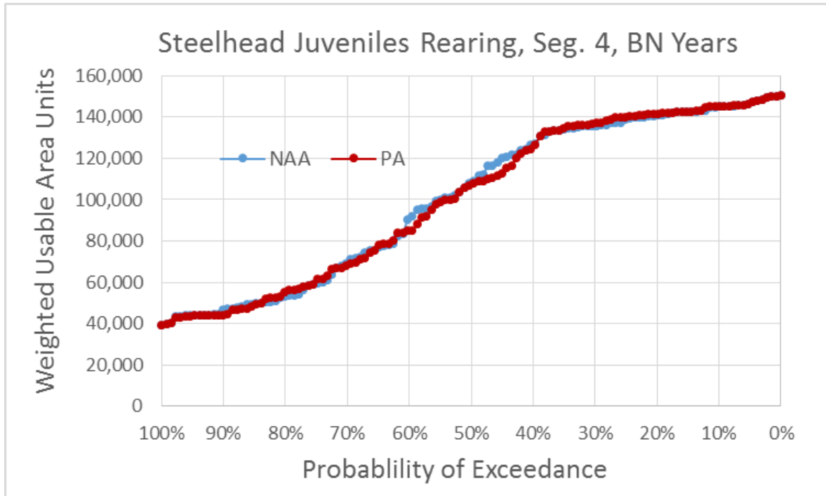
Figure 5.4-239. Exceedance Plot of CCV Steelhead Juvenile Rearing Weighted Usable Area (WUA) for NAA and PA Model Scenarios in River Segment 4, Below Normal Water Years
