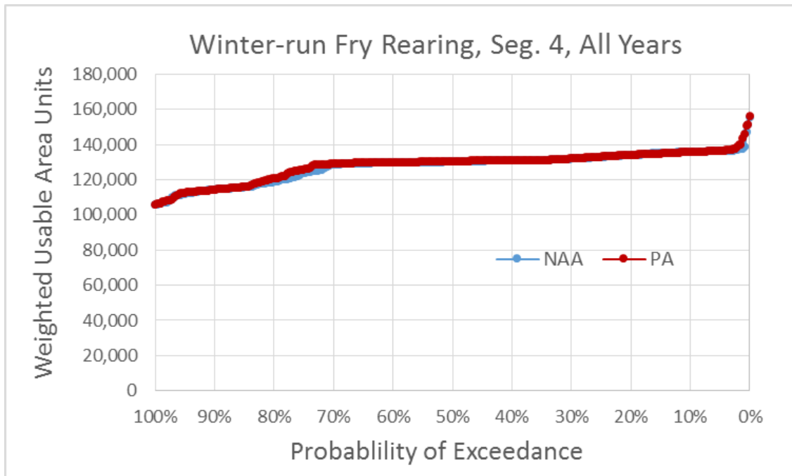
Figure 5.4-80. Exceedance Plot of Winter-Run Chinook Salmon Fry Rearing Weighted Usable Area (WUA) for NAA and PA Model Scenarios in River Segment 4, All Water Years
