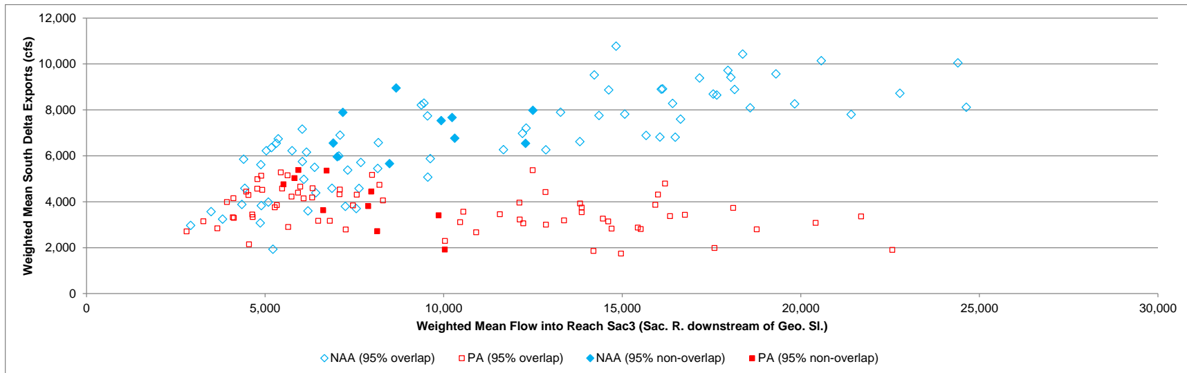
Figure 5.4-10. Delta Passage Model: Annual mean Sacramento River Flow into Reach Sac3 (Downstream of Georgiana Slough) and South Delta Exports, Weighted by Proportional Entry into the Delta of Winter-Run Chinook Salmon, Classified into Years of Overlapping and Non-overlapping Through-Delta Survival 95% Confidence Intervals.
