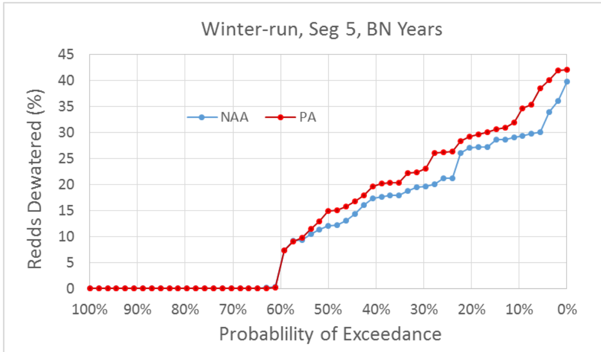
Figure 5.4-51. Exceedance Plot of Winter-Run Chinook Salmon Percent of Redds Dewatered for NAA and PA Model Scenarios, Below Normal Water Years
