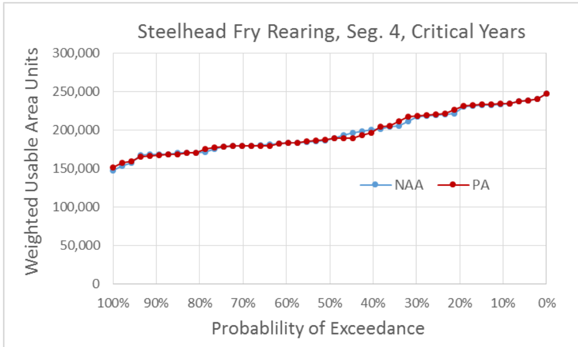
Figure 5.4-223. Exceedance Plot of CCV Steelhead Fry Rearing Weighted Usable Area (WUA) for NAA and PA Model Scenarios in River Segment 4, Critical Water Years
