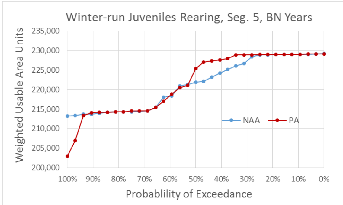
Figure 5.4-95. Exceedance Plot of Winter-Run Chinook Salmon Juvenile Rearing Weighted Usable Area (WUA) for NAA and PA Model Scenarios in River Segment 5, Below Normal Water Years
