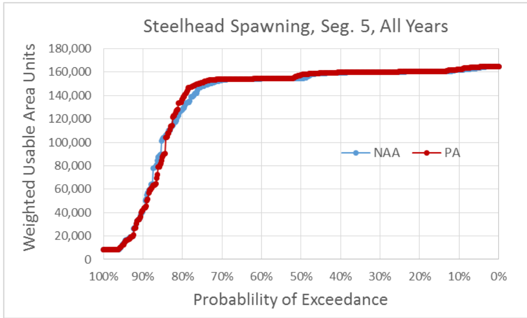
Figure 5.4-186. Exceedance Plot of Central Valley Steelhead Spawning Weighted Usable Area (WUA) for NAA and PA Model Scenarios in River Segment 5, All Water Years
