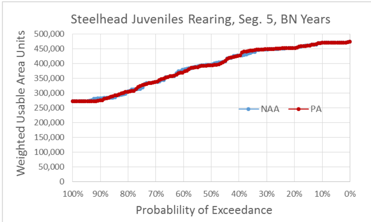
Figure 5.4-233. Exceedance Plot of CCV Steelhead Juvenile Rearing Weighted Usable Area (WUA) for NAA and PA Model Scenarios in River Segment 5, Below Normal Water Years
