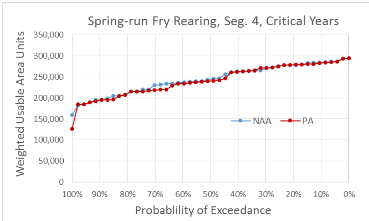
Figure 5.4-158. Exceedance Plot of Spring-Run Chinook Salmon Fry Rearing Weighted Usable Area (WUA) for NAA and PA Model Scenarios in River Segment 4, Critical Water Years
