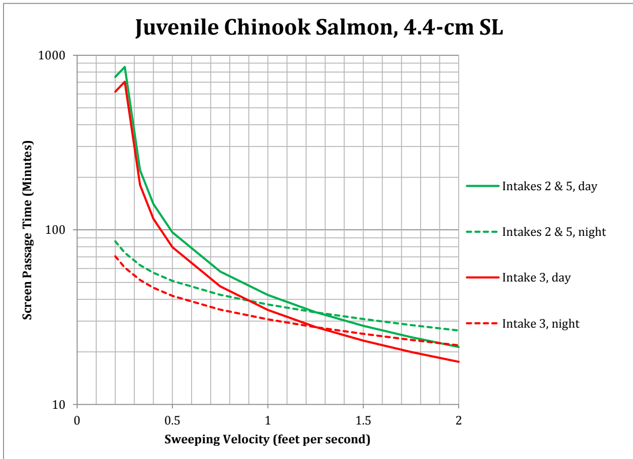
Figure 5.4-1. Estimated Screen Passage Time for Juvenile Chinook Salmon (4.4-cm Standard Length) Encountering Proposed NDD Fish Screens at Approach Velocity of 0.2 Feet per Second during the Day and Night.
