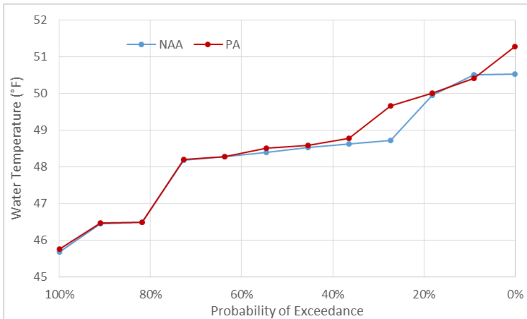
Figure 5.4-204. Exceedance Plot of Mean Monthly Water Temperatures (°F) in the Sacramento River at Bend Bridge in February of Critical Water Years
