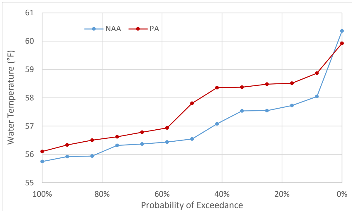
Figure 5.4-56. Exceedance Plot of Mean Monthly Water Temperatures (°F) in the Sacramento River at Red Bluff in September of Above Normal Water Years
