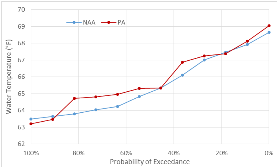
Figure 5.4-244. Exceedance Plot of Mean Monthly Water Temperatures (°F) in the Sacramento River at Hamilton City in July of Critical Water Years
