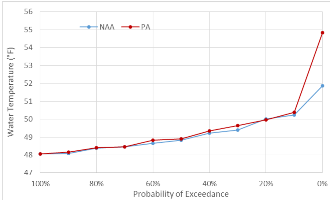
Figure 5.4-242. Exceedance Plot of Mean Monthly Water Temperatures (°F) in the Sacramento River at Keswick Dam in May of Below Normal Water Years
