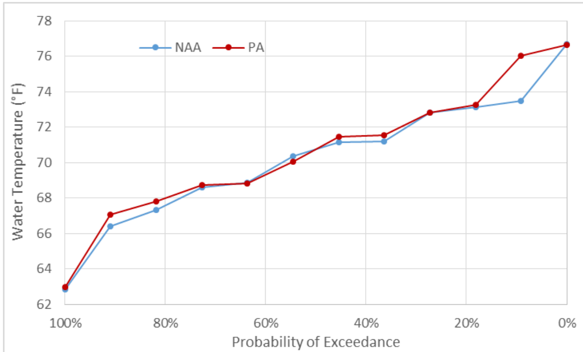
Figure 5.4-263. Exceedance Plot of Mean Monthly Water Temperatures (°F) in the American River at Watt Avenue in June of Critical Water Years
