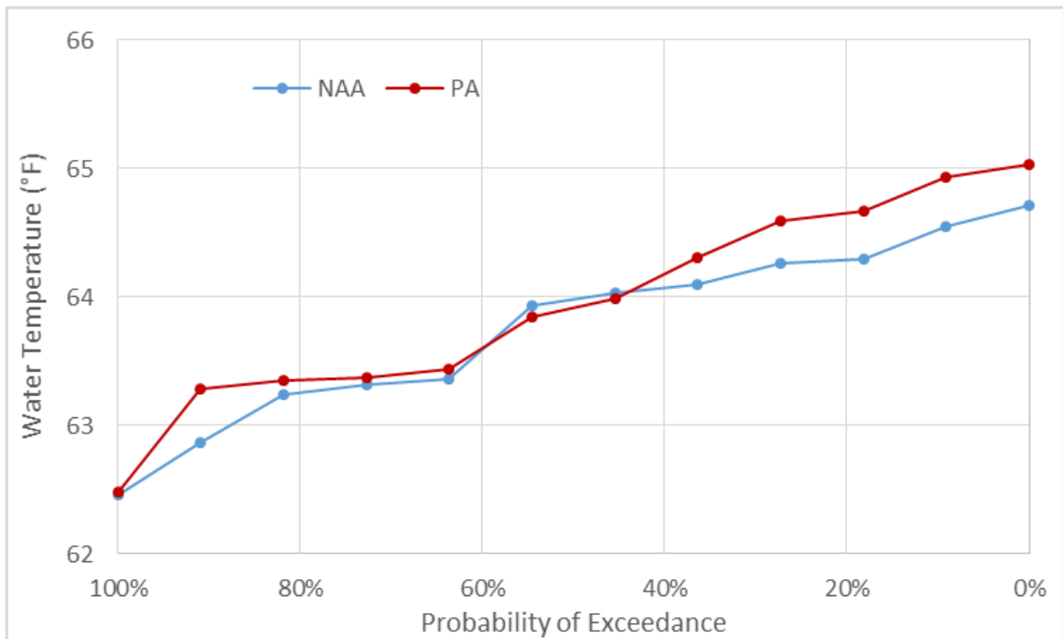
Figure 5.4-265. Exceedance Plot of Mean Monthly Water Temperatures (°F) in the American River at Watt Avenue in October of Above Normal Water Years
