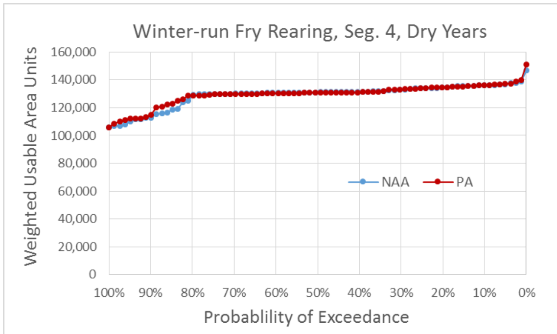
Figure 5.4-84. Exceedance Plot of Winter-Run Chinook Salmon Fry Rearing Weighted Usable Area (WUA) for NAA and PA Model Scenarios in River Segment 4, Dry Water Years
