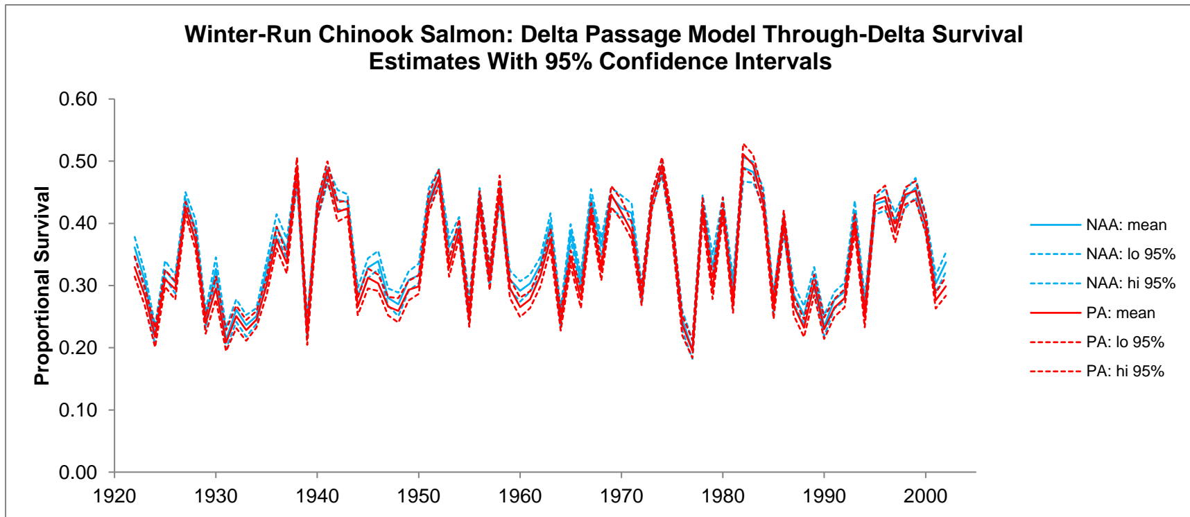
Figure 5.4-9. Time Series of Mean (With 95% Confidence Interval) Annual Juvenile Winter-Run Chinook Salmon Through-Delta Survival Estimated from the Delta Passage Model.
