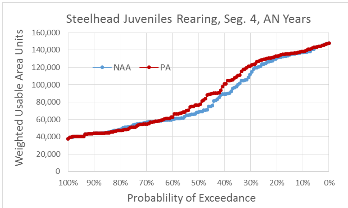
Figure 5.4-238. Exceedance Plot of CCV Steelhead Juvenile Rearing Weighted Usable Area (WUA) for NAA and PA Model Scenarios in River Segment 4, Above Normal Water Years
