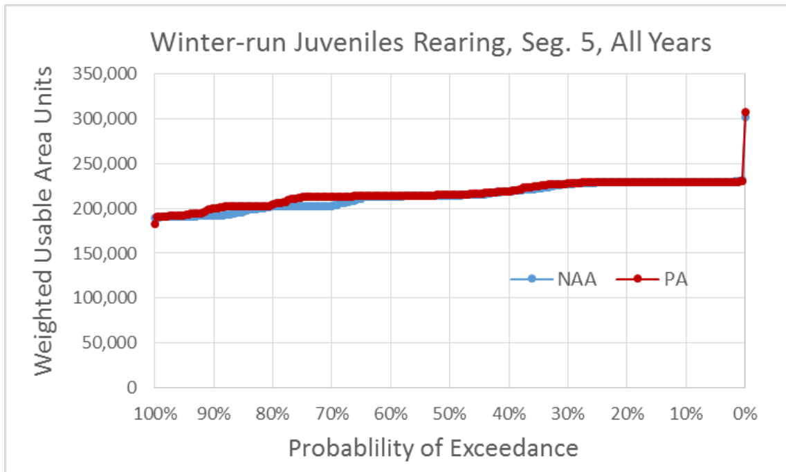
Figure 5.4-92. Exceedance Plot of Winter-Run Chinook Salmon Juvenile Rearing Weighted Usable Area (WUA) for NAA and PA Model Scenarios in River Segment 5, All Water Years
