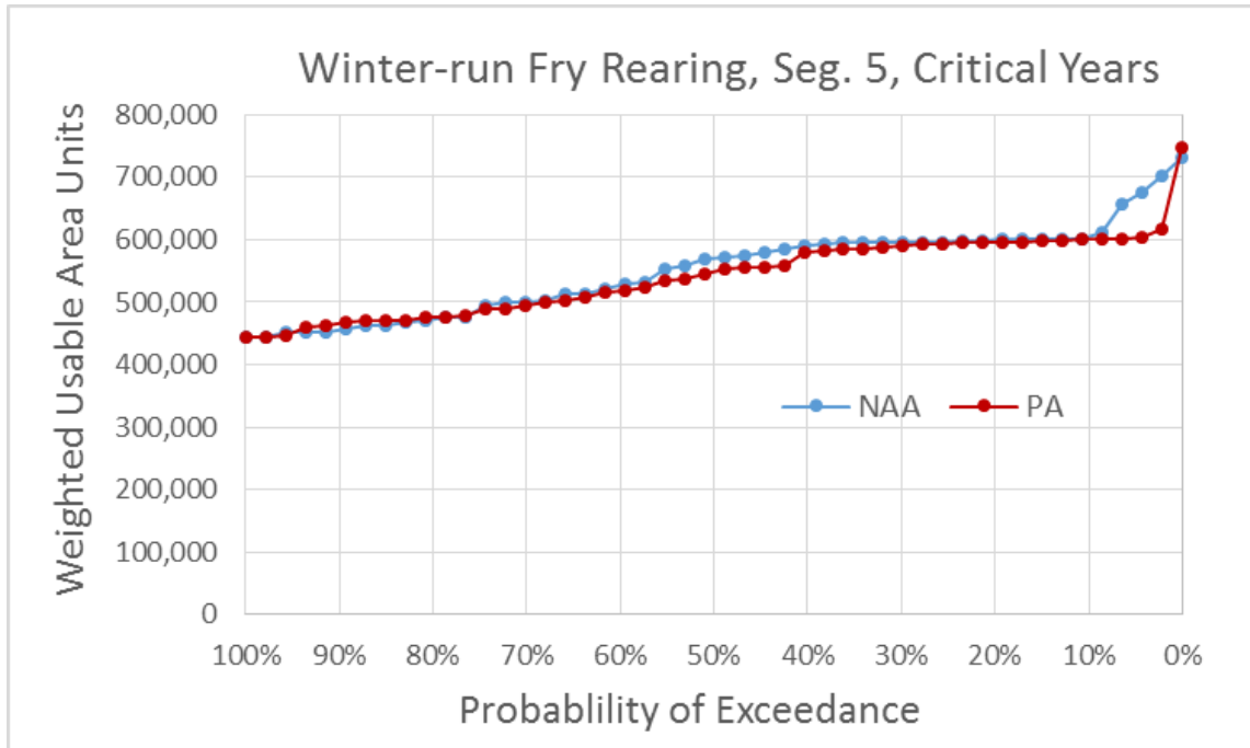
Figure 5.4-79. Exceedance Plot of Winter-Run Chinook Salmon Fry Rearing Weighted Usable Area (WUA) for NAA and PA Model Scenarios in River Segment 5, Critical Water Years
