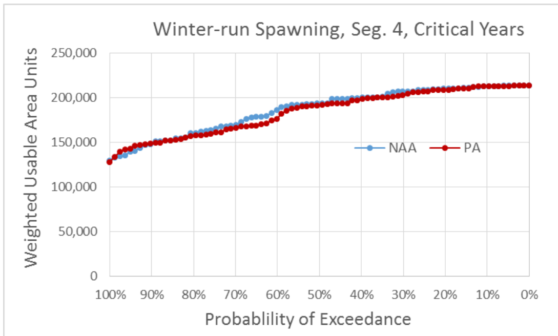
Figure 5.4-47. Exceedance Plot of Winter-Run Chinook Salmon Spawning Weighted Usable Area (WUA) for NAA and PA Model Scenarios in River Segment 4, Critical Water Years
