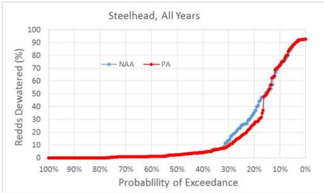
Figure 5.4-198. Exceedance Plot of Central Valley Steelhead Percent of Redds Dewatered for NAA and PA Model Scenarios, All Water Years
