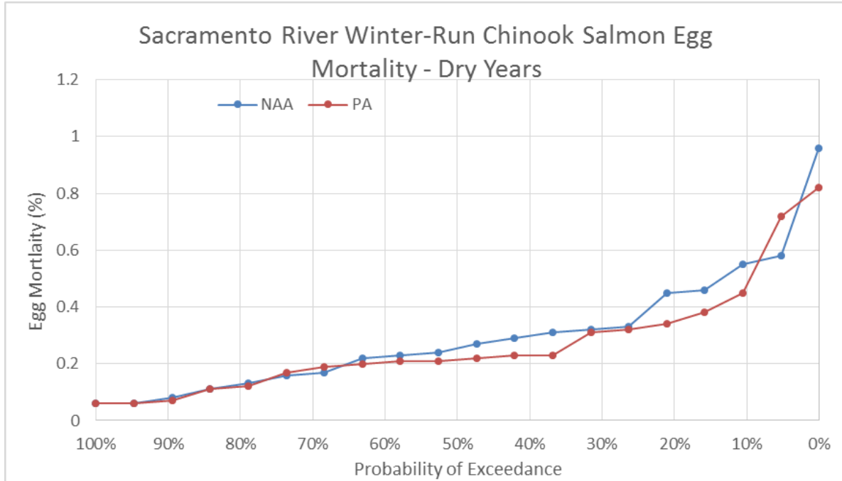
Figure 5.4-65. Exceedance Plot of Winter-Run Chinook Salmon Egg Mortality for NAA and PA Model Scenarios, Reclamation Egg Mortality Model, Dry Water Years
