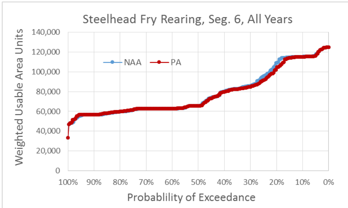
Figure 5.4-206. Exceedance Plot of CCV Steelhead Fry Rearing Weighted Usable Area (WUA) for NAA and PA Model Scenarios in River Segment 6, All Water Years
