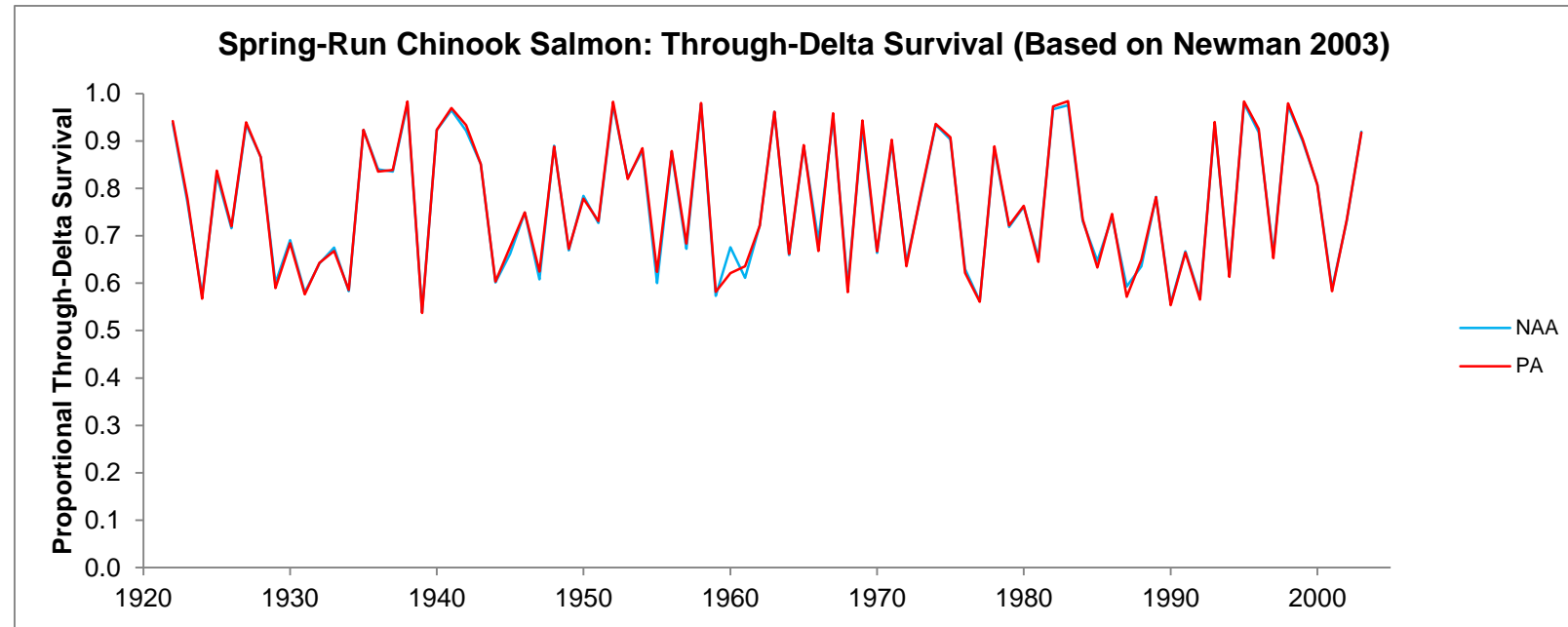
Figure 5.4-16. Time Series of Spring-Run Chinook Salmon Annual Through-Delta Survival Estimated from the Analysis Based on Newman (2003).
