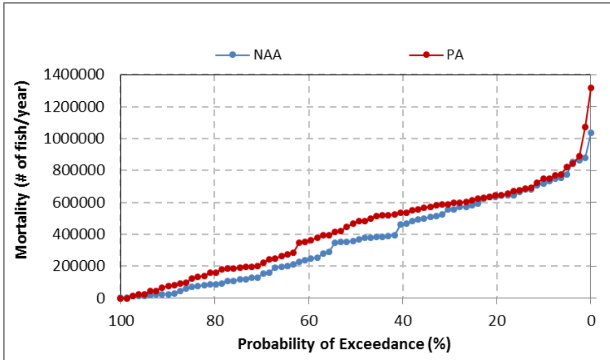
Figure 5.4-54. Exceedance Plot of Annual Flow-Based Mortality (#of Fish/Year) of Winter-Run Chinook Salmon Spawning, Egg Incubation, and Alevins
