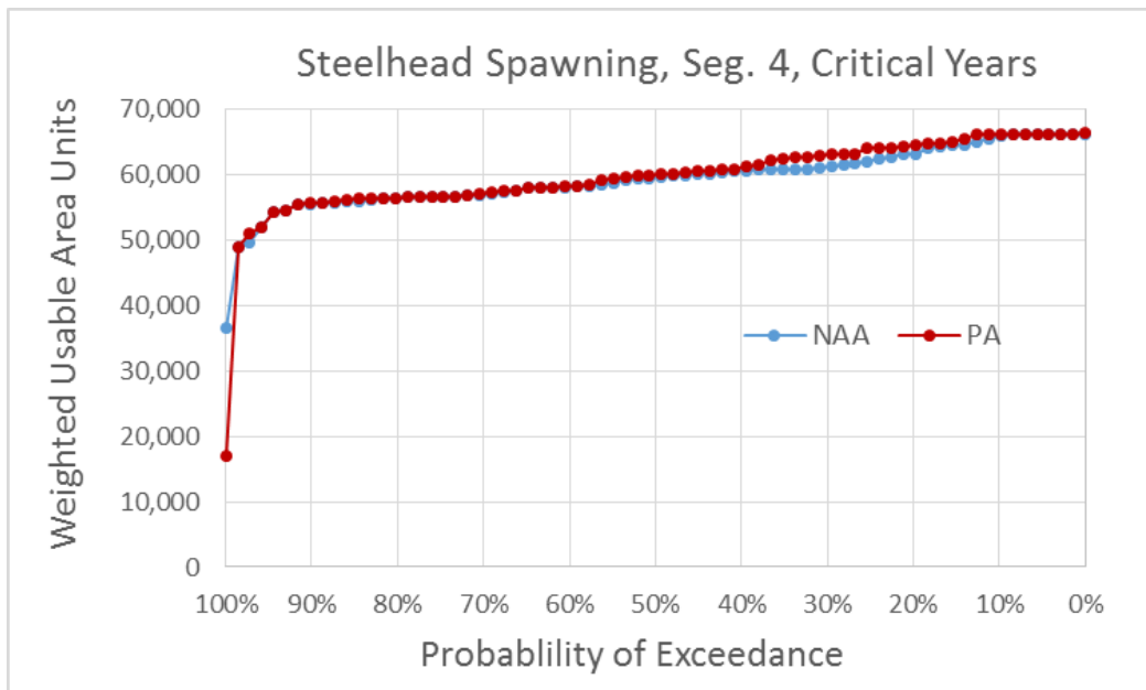
Figure 5.4-197. Exceedance Plot of Central Valley Steelhead Spawning Weighted Usable Area (WUA) for NAA and PA Model Scenarios in River Segment 4, Critical Water Years
