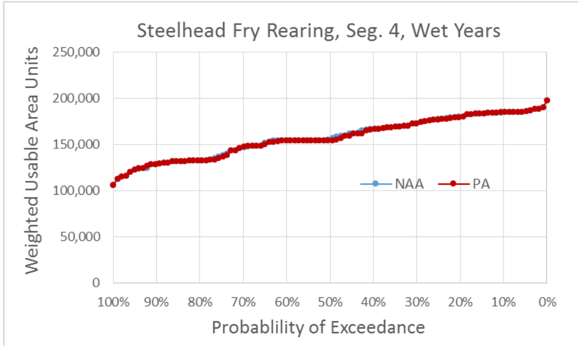
Figure 5.4-219. Exceedance Plot of CCV Steelhead Fry Rearing Weighted Usable Area (WUA) for NAA and PA Model Scenarios in River Segment 4, Wet Water Years
