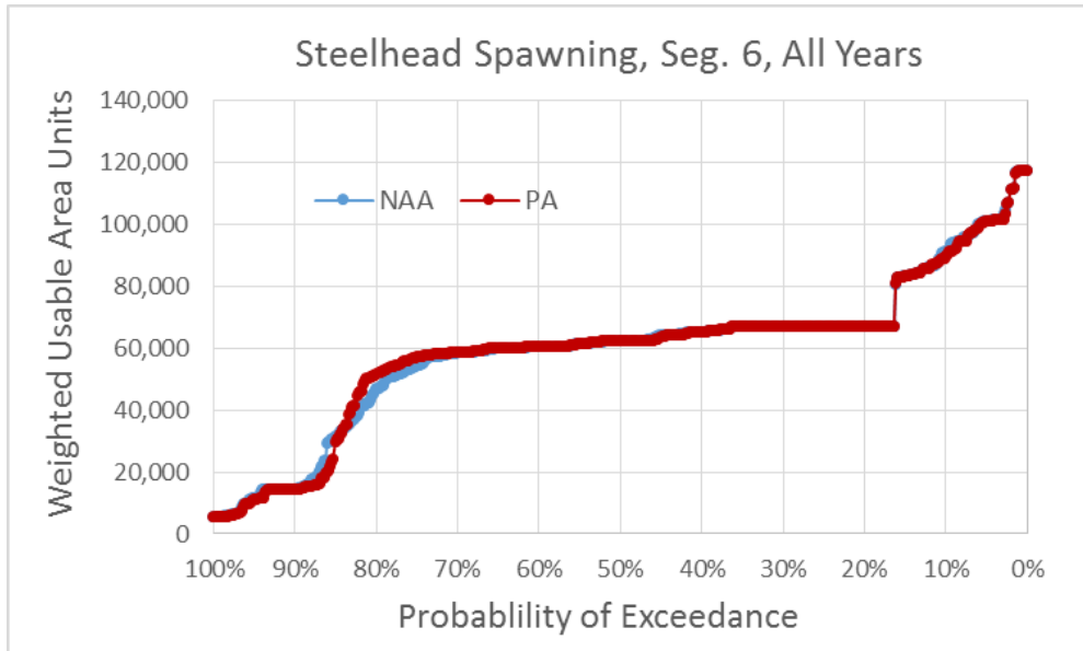
Figure 5.4-180. Exceedance Plot of Central Valley Steelhead Spawning Weighted Usable Area (WUA) for NAA and PA Model Scenarios in River Segment 6, All Water Years
