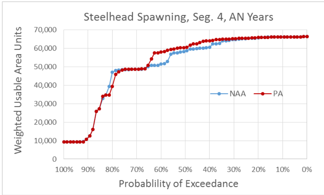
Figure 5.4-194. Exceedance Plot of Central Valley Steelhead Spawning Weighted Usable Area (WUA) for NAA and PA Model Scenarios in River Segment 4, Above Normal Water Years
