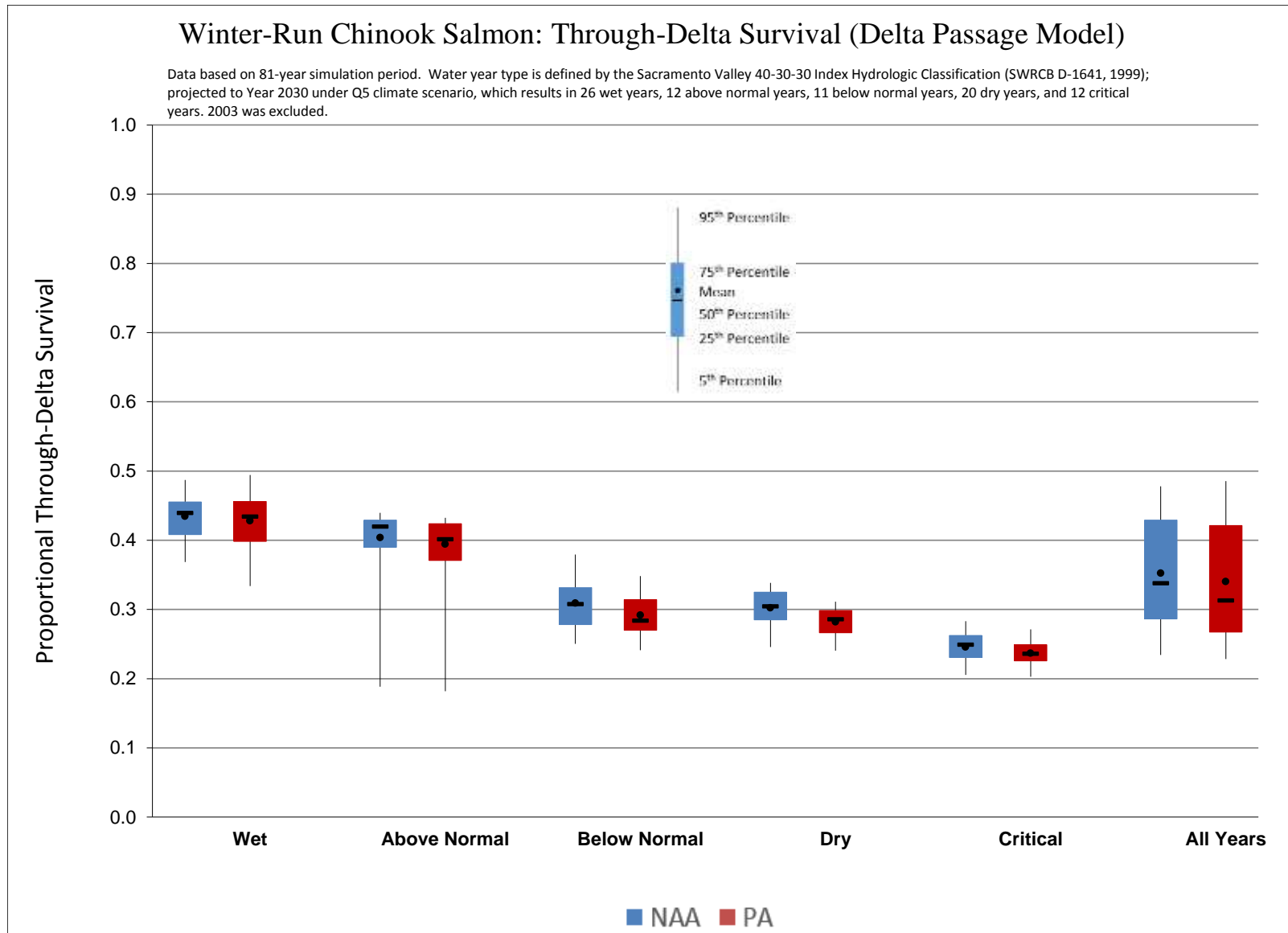
Figure 5.4-7. Box Plots of Winter-Run Chinook Salmon Annual Through-Delta Survival Estimated from the Delta Passage Model, Grouped by Water Year Type.
