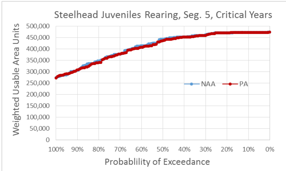
Figure 5.4-235. Exceedance Plot of CCV Steelhead Juvenile Rearing Weighted Usable Area (WUA) for NAA and PA Model Scenarios in River Segment 5, Critical Water Years
