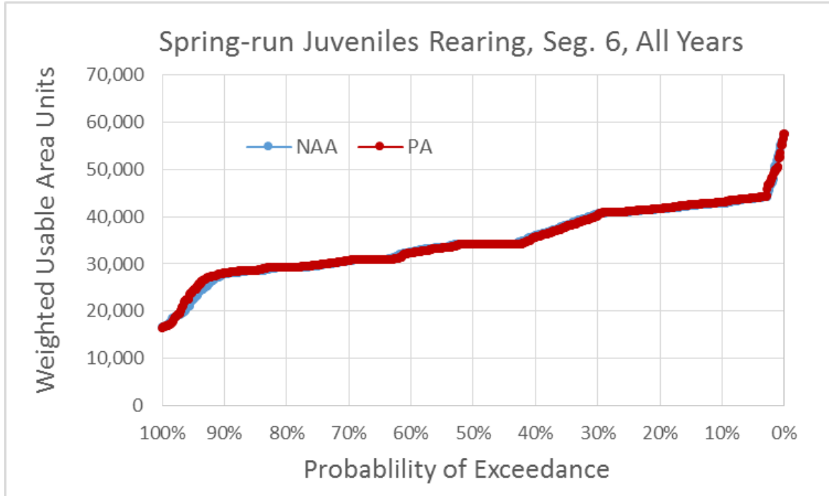
Figure 5.4-159. Exceedance Plot of Spring-Run Chinook Salmon Juvenile Rearing Weighted Usable Area (WUA) for NAA and PA Model Scenarios in River Segment 6, All Water Years
