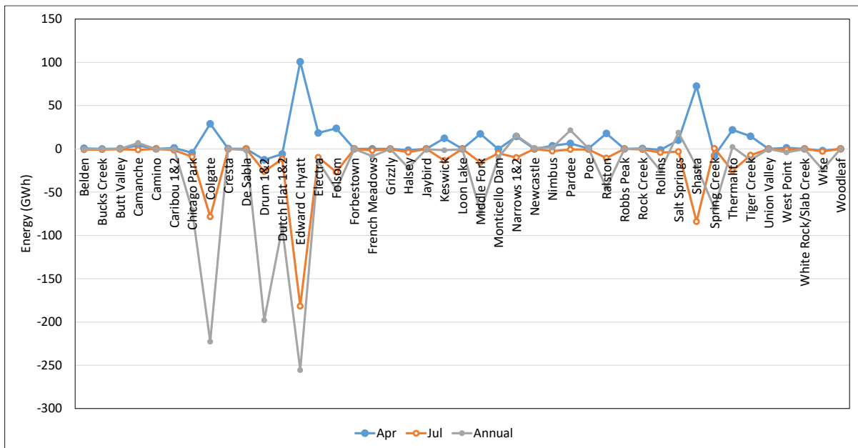
Figure A5-19. Estimated Average Change in Hydropower Generation for the 65 Scenario at Individual Hydropower Facilities
