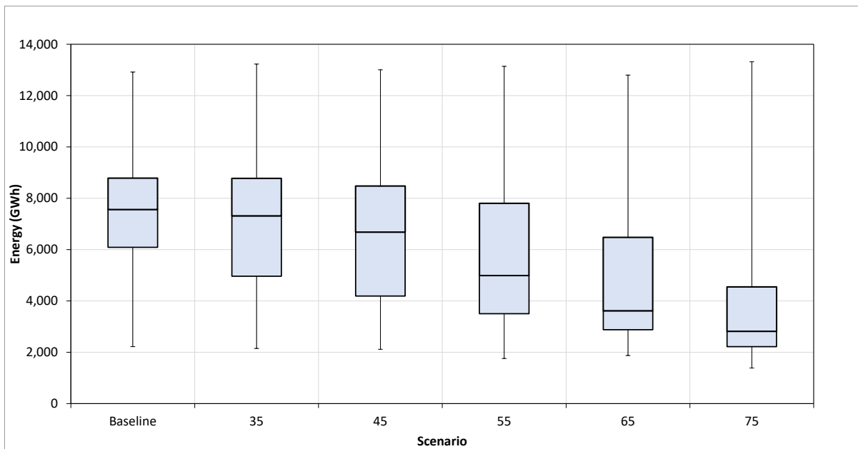
Figure A5-29. Estimated Monthly Changes in Energy Required for CVP and SWP Exports
