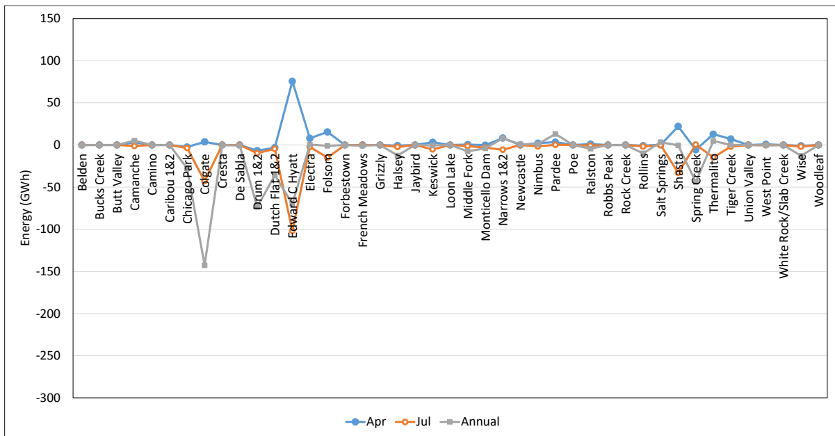
Figure A5-17. Estimated Average Change in Hydropower Generation for the 45 Scenario at Individual Hydropower Facilities
