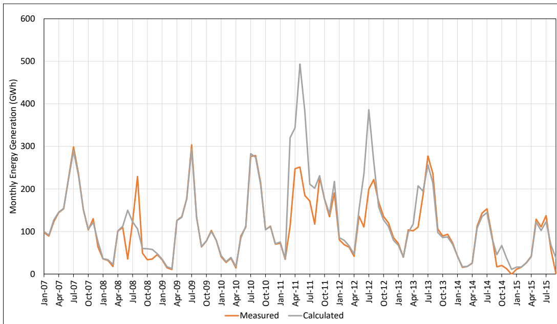
Figure A5-10. Comparison of Measured and Calculated Hydropower Generation at Hyatt Power Plant for 2007–2015
