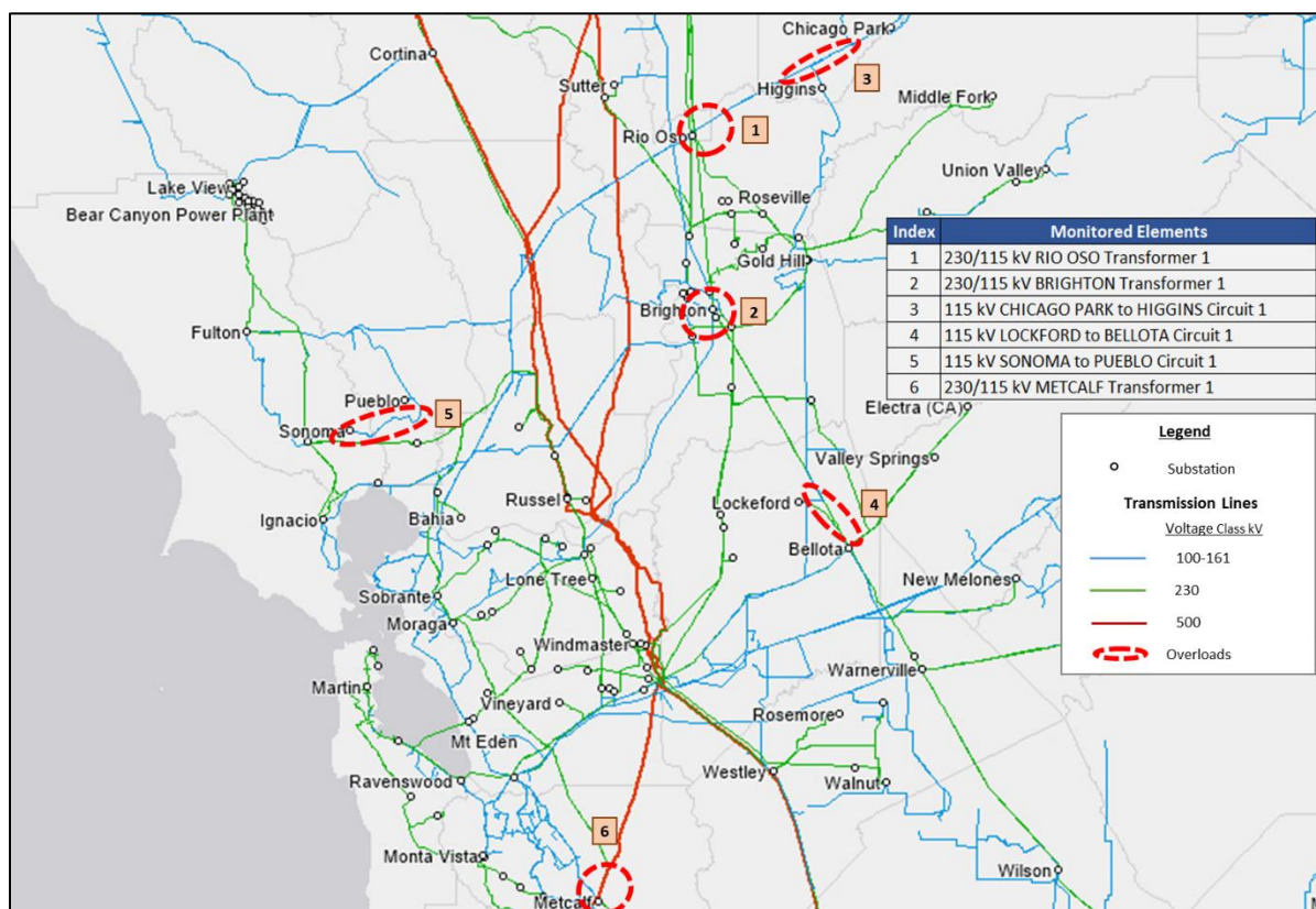
Figure A5-27. Location of Overloaded Transmission Facilities (Transmission Lines and Transformers) Prior to Generation Redispatch
