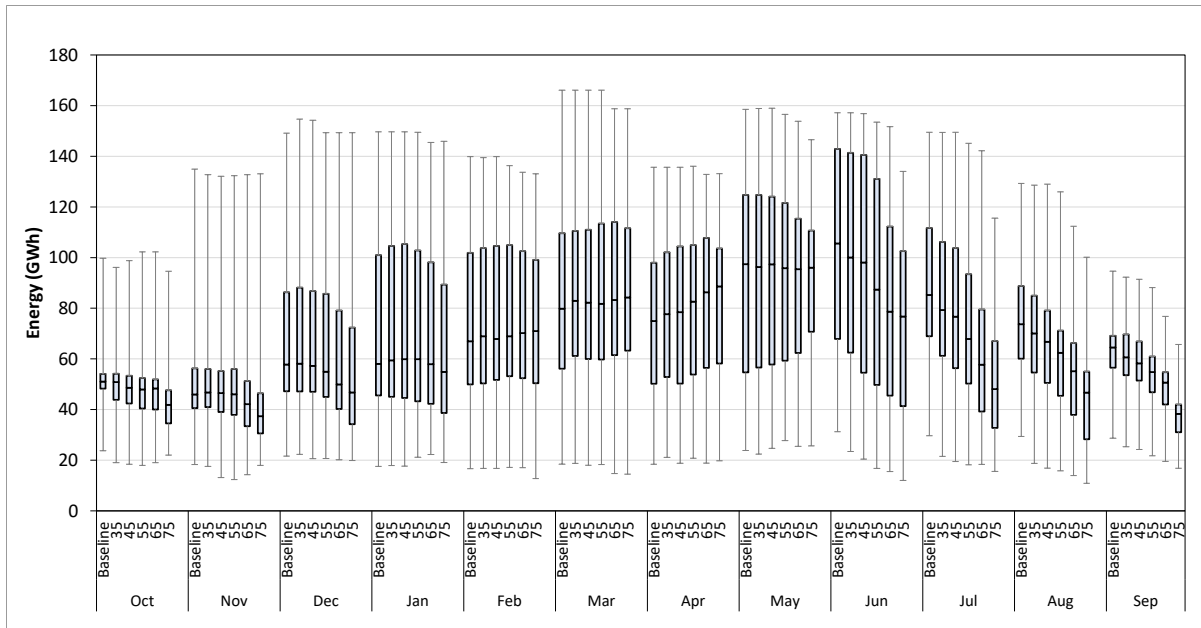
Figure A5-21. Monthly Changes in Hydropower Generation at Sixteen Renewables Portfolio Standard Facilities Potentially Subject to Changes in Flow
