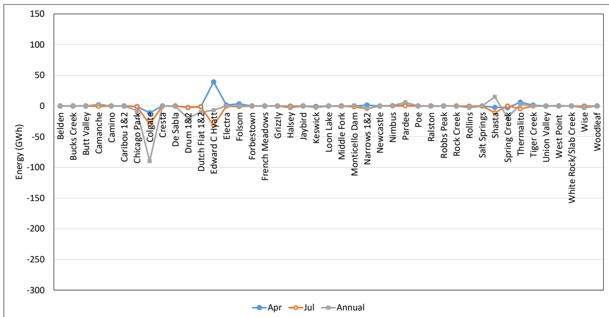
Figure A5-16. Estimated Average Change in Hydropower Generation for the 35 Scenario at Individual Hydropower Facilities
