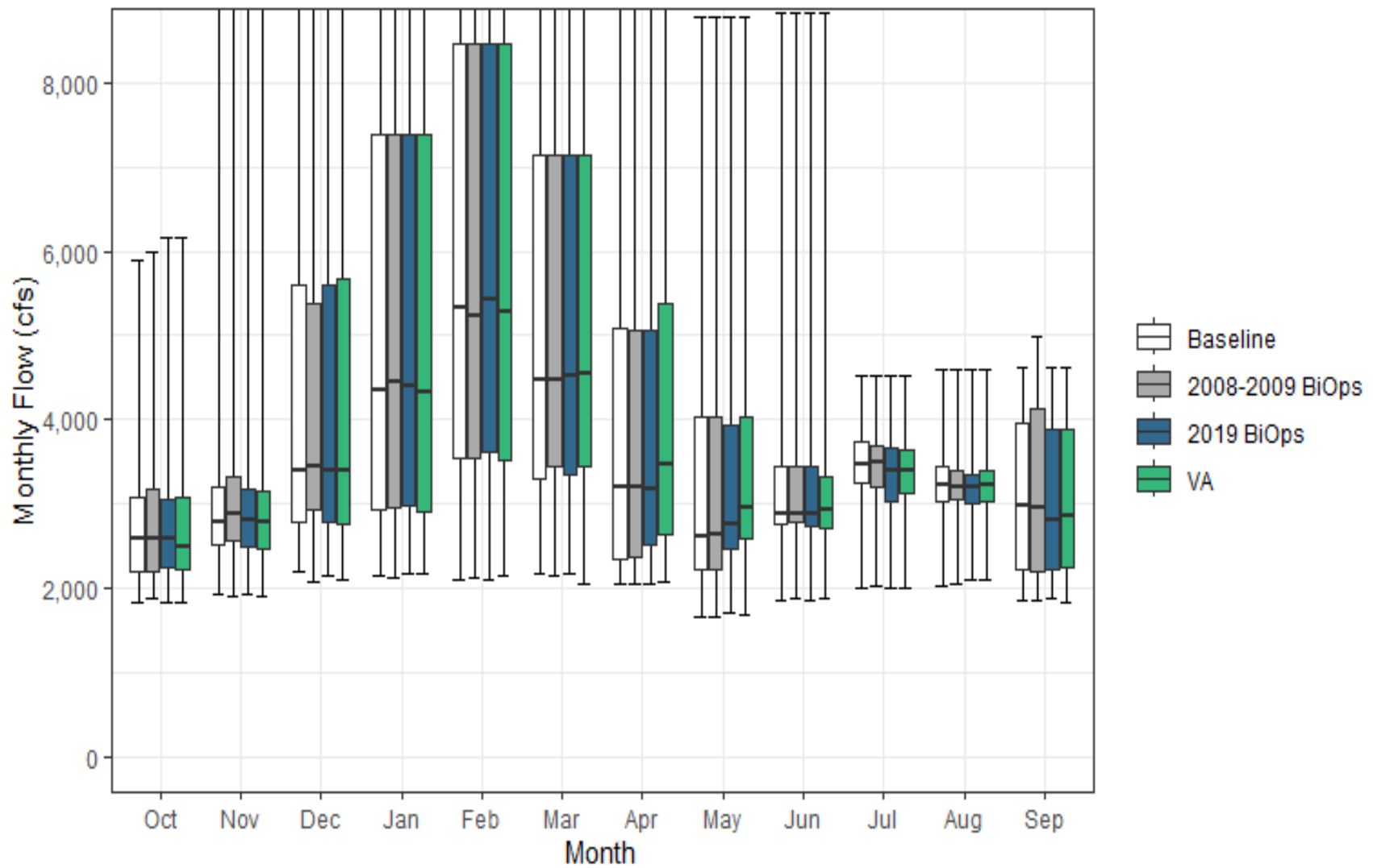
Figure G3a-34. Georgiana Slough Monthly Boxplot
