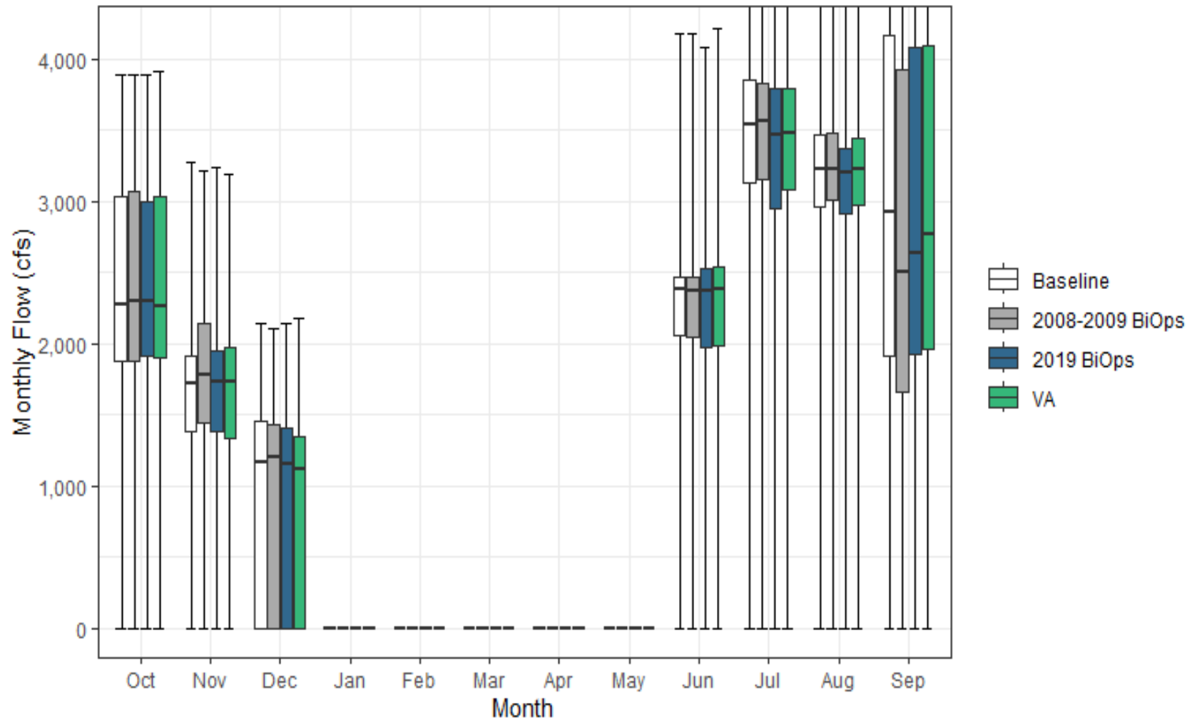
Figure G3a-33. Delta Cross Channel Monthly Boxplot
