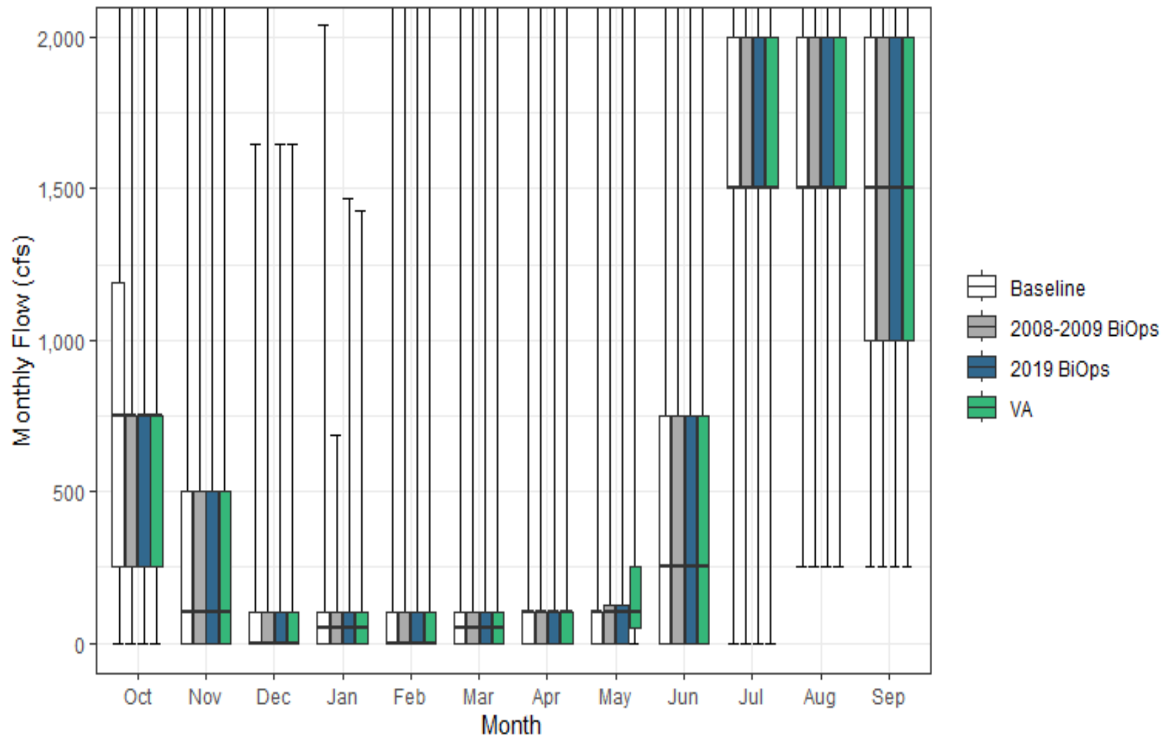
Figure G3a-45. Clear Creek Tunnel Monthly Boxplot
