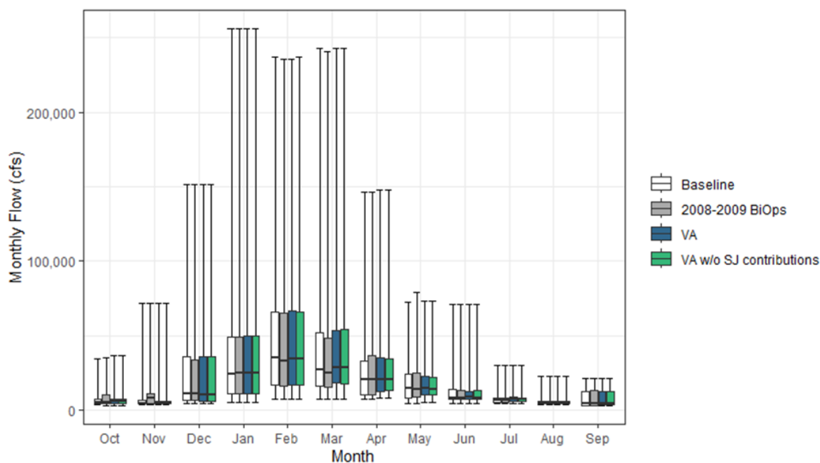
Figure G3a-2. Baseline, 2008-2009 BiOps, and VA Modeled Flow Including Postprocessed Components (cfs), Delta Outflow
