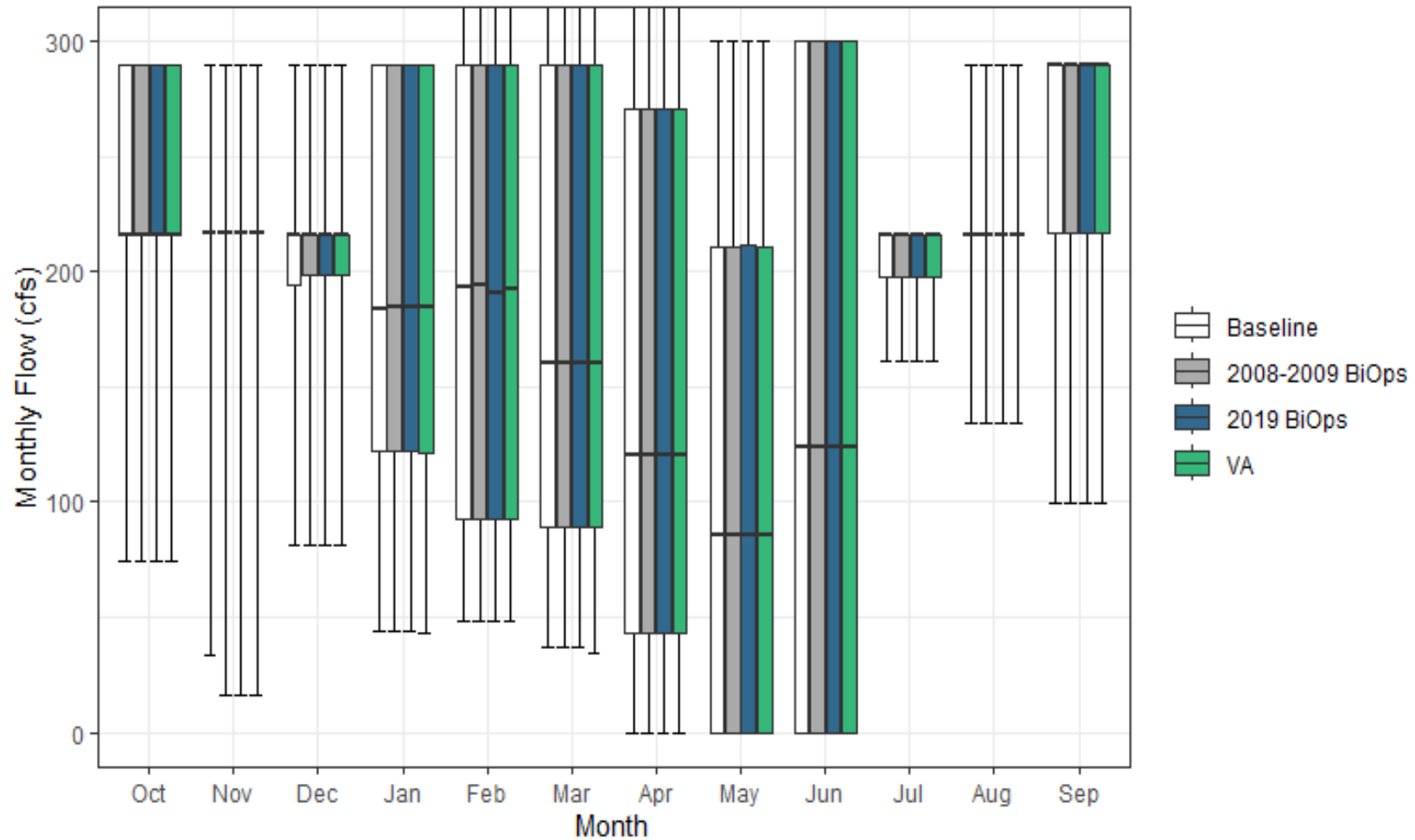
Figure G3a-39. Bowman-Spaulding Conduit Monthly Boxplot
