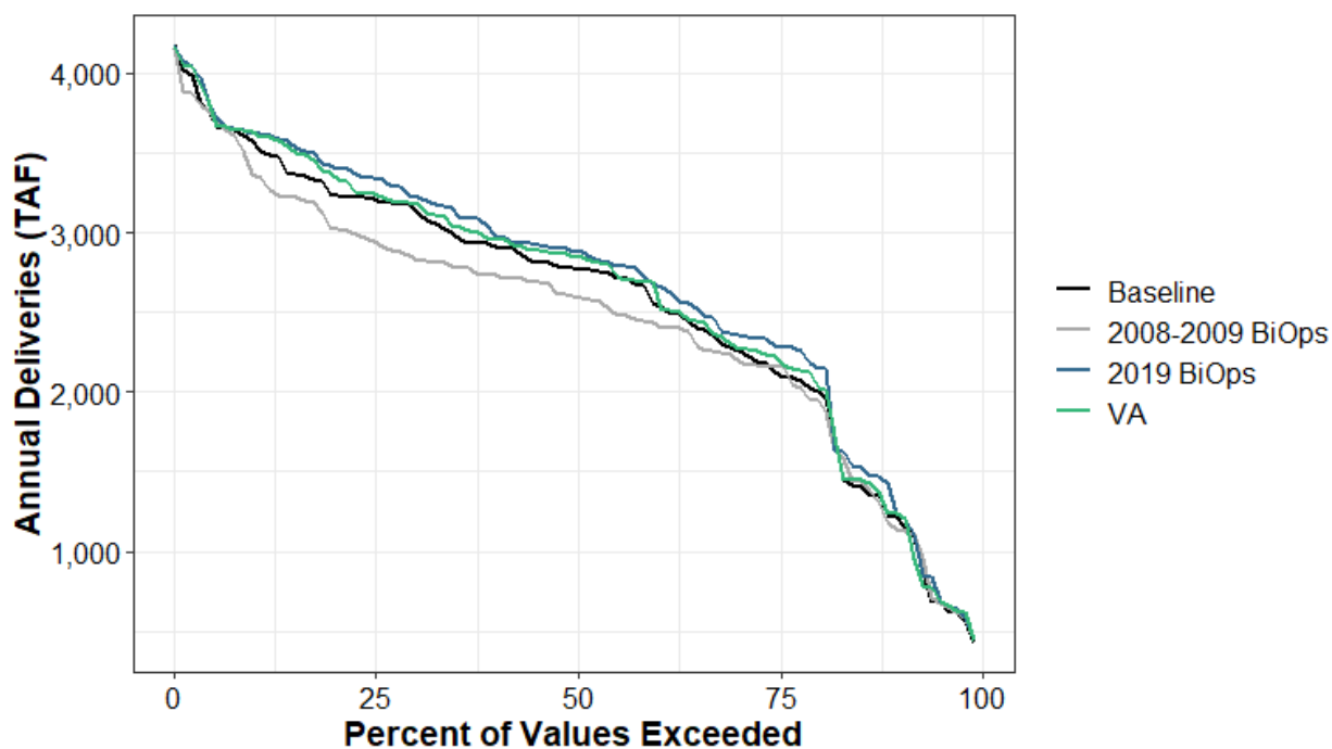
Figure G3a-112. Surface Water Supplied to Total SWP Table A Annual Percent Exceedance Plot
