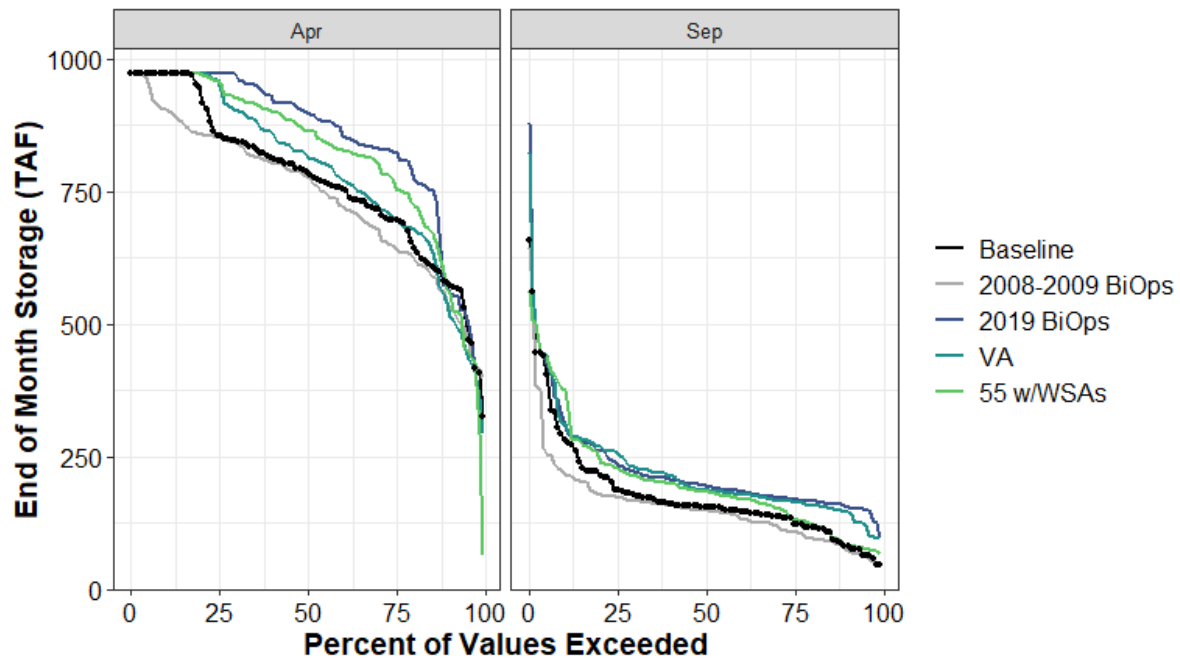
Figure H1a2-85. CVP San Luis Reservoir End of April and End of September Storage (TAF) Percent Exceedance Plot
