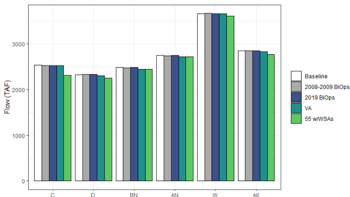
Figure H1a2-235. Total Average Annual Groundwater Recharge for the Sacramento River Watershed by WYT and Scenario (TAF/yr).
