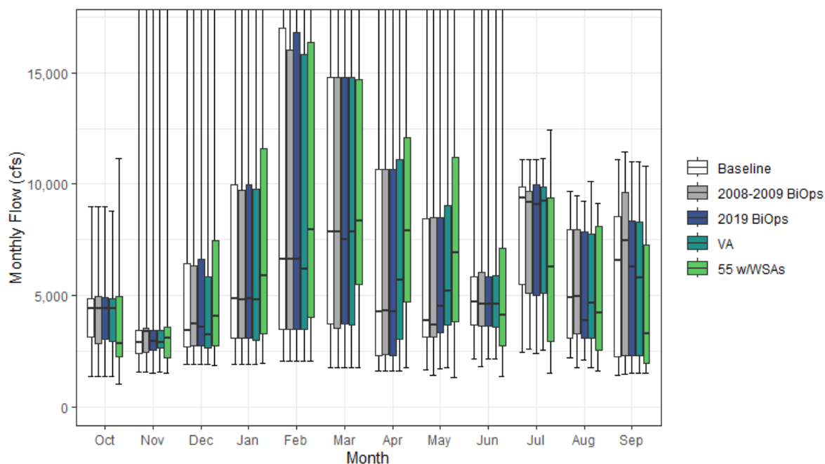
Figure H1a2-20. Feather River Streamflow above Confluence with Sacramento River Monthly Boxplot (cfs)
