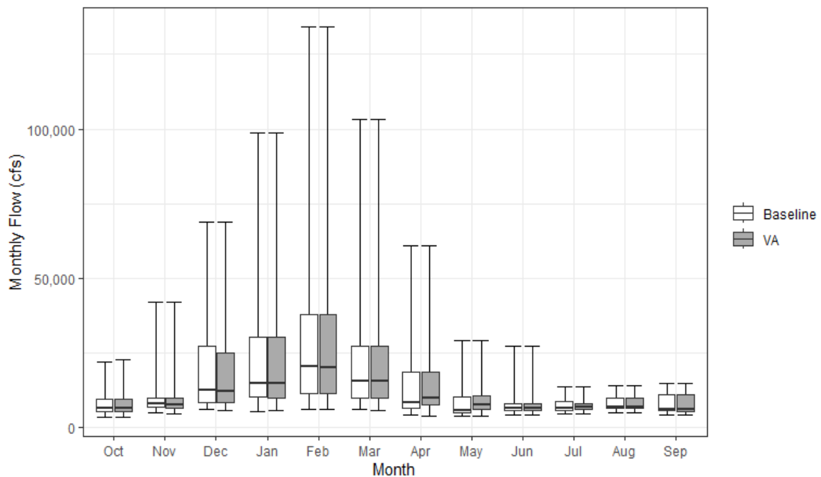
Figure 9.5-3. Sacramento River Inflow under Baseline and Proposed VAs
