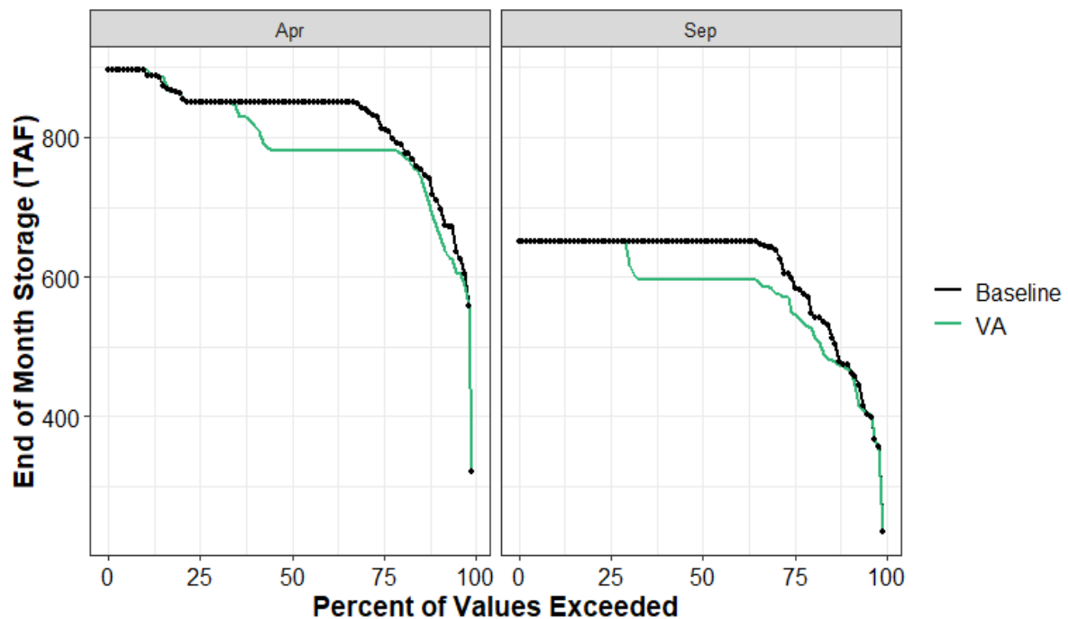
Figure 9.5-10. New Bullards Bar Reservoir End of April and End of September Carryover Storage under Baseline and Proposed VAs
