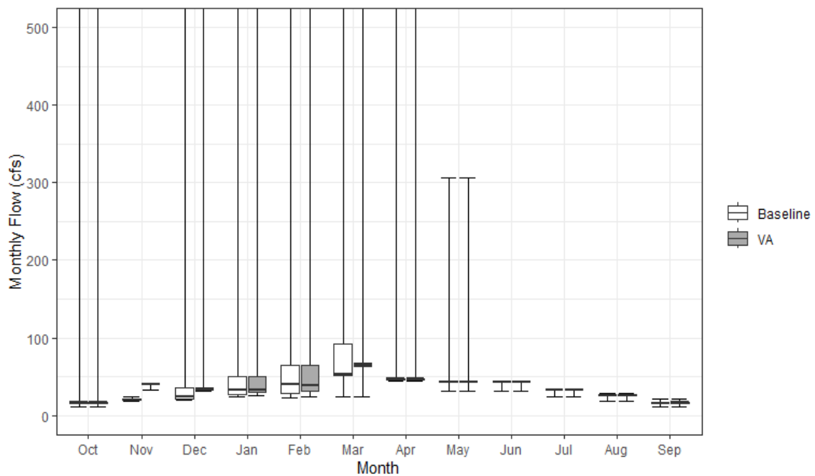
Figure 9.5-17. Monthly Streamflow for Putah Creek above the Yolo Bypass under Baseline and Proposed VAs
