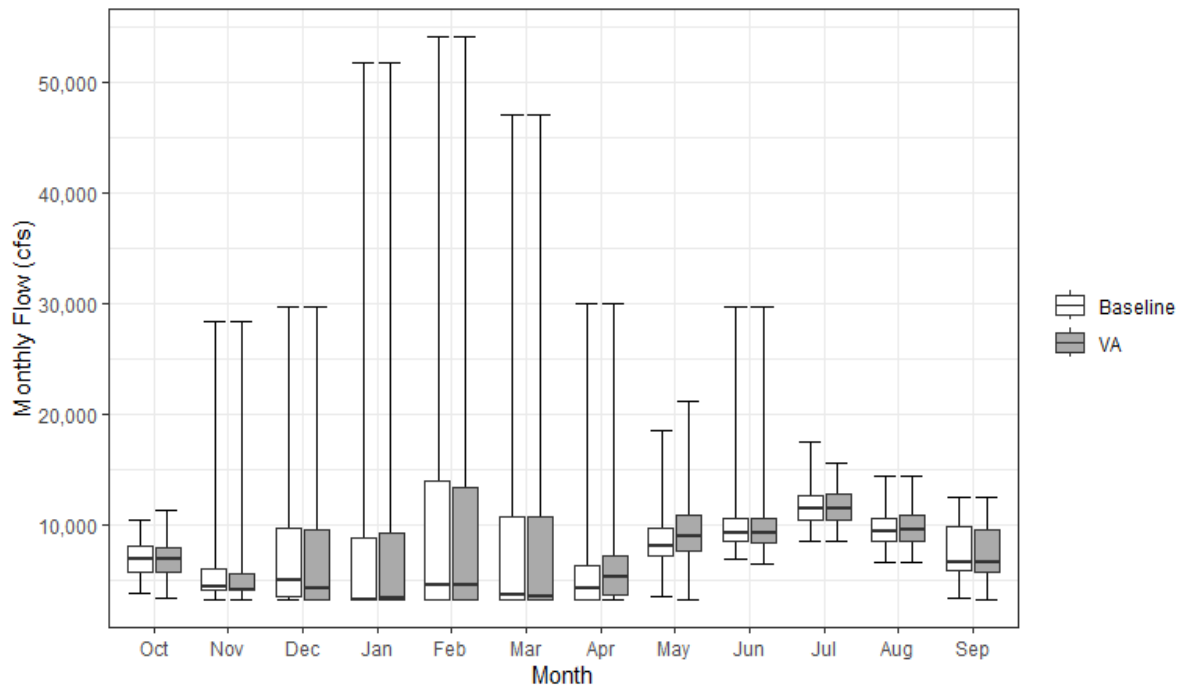
Figure 9.5-2. Monthly Streamflow of the Sacramento River below Keswick Reservoir under Baseline and Proposed VAs
