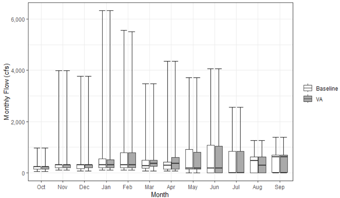
Figure 9.5-15. Monthly Streamflow for the Mokelumne River above the Confluence with the Cosumnes River under Baseline and Proposed VAs
