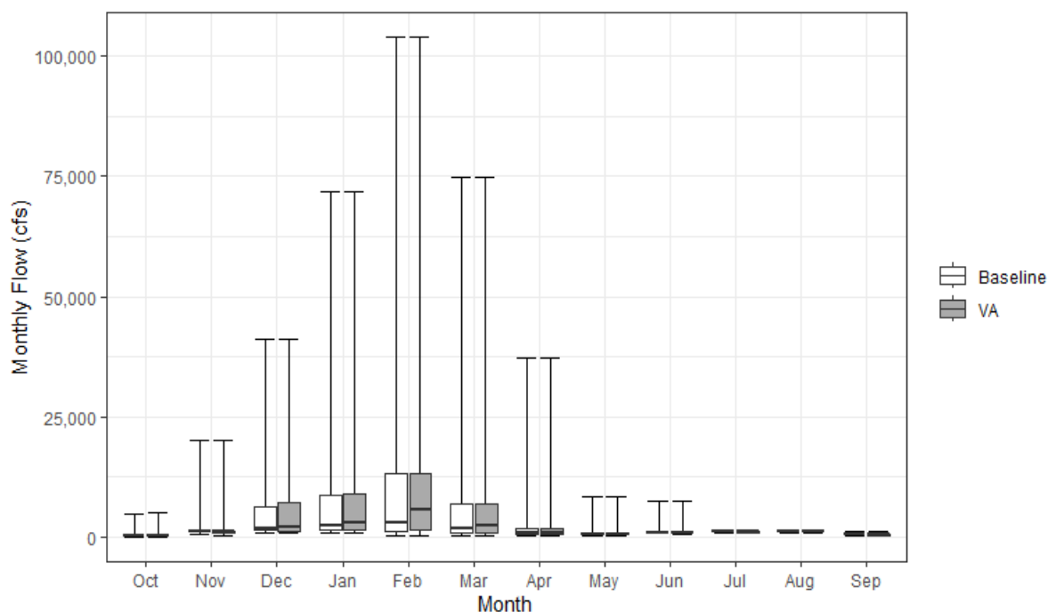
Figure 9.5-6. Monthly Streamflow at Sacramento Slough (Downstream End of Sutter Bypass) under Baseline and Proposed VA
