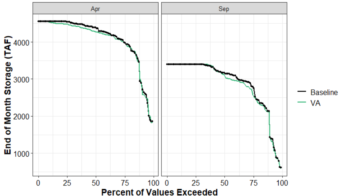
Figure 9.5-1. Change in Shasta Reservoir End of April and End of September Carryover Storage under Baseline and Proposed VAs
