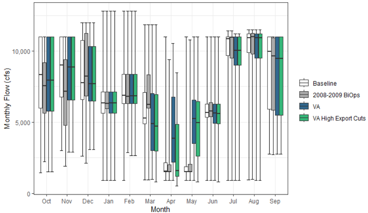
Figure 9.5-19. Monthly South of Delta Exports for Baseline, 2008–2009 BiOps Condition, VA, and VA High Export Cuts Scenarios
