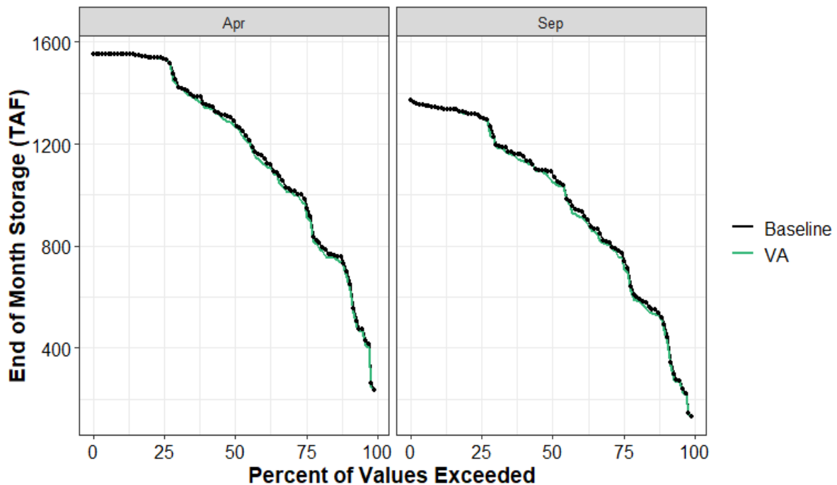
Figure 9.5-16. Lake Berryessa end of April and End of September Carryover Storage under Baseline and Proposed VAs
