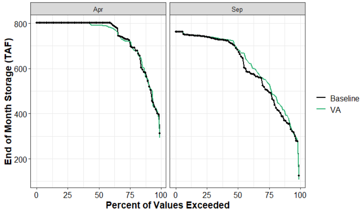
Figure 9.5-12. Folsom Reservoir End of April and End of September Carryover Storage under Baseline and Proposed VAs
