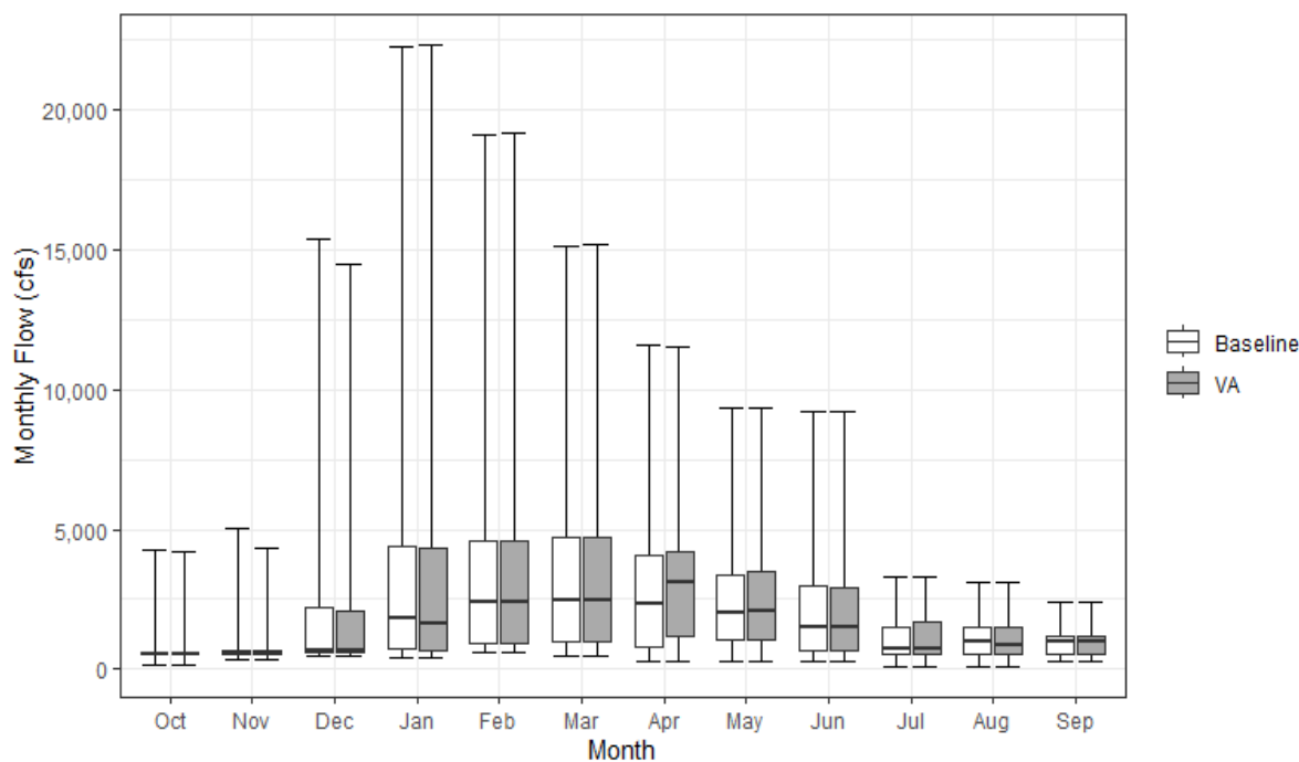
Figure 9.5-11. Monthly Streamflow for the Yuba River above the Feather River under Baseline and Proposed VAs
