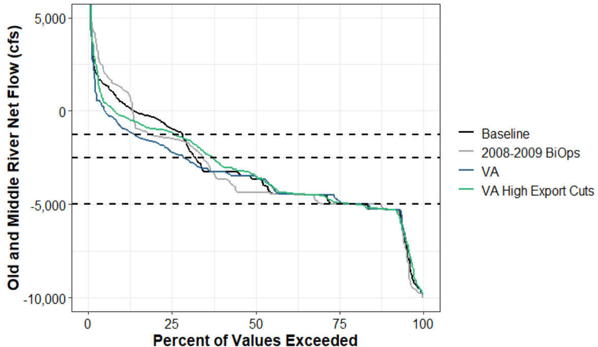
Figure 9.5-20. Monthly Exceedance Frequency Distribution of Old and Middle River Net Flow (cfs) for December–June under Baseline, 2008–2009 BiOps Condition, VA, and VA High Export Cuts Scenarios
