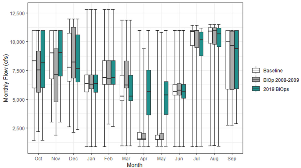
Figure 9.3-2. Monthly CVP and SWP Total South of Delta Exports for Baseline, the 2008–2009 BiOps Condition, and 2019 BiOps Condition
