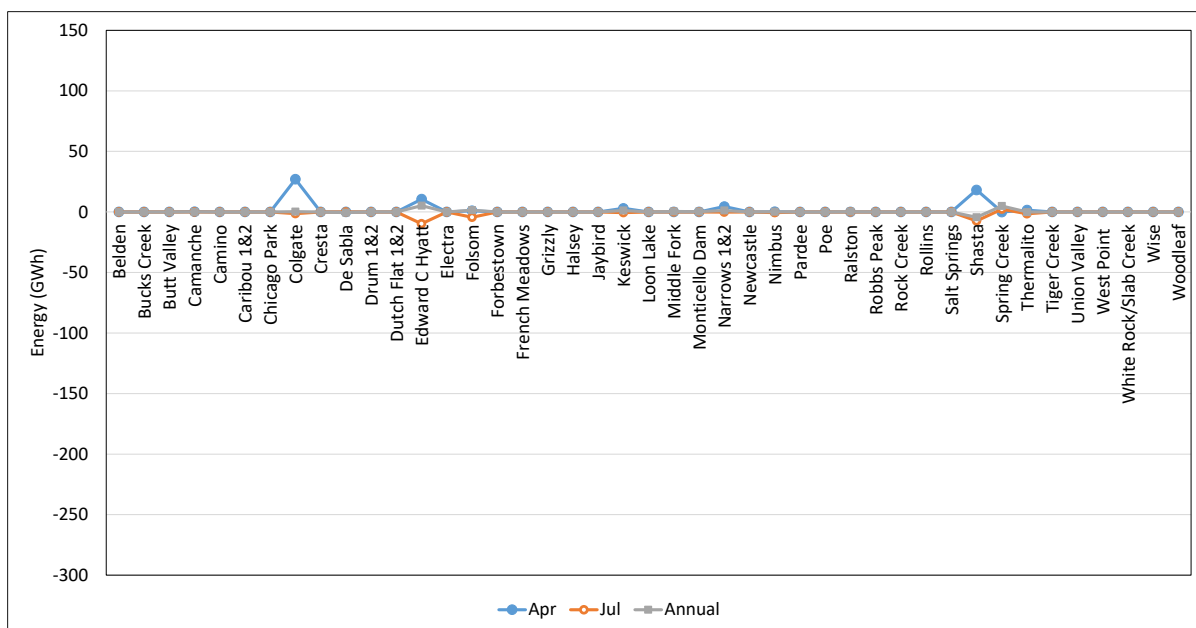
Figure 9.7-4. Estimated Average Change in Hydropower Generation for the VAs at Individual Hydroelectric Facilities
