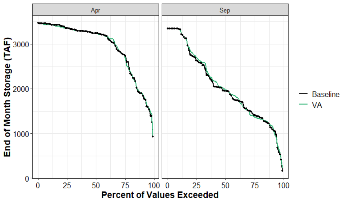
Figure 9.5-7. Oroville Reservoir End of April and End of September Carryover Storage under Baseline and Proposed VAs
