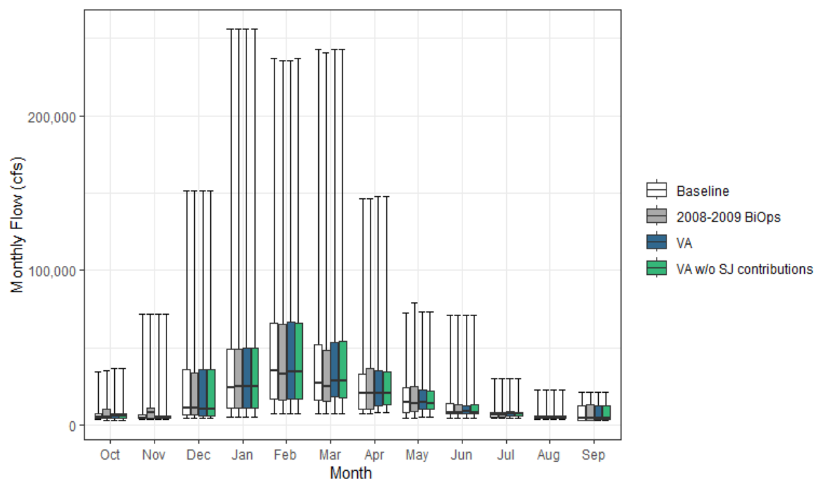
Figure 9.5-22. Monthly Total Delta Outflow for Baseline, 2008–2009 BiOps Condition, VA, and VA without San Joaquin Contributions Scenarios
