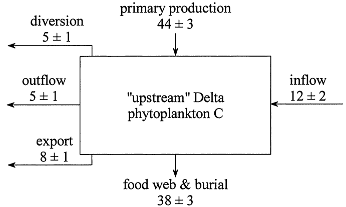
Fig. 9. Phytoplankton C budget (tons d^{-1} \pm SE among years) for the upstream Delta, averaged for March–October during 1975–1993. Primary (net) production is estimated as described in this publication. Inflow, outflow, diversion, and export are estimated as described by Jassby and Cloern (2000). Food web and burial is the residual amount required to balance the other flows.
