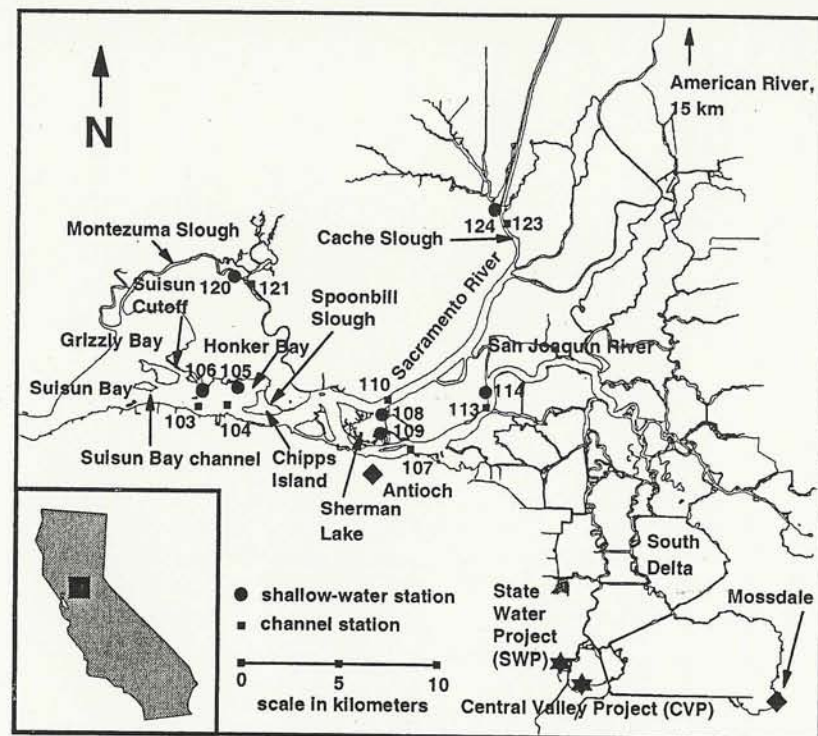
Figure 1. Delta smelt purse-seining stations in the Sacramento-San Joaquin Estuary.
