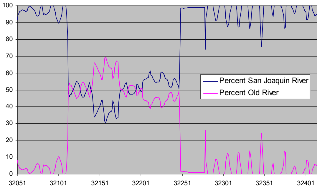
Flow Split Percentages: Old River and San Joaquin River, Case 1 SDIP HORB, Water Year 1988
