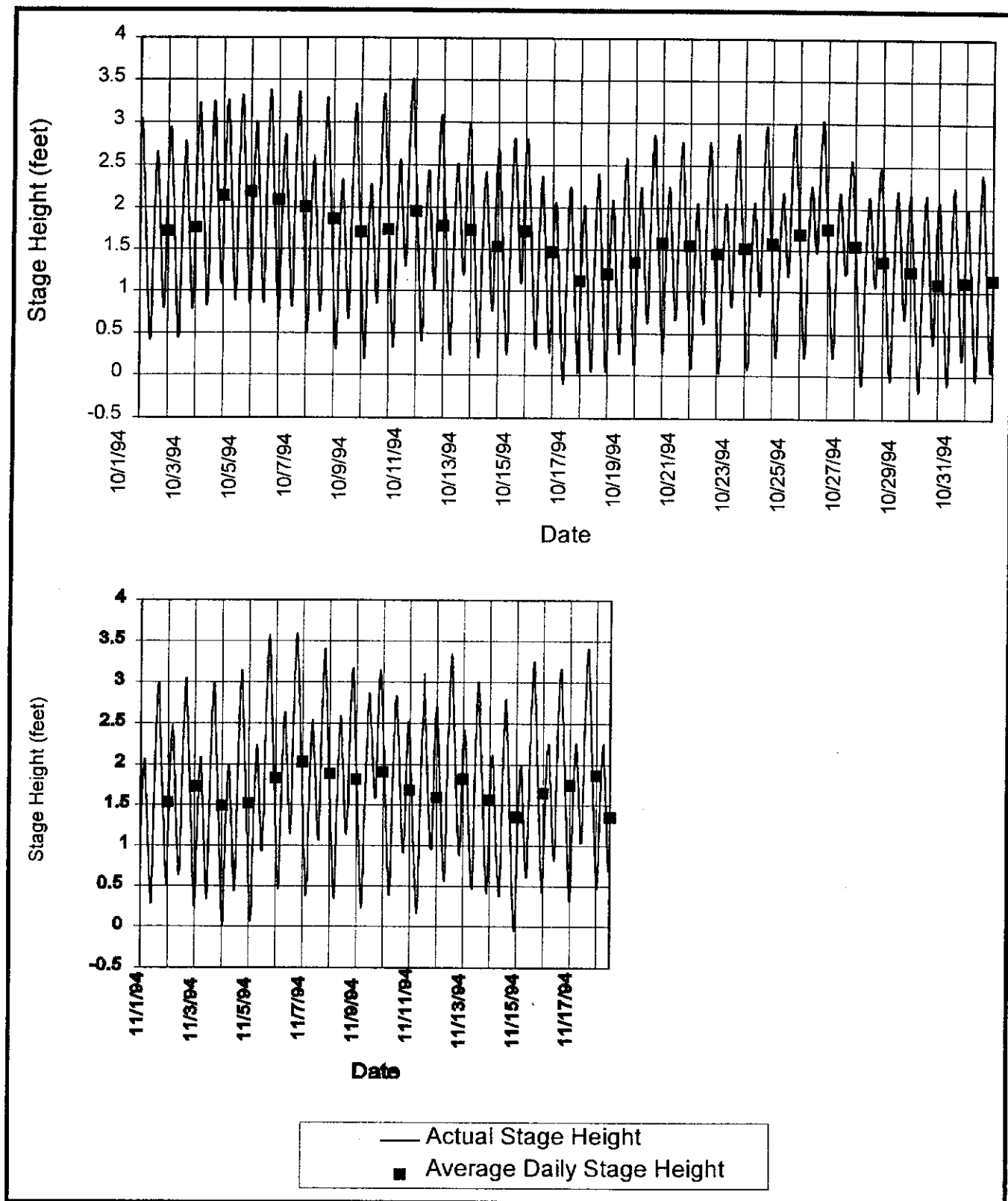
Figure 15 SACRAMENTO RIVER WATER SURFACE ELEVATION DURING THE FALL INVESTIGATIONS
