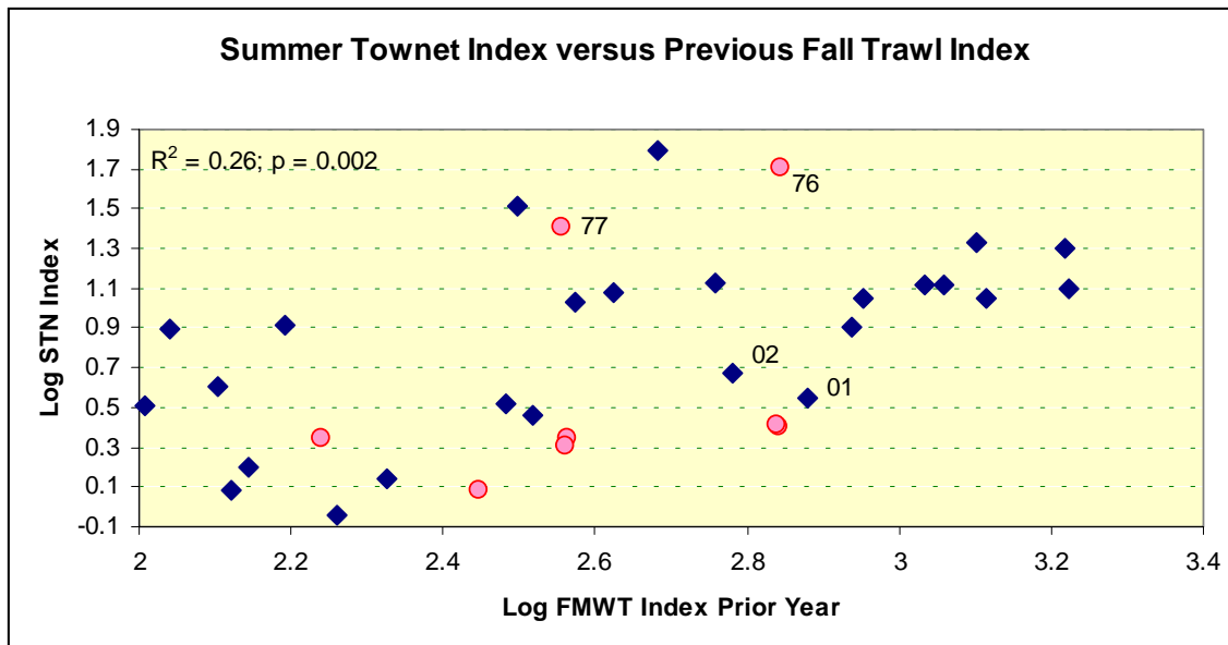
Figure S-14. Log of delta smelt summer towntnet index versus log of fall midwater trawl index the prior year – 1969-2003. Drought years shown with red dots. Drought years 1987-1992 tended to have lower production of young per size of population the previous fall.
