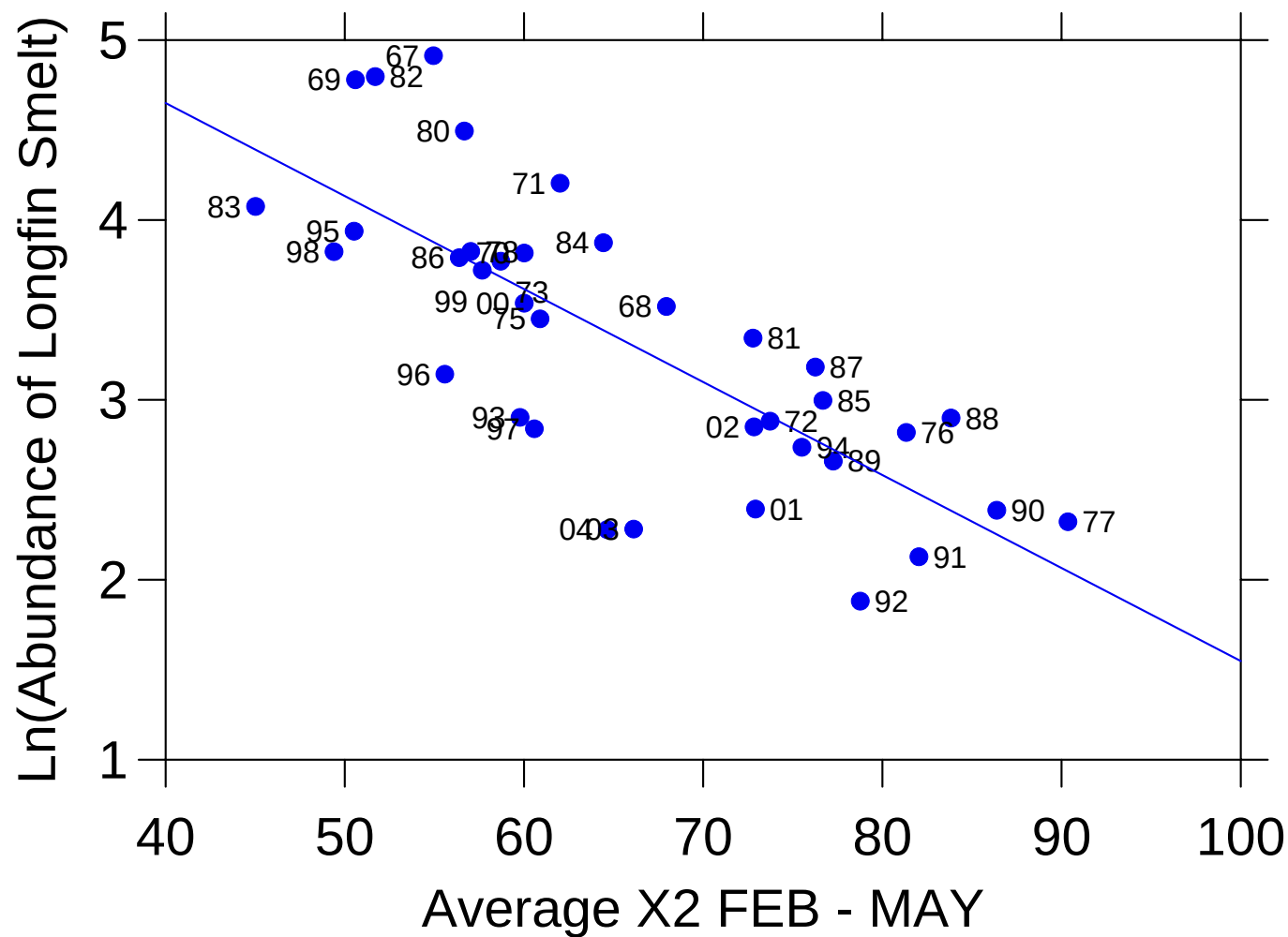
Figure 2. Longfin Smelt Abundance vs. X2 IEP Fall Midwater Trawl 1967 through 2004
