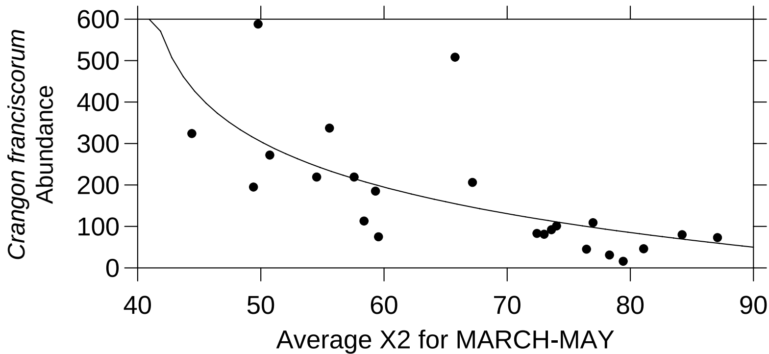
Figure 1. Bay Shrimp Year Class Strength vs. X2 IEP Bay Study Otter Trawl 1980 through 2004
