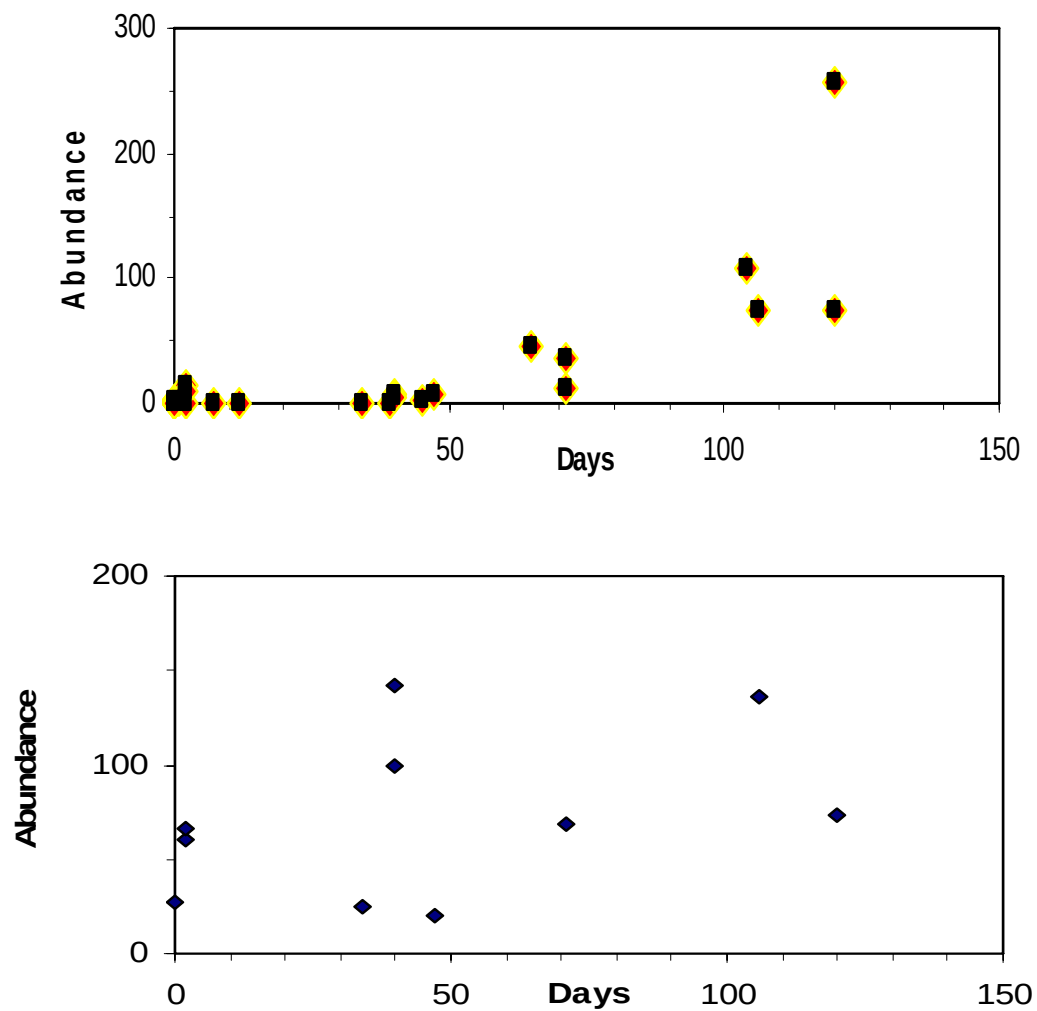
Figure 3. Days of floodplain inundating flow vs DFG FMWT Splittail Age-0 Abundance (Top) and FWS Beach Seine Abundance (Bottom)
