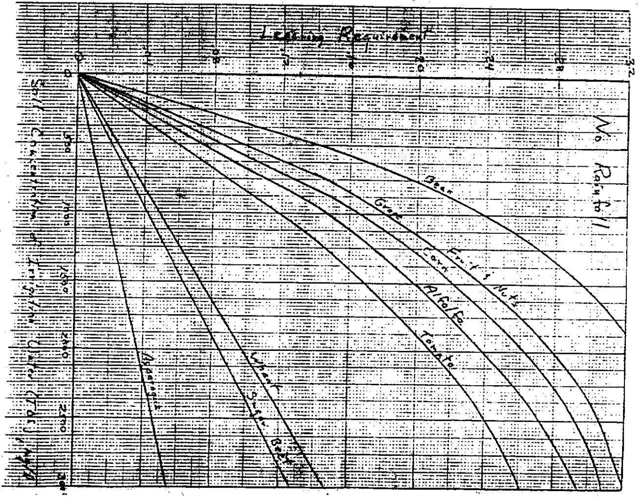
Fig. 1. Leaching requirement of the prominent crops in the South Delta as a function of the salinity of the irrigation water without rainfall.
