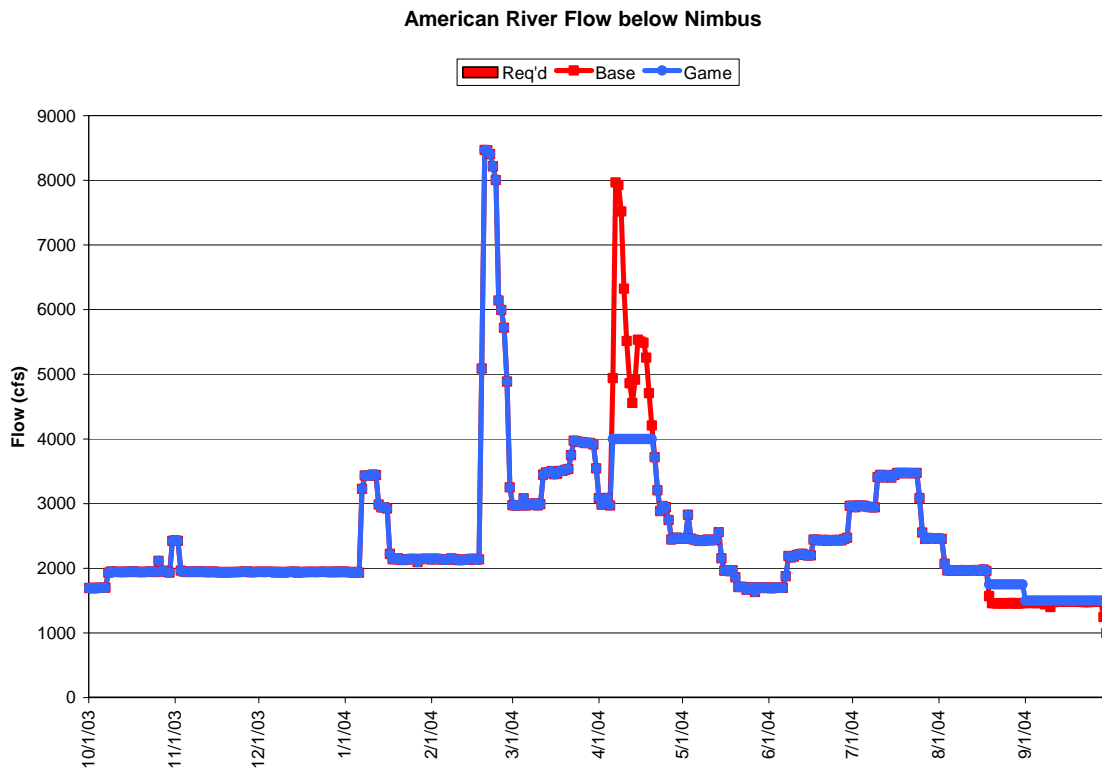
Figures 5a and 5b. Sacramento River Delta inflow and American River flow changes due to actions taken in Game 2.2 for water years 2003-04.
