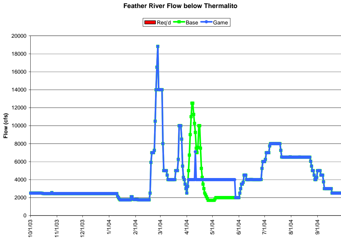
Figures 7c and 7d. Sacramento River below Keswick and Feather River below Thermalito flow changes due to actions taken in Game 3.1 for water years 2003-04.
