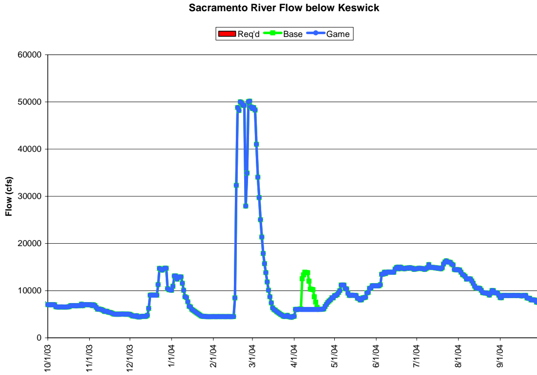
Figures 5c. Sacramento River below Keswick flow changes due to actions taken in Game 2.2 for water year 2004 (summer/fall releases for exports not simulated)..
