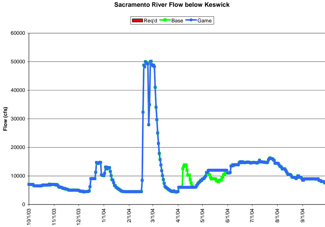
Figures 4c. Sacramento River below Keswick flow changes due to actions taken in Game 2.1 for water year 2004.
