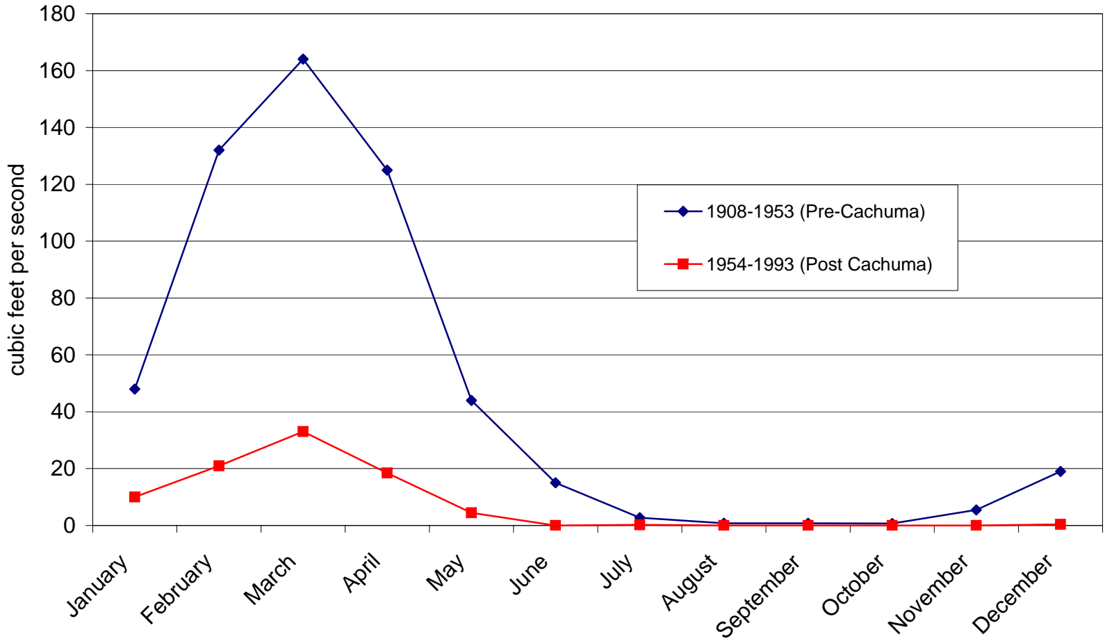
Chart 5-3. Historical Median Daily Streamflow at the Narrows
