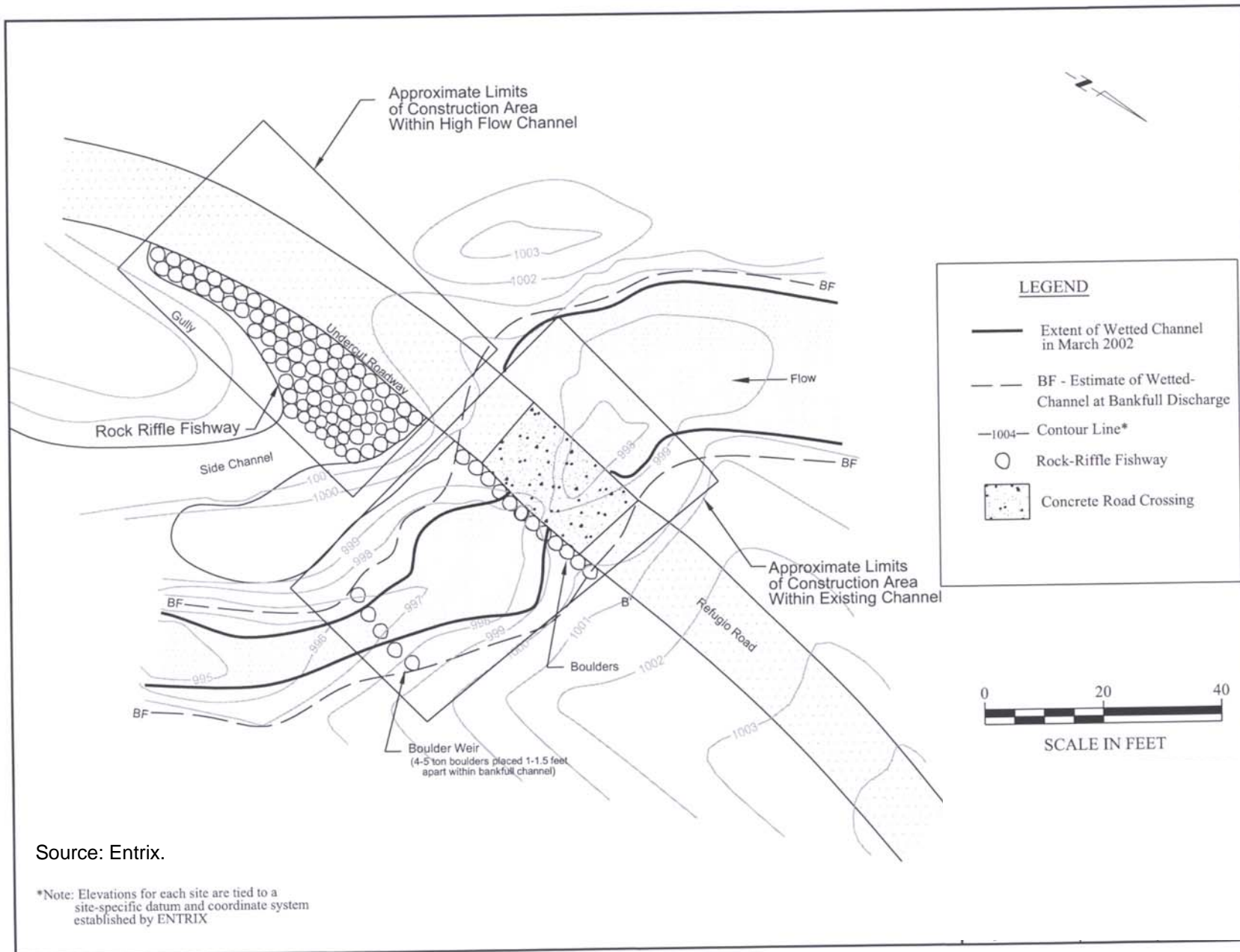
Figure 2-14. Proposed Fishway at Quiota Creek Crossing No. 5
