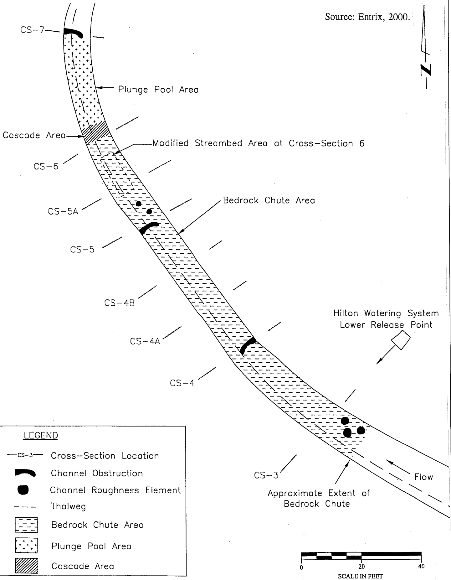
Figure 2-3. Cascade and Bedrock Chute Passage Impediments on Lower Hilton Creek
