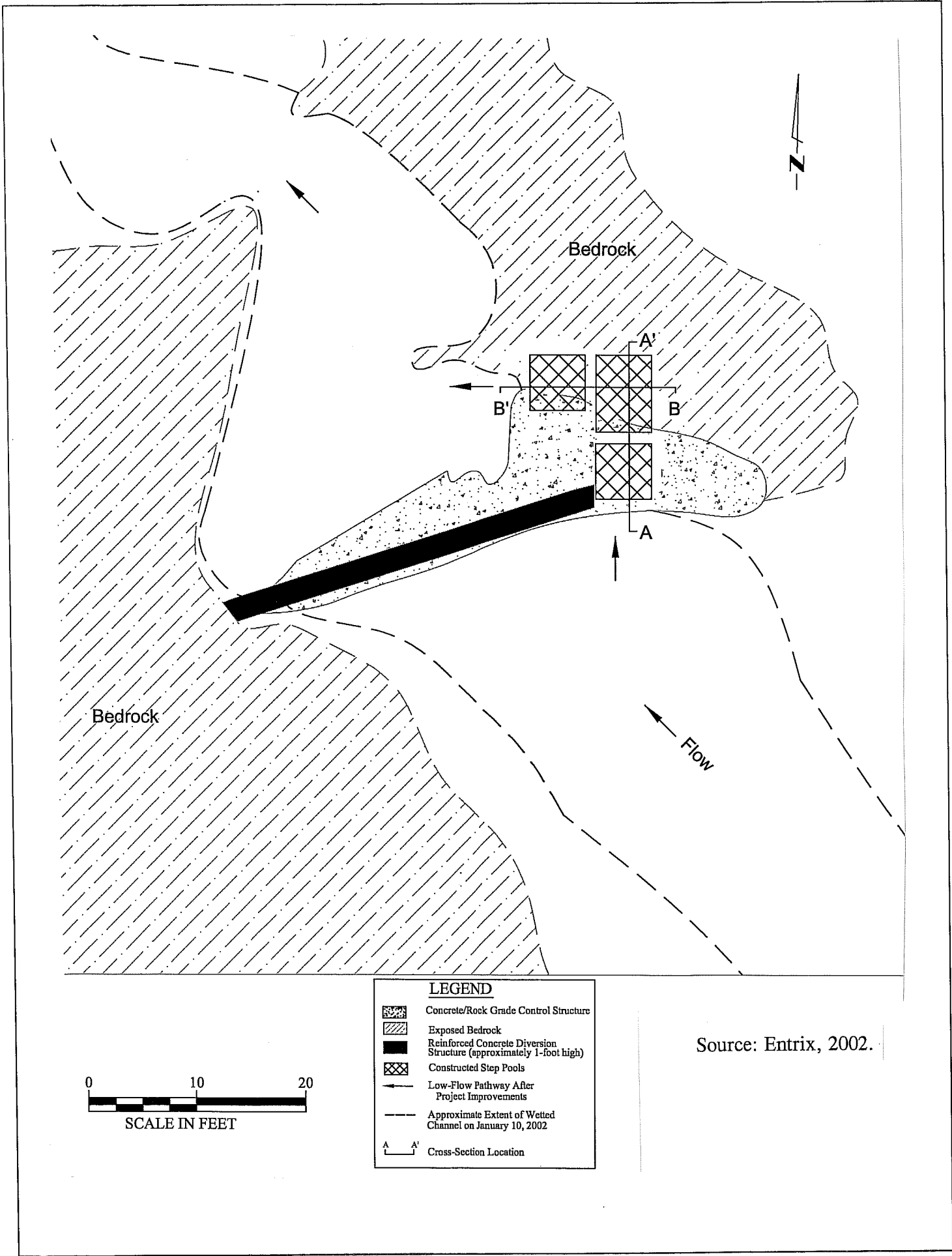
Figure 2-9. Proposed Modifications to the Grade Control Structure on Jalama Road Bridge
