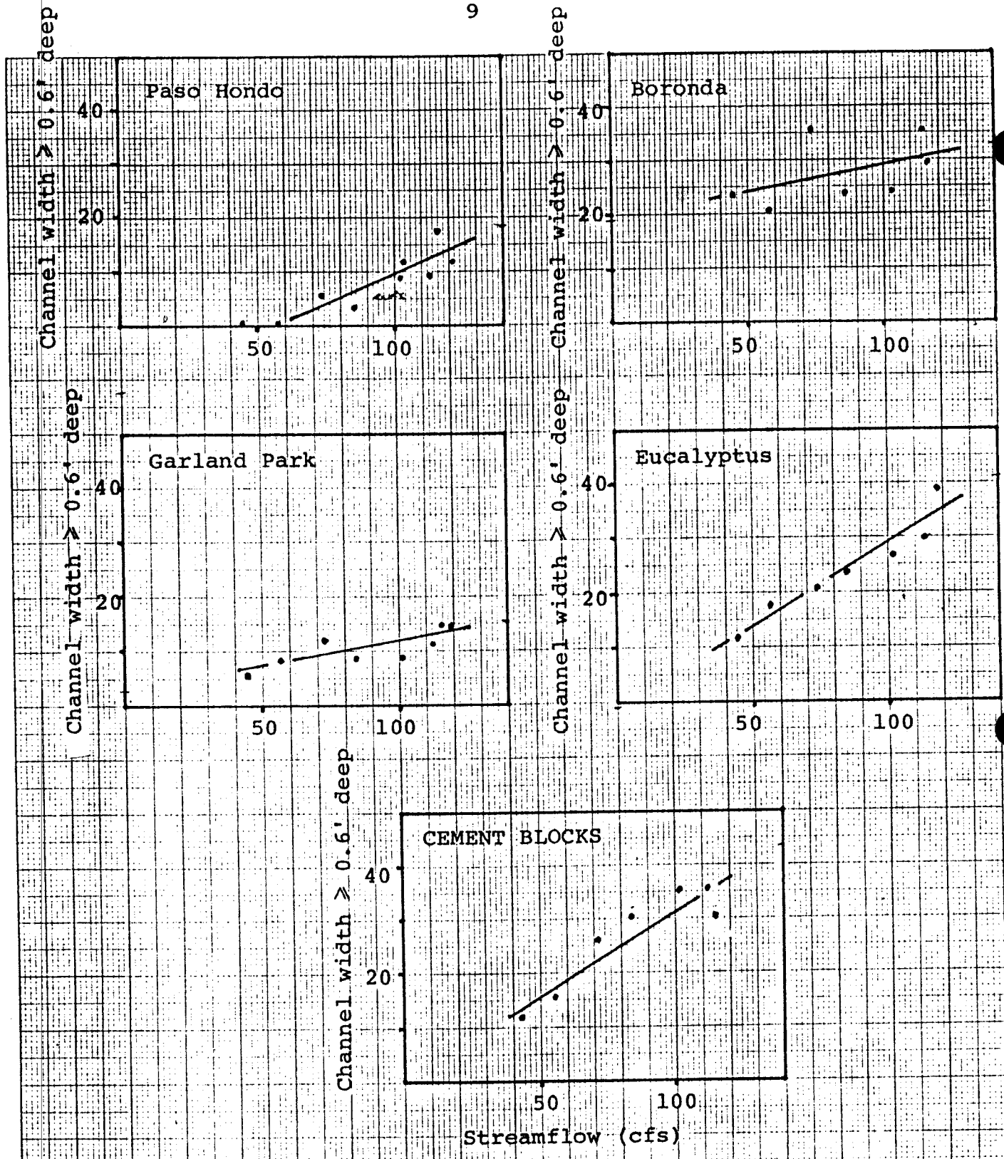
Figure II-3. Relationship between streamflows at Robles del Rio and widths of channel deep enough for steelhead migration over shallow riffles. Carmel River, 1981-82.
