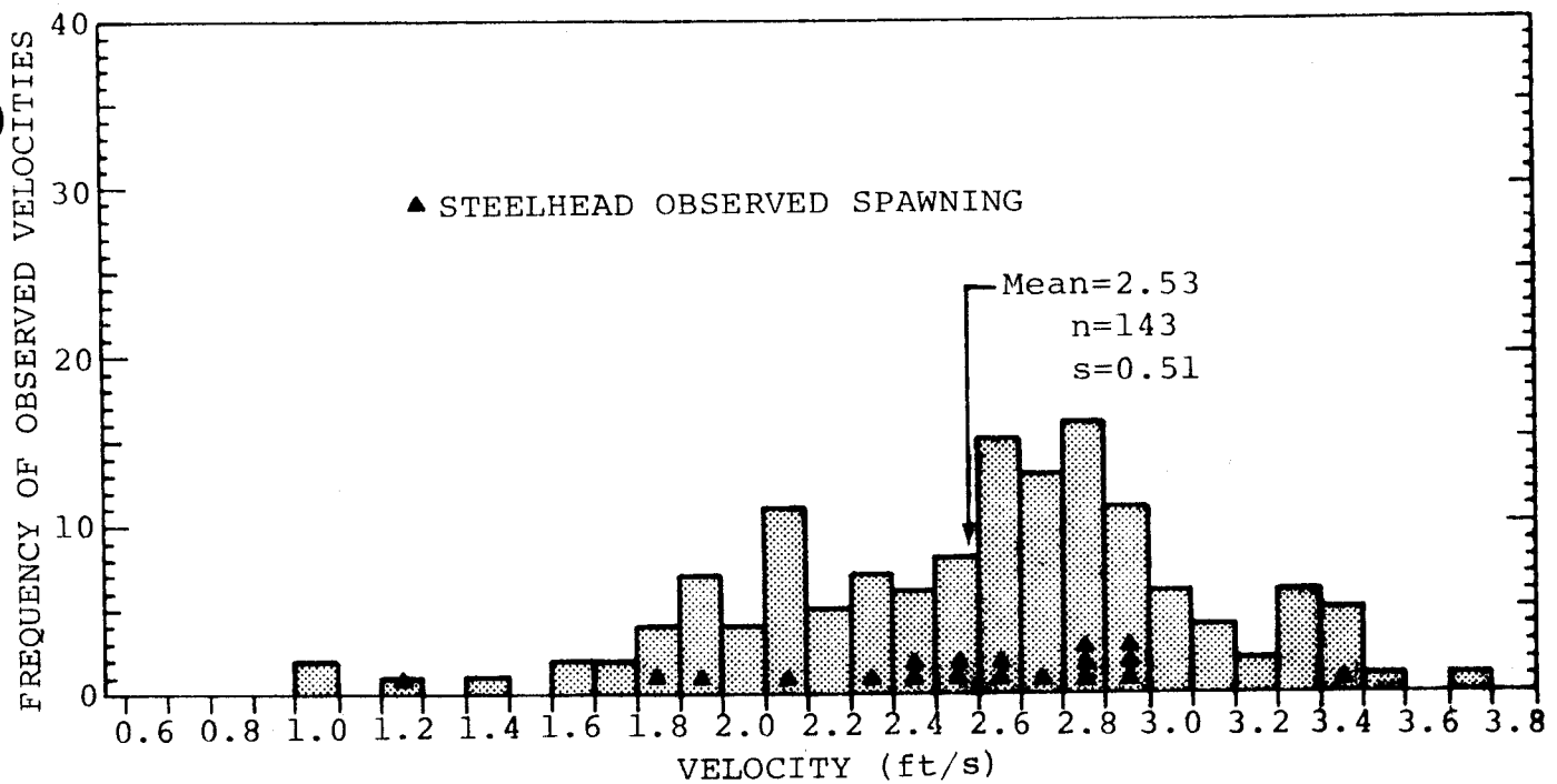
Figure III-4. Velocity of water over top of steelhead nests in Carmel River below San Clemente Dam, Feb. 22-March 10, 1982. Streamflow at time of measurement ranged from 150-230 cfs at Robles del Rio USGS gage. Velocity measured at 0.6' depth from water surface.
