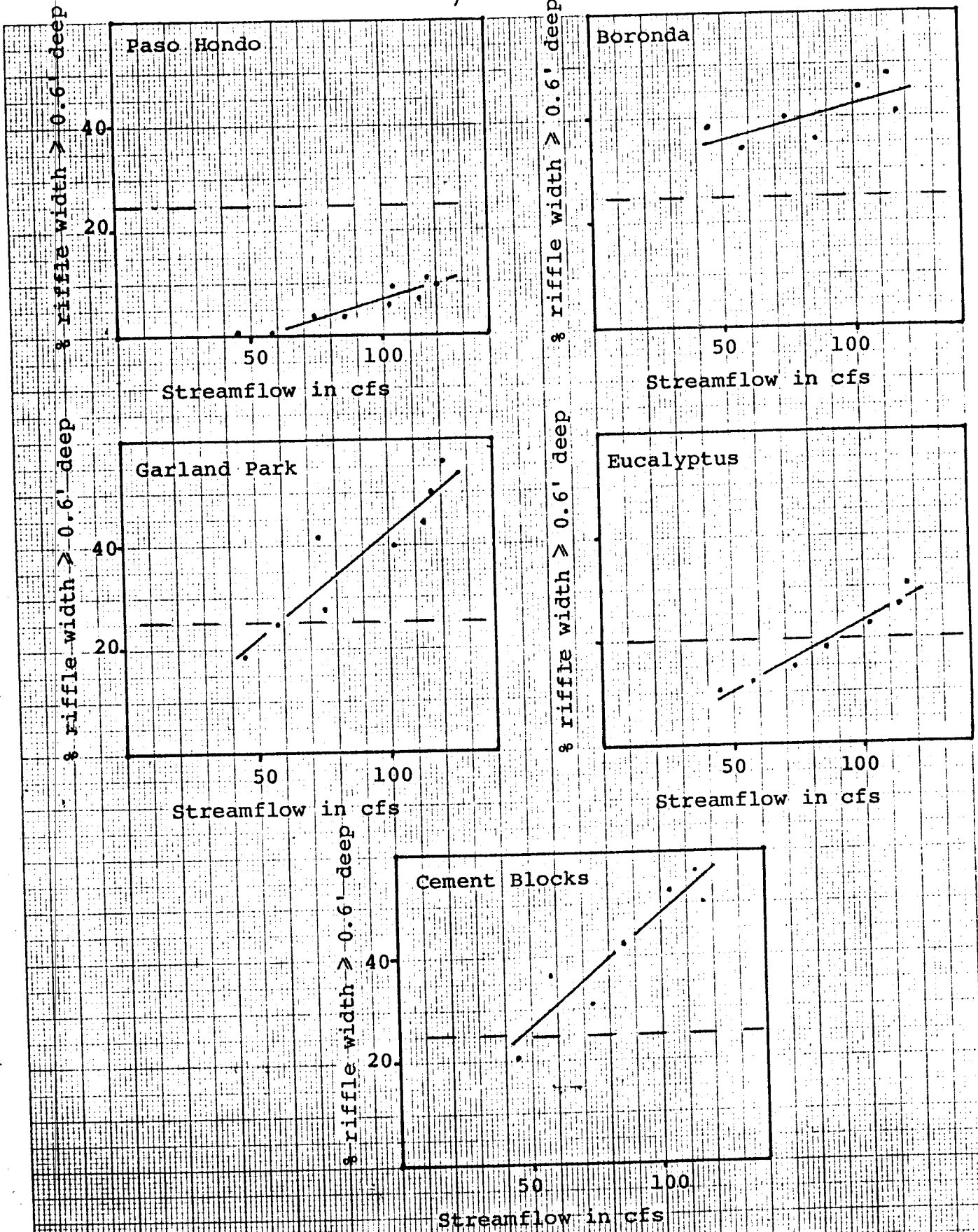
Figure II-2. Relationship between streamflows at Robles del Rio and percent of riffle widths deep enough for steelhead passage. Dash line indicates 25% of riffle width (Thompson's criteria). Carmel River, Dec. 1981-March 1982. Thompson's criteria was never met at the Paso Hondo riffle where the streambed was continuously moving.
