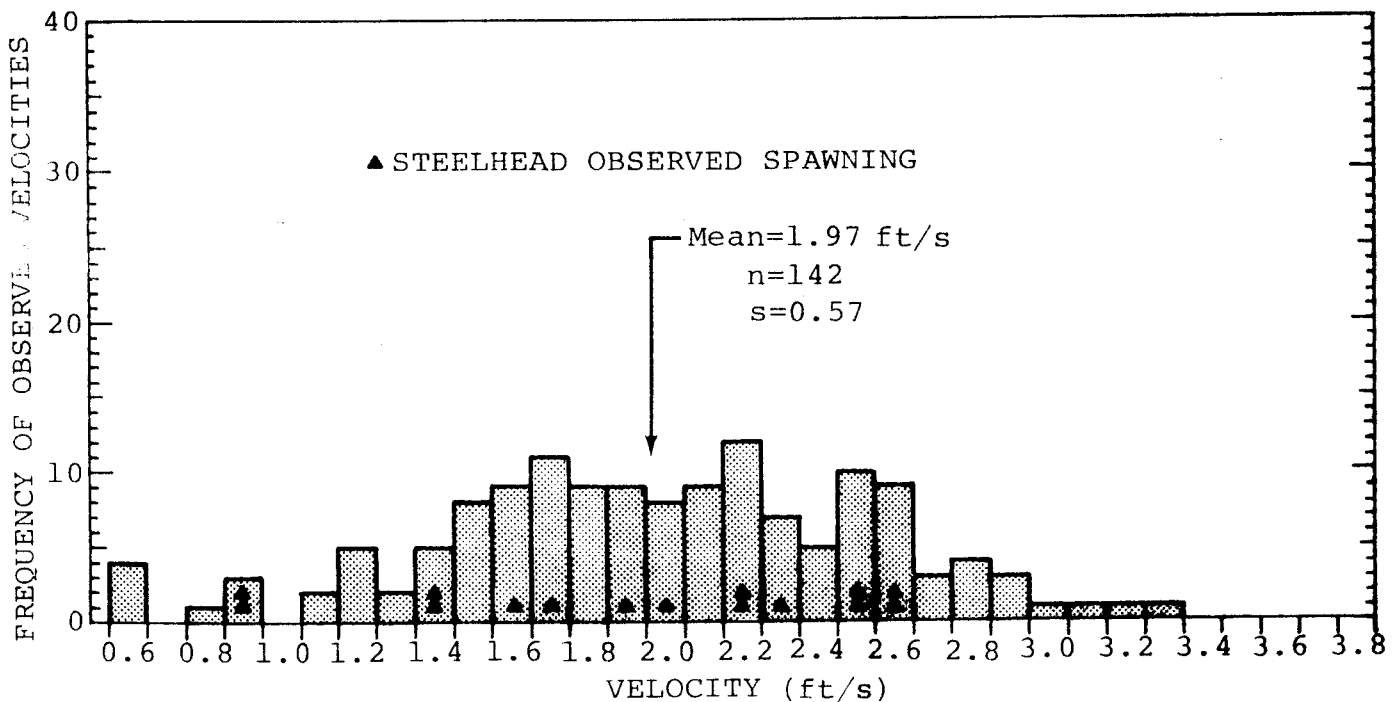
Figure III-5. Velocity of water over depression in steelhead nests in Carmel River below San Clemente Dam, Feb. 22-Mar. 10, 1982. Streamflow at time of measurements ranged from 150-230 cfs at Robles del Rio USGS gage. Velocity measured at 0.6; depth from surface of water.
