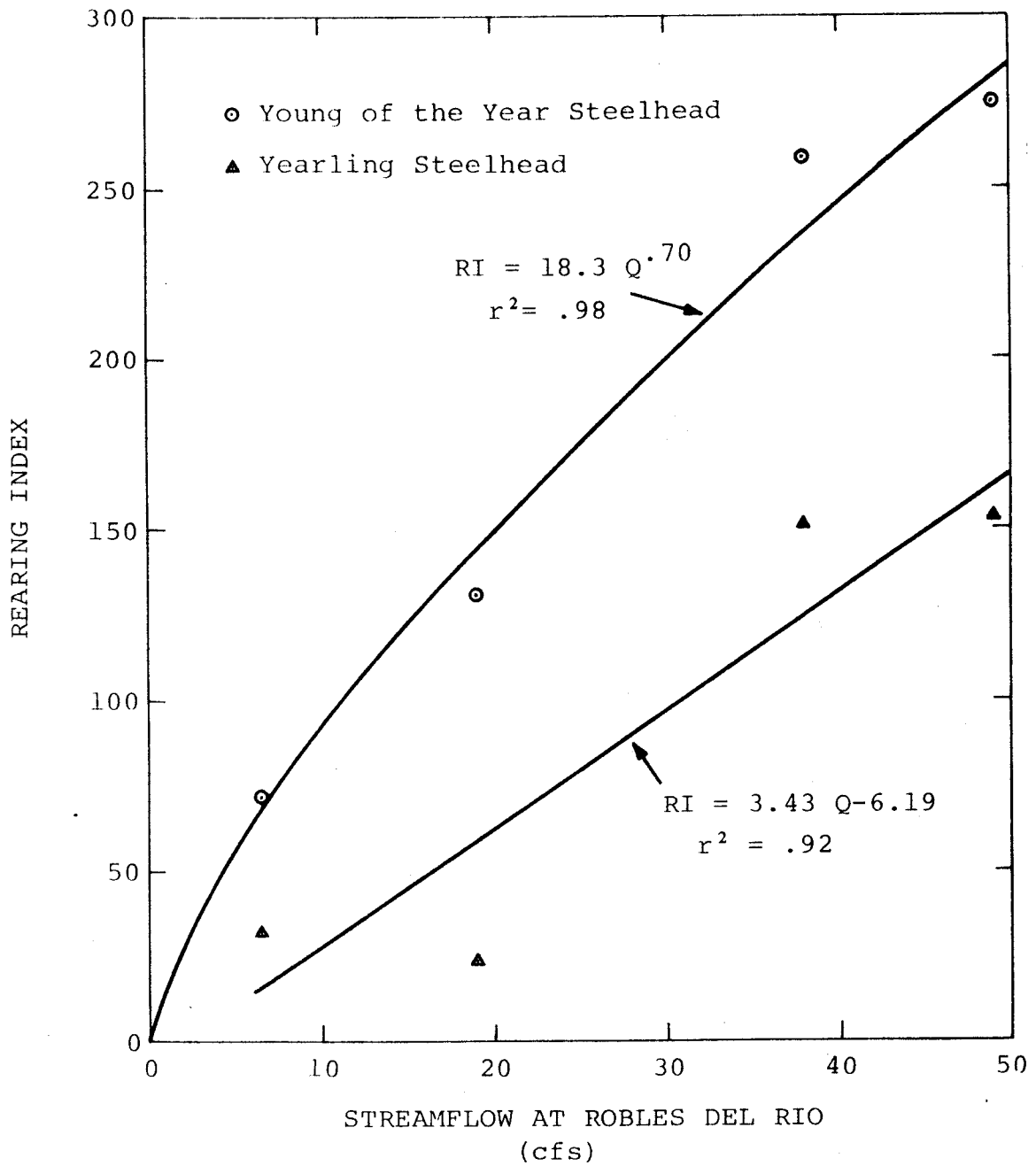
Figure IV-11c. Relationship between juvenile steelhead rearing indexes and streamflow in the Carmel River between Boronda Road Bridge and the Paso Hondo critical riffle.
