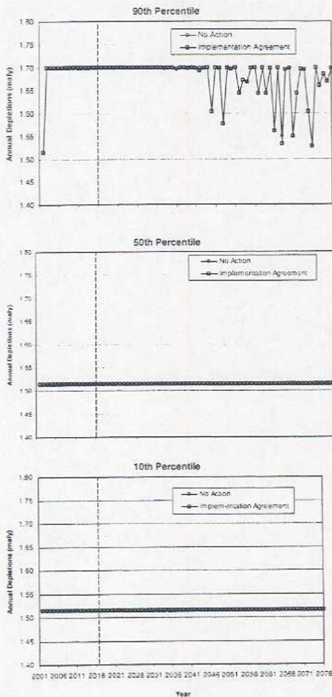
Figure 4.5-20 Mexico Modeled Annual Depletions Comparison of Implementation Agreement Conditions to No Action Conditions 90th, 50th and 10th Percentile Values
