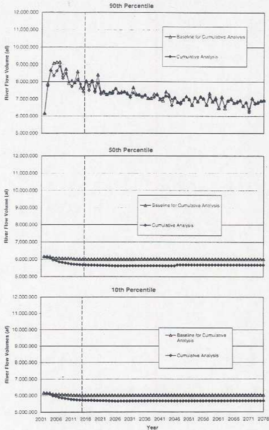
Figure 3.3-18 Colorado River Downstream of Palo Verde Diversion Dam Annual Flow Volume (af) Comparison of Cumulative Analysis to Baseline for Cumulative Analysis Conditions 90 th , 50 th and 10 th Percentile Values
