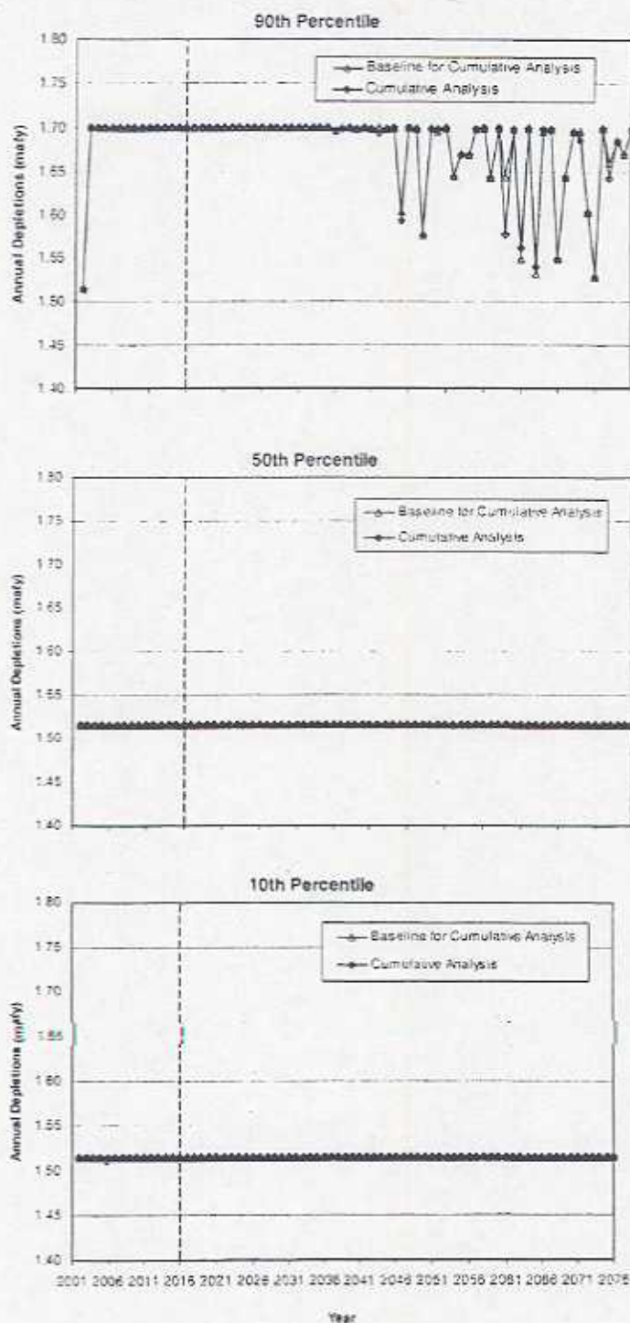
Figure 4.6-20 Mexico Modeled Annual Depletions Comparison of Cumulative Analysis Conditions to Baseline Conditions 90th, 50th and 10th Percentile Values
