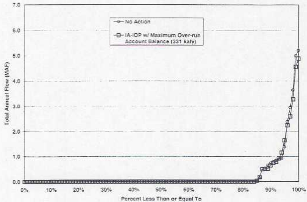
Figure 20 Comparison of Magnitude of Excess Flows Below Morelos Dam in Year 2026 No Action to IA-IOP w/ Maximum Observed Lower Basin Overrun Account Balance of 331 kafy 10 Percent Maximum Allowed Overrun w/ 3-Year Payback Schedule
