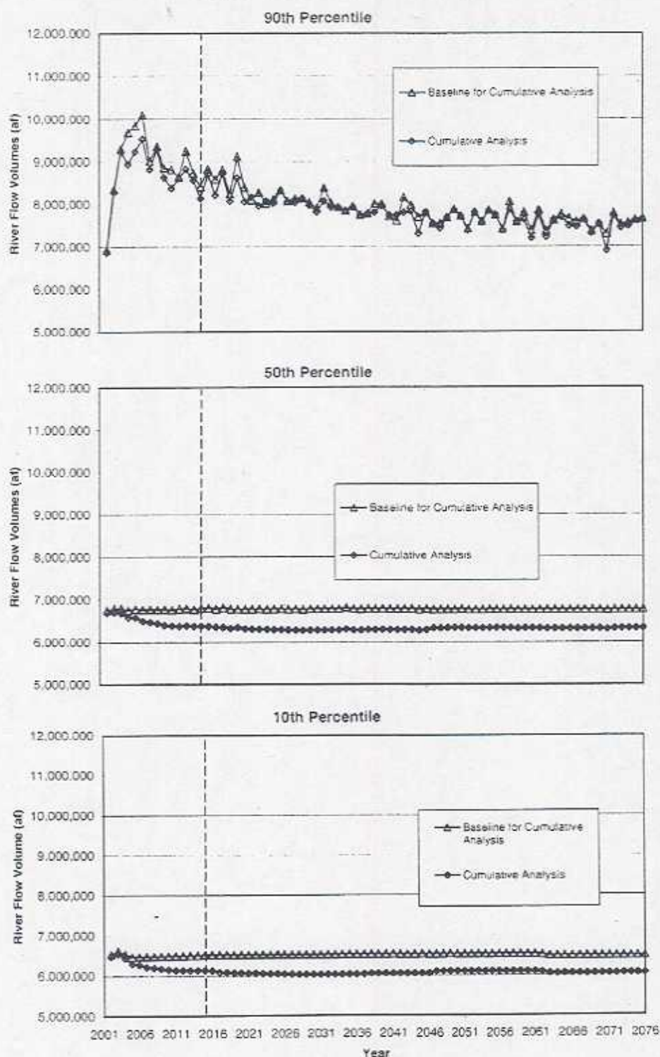
Figure 3.3-15 Colorado River Upstream of CRIR Diversion Annual Flow Volume (af) Comparison of Implementation Agreement to Baseline for Cumulative Analysis Conditions 90 th , 50 th and 10 th Percentile Values
