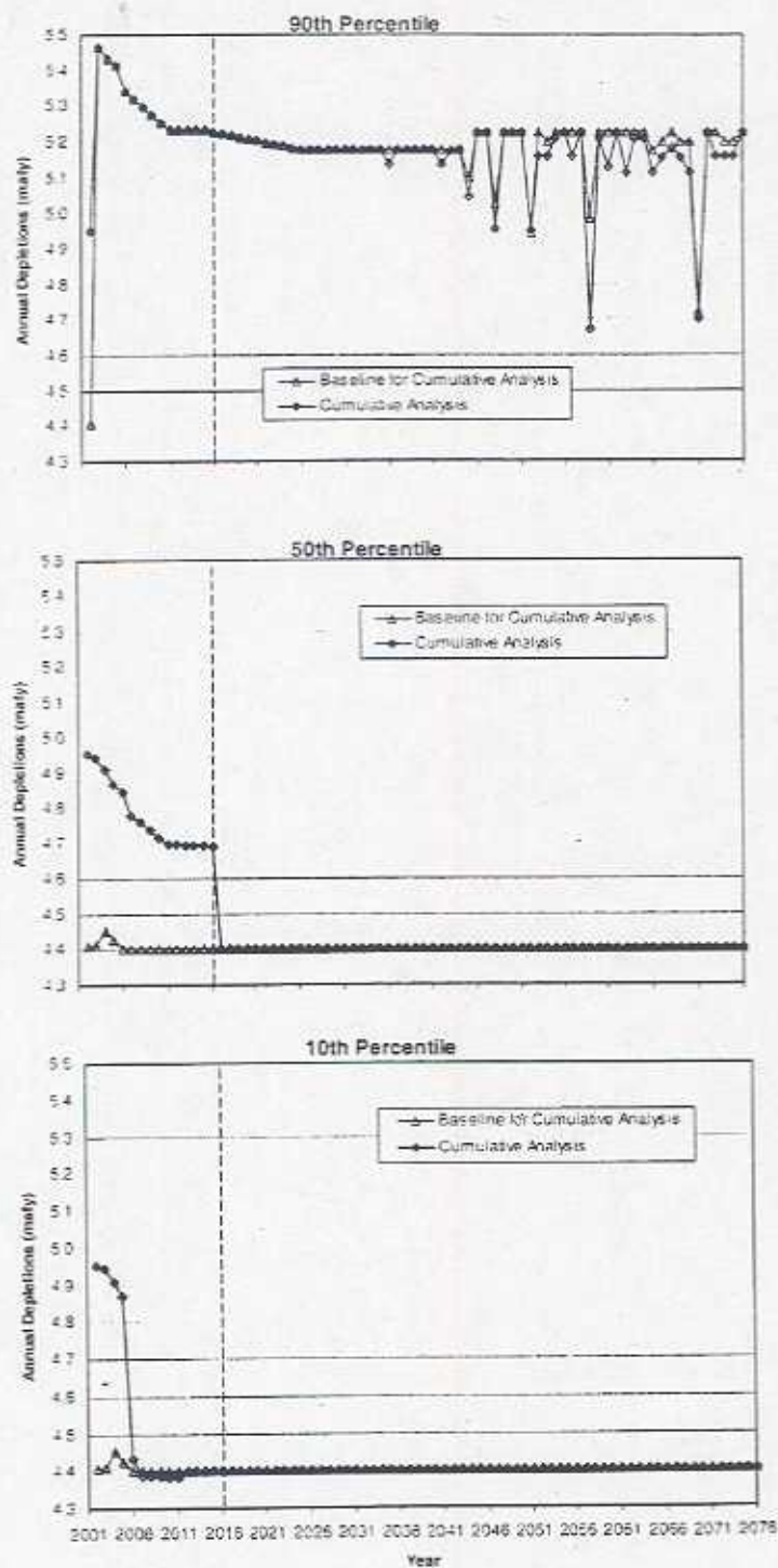
Figure 4.6-10 California Modeled Annual Depletions Comparison of Cumulative Analysis Conditions to Baseline Conditions 90th, 50th and 10th Percentile Values
