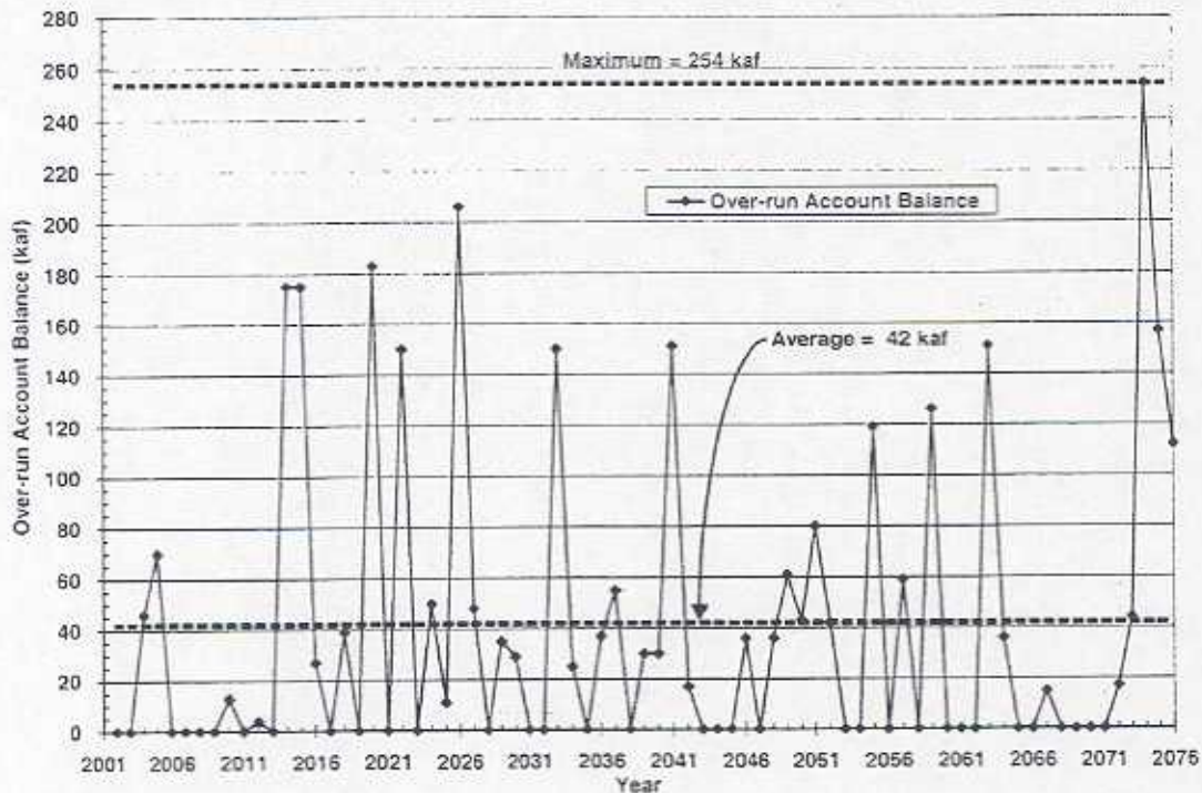
Figure 10 End-of-Year Overrun Account Balances and Resulting Reductions in Lake Mead Storage (PVID/YPRD/ID/CVWD End-of-Year Overrun Account Balances – Based on 10% O.R. & 1-Year Payback)
