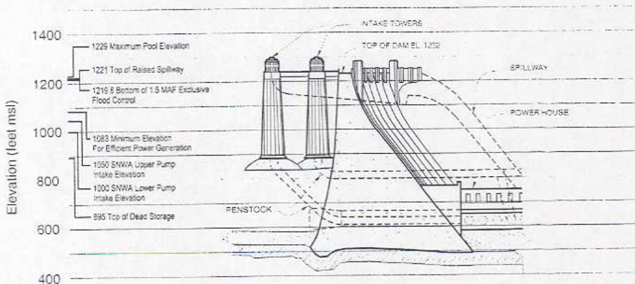
Figure 1.3-1 Lake Mead and Hoover Dam Important Operating Elevations
