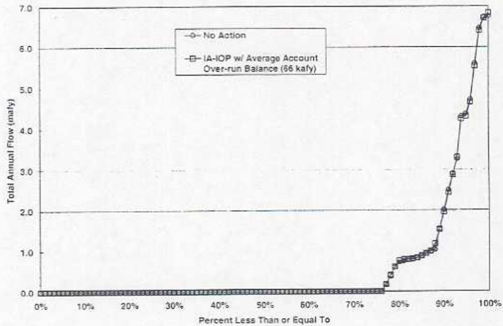
Figure 13 Comparison of Magnitude of Excess Flows Below Morelos Dam in Year 2006 No Action to IA-IOP w/ Average Lower Basin Over-run Account Balance of 66 kafy 10 Percent Maximum Allowed Overrun w/ 3-Year Payback Schedule
