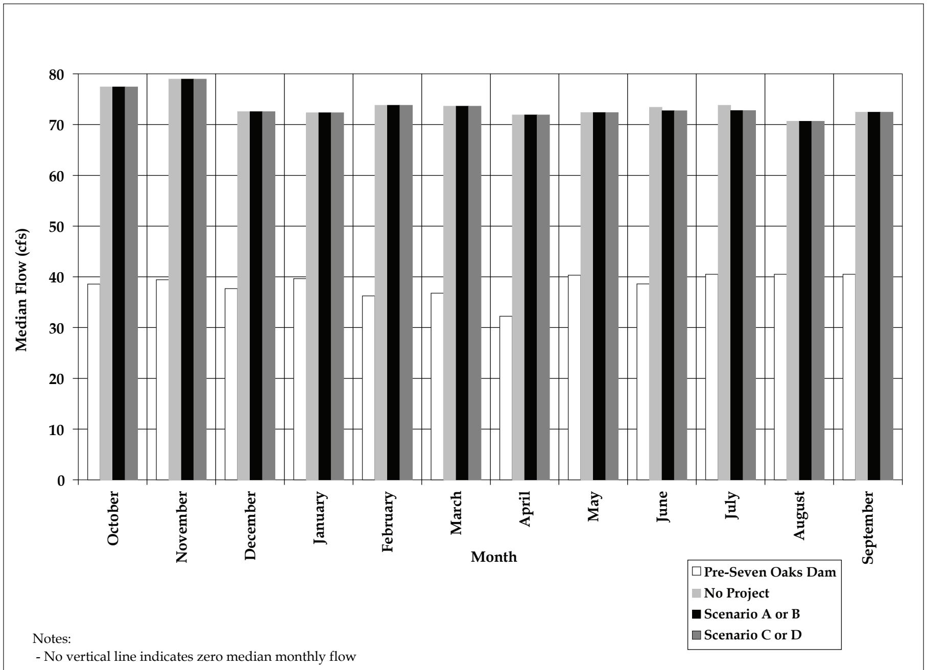
Figure 6.2-6. Median Monthly Flows (Non-Storm Days) for SAR Segment F, below RIX and Rialto Effluent Outfall, WY 1966-67 through WY 1999-2000
