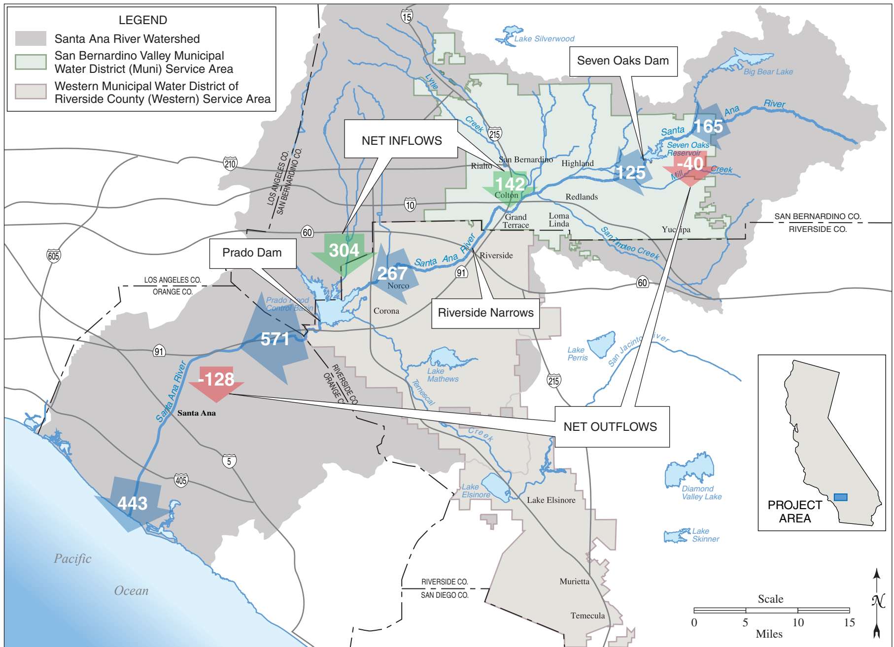
Santa Ana River Flows in Water Year 1992-1993 (in thousands of acre-feet)
