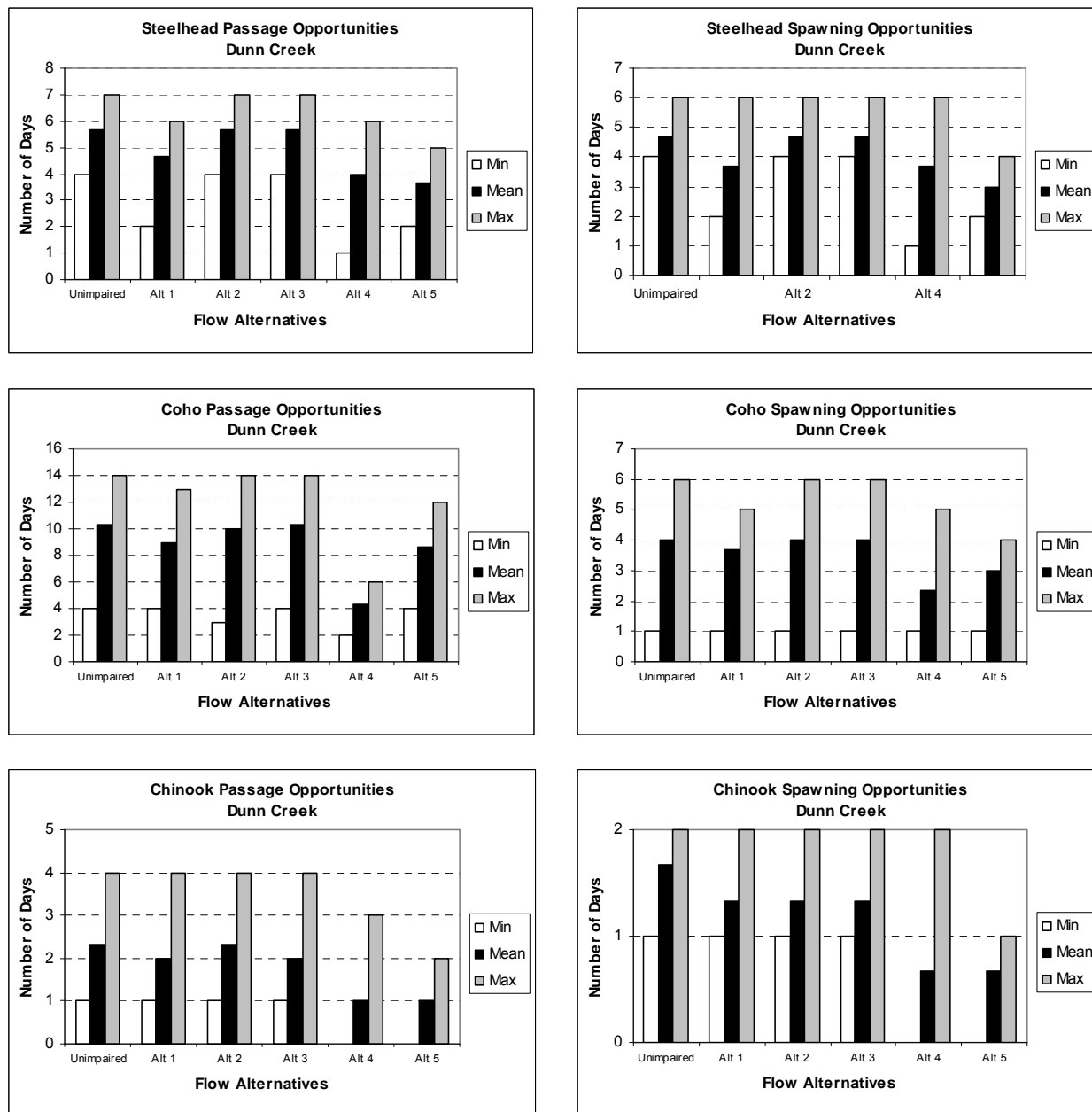
Figure I-3. Comparison of Flow Alternative Scenarios 1 to 5 and unimpaired flow conditions for upstream passage and spawning in the Dunn Creek validation site (drainage area = 1.9 mi 2 ), expressed as number of days per water year. Minimum, mean, and maximum values are evaluated for each species' passage and spawning periods, for the period of record at a nearby USGS stream gage.
