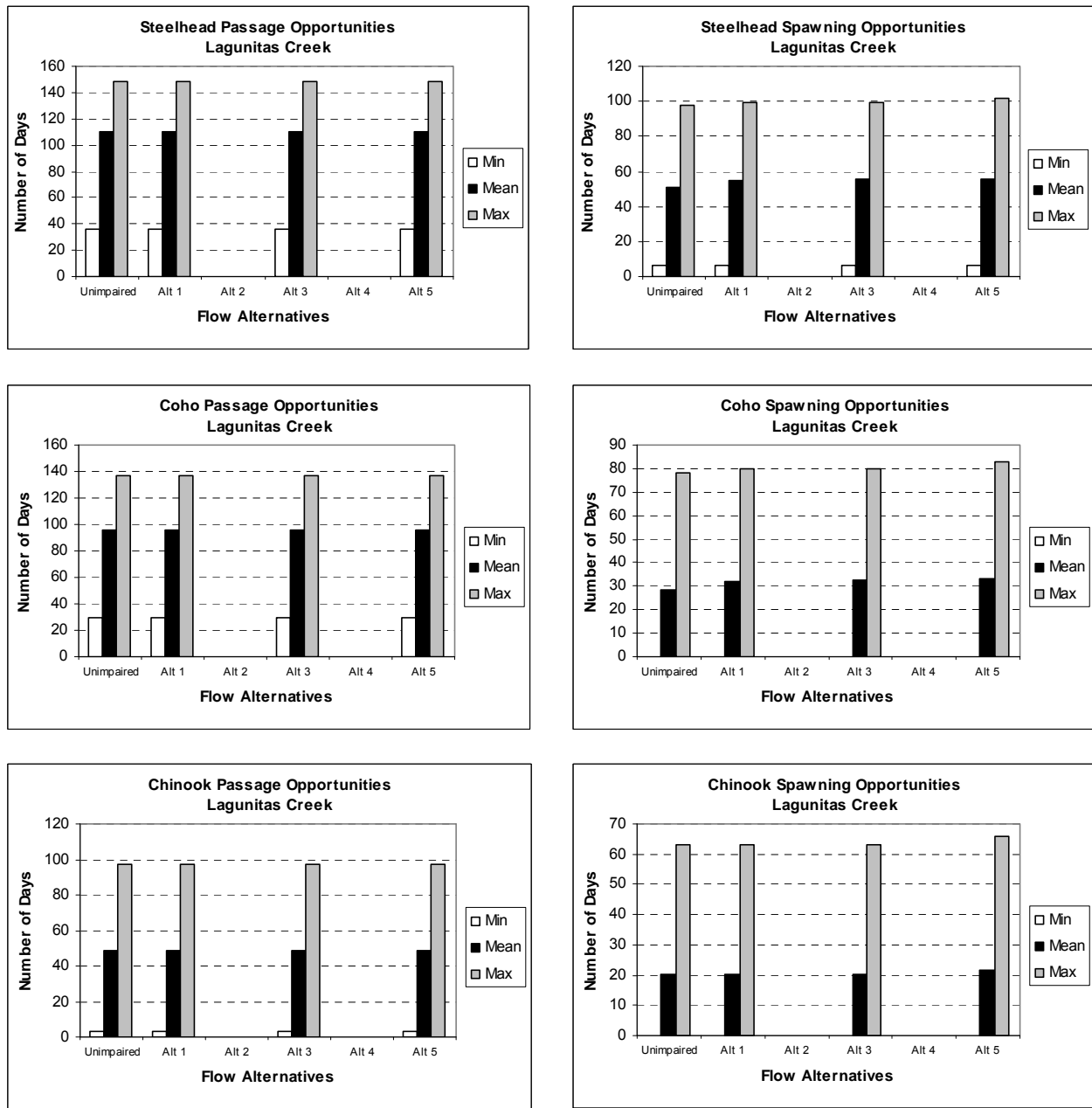
Figure I-13. Comparison of Flow Alternative Scenarios 1 to 5 and unimpaired flow conditions for upstream passage and spawning in the Lagunitas Creek validation site (drainage area = 34 mi 2 ), expressed as number of days per water year. Minimum, mean, and maximum values are evaluated between 10/1-3/31 over the period of record at a nearby USGS stream gage.
