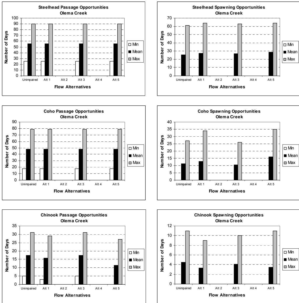
Figure I-6. Comparison of Flow Alternative Scenarios 1 to 5 and unimpaired flow conditions for upstream passage and spawning in the Olema Creek validation site (drainage area = 7.0 mi 2 ), expressed as number of days per water year. Minimum, mean, and maximum values are evaluated for each species' passage and spawning periods, for the period of record at a nearby USGS stream gage.
