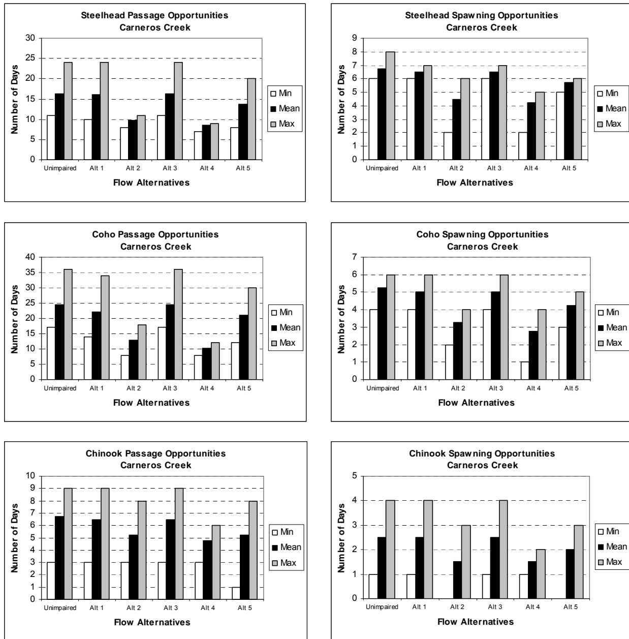
Figure I-4. Comparison of Flow Alternative Scenarios 1 to 5 and unimpaired flow conditions for upstream passage and spawning in the Carneros Creek validation site (drainage area = 2.8 mi 2 ), expressed as number of days per water year. Minimum, mean, and maximum values are evaluated for each species' passage and spawning periods, for the period of record at a nearby USGS stream gage.
