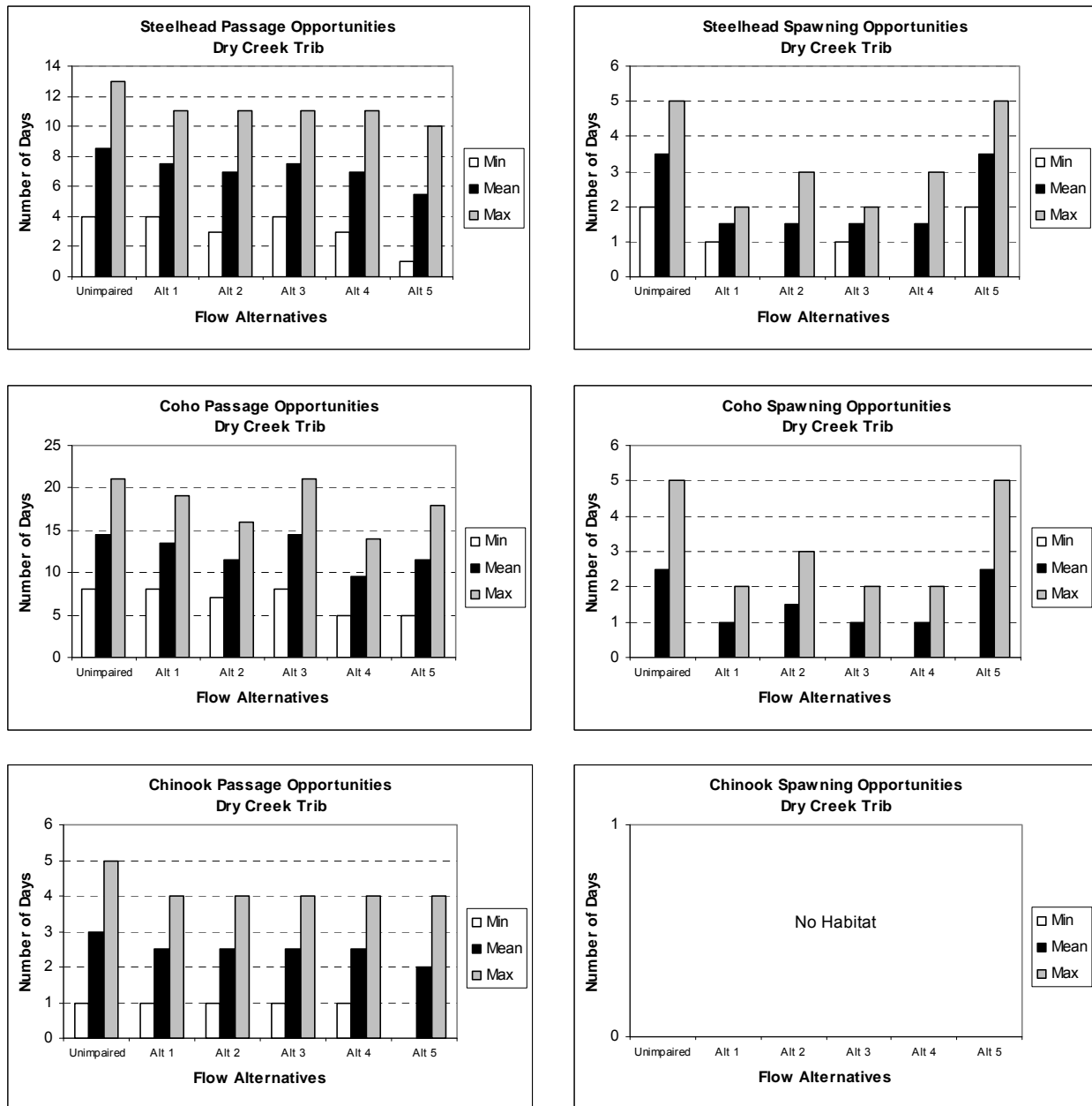
Figure I-2. Comparison of Flow Alternative Scenarios 1 to 5 and unimpaired flow conditions for upstream passage and spawning in the Dry Creek Tributary validation site (drainage area = 1.2 mi 2 ), expressed as number of days per water year. Minimum, mean, and maximum values are evaluated for each species' passage and spawning periods, for the period of record at a nearby USGS stream gage.
