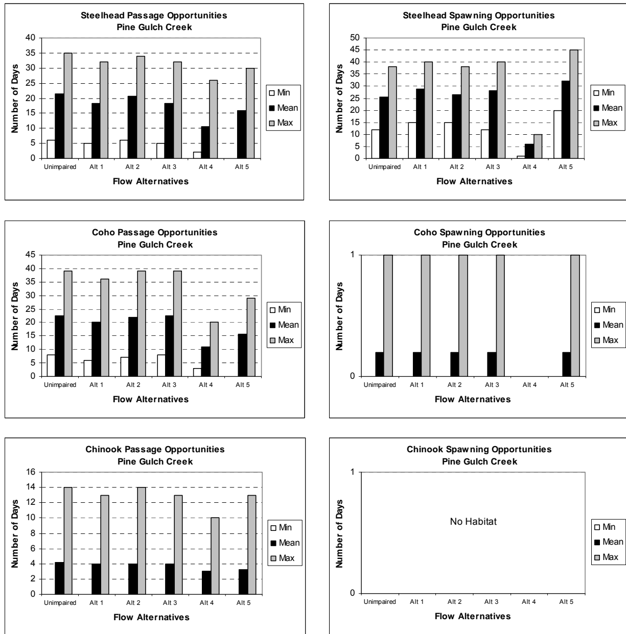
Figure I-7. Comparison of Flow Alternative Scenarios 1 to 5 and unimpaired flow conditions for upstream passage and spawning in the Pine Gulch Creek validation site (drainage area = 7.8 mi 2 ) expressed as number of days per water year. Minimum, mean, and maximum values are evaluated for each species' passage and spawning periods, for the period of record at a nearby USGS stream gage.
