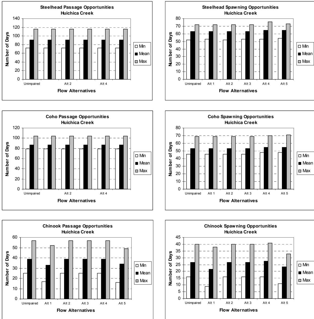
Figure I-5. Comparison of Flow Alternative Scenarios 1 to 5 and unimpaired flow conditions for upstream passage and spawning in the Huichica Creek validation site (drainage area = 4.9 mi 2 ), expressed as number of days per water year. Minimum, mean, and maximum values are evaluated for each species' passage and spawning periods, for the period of record at a nearby USGS stream gage.
