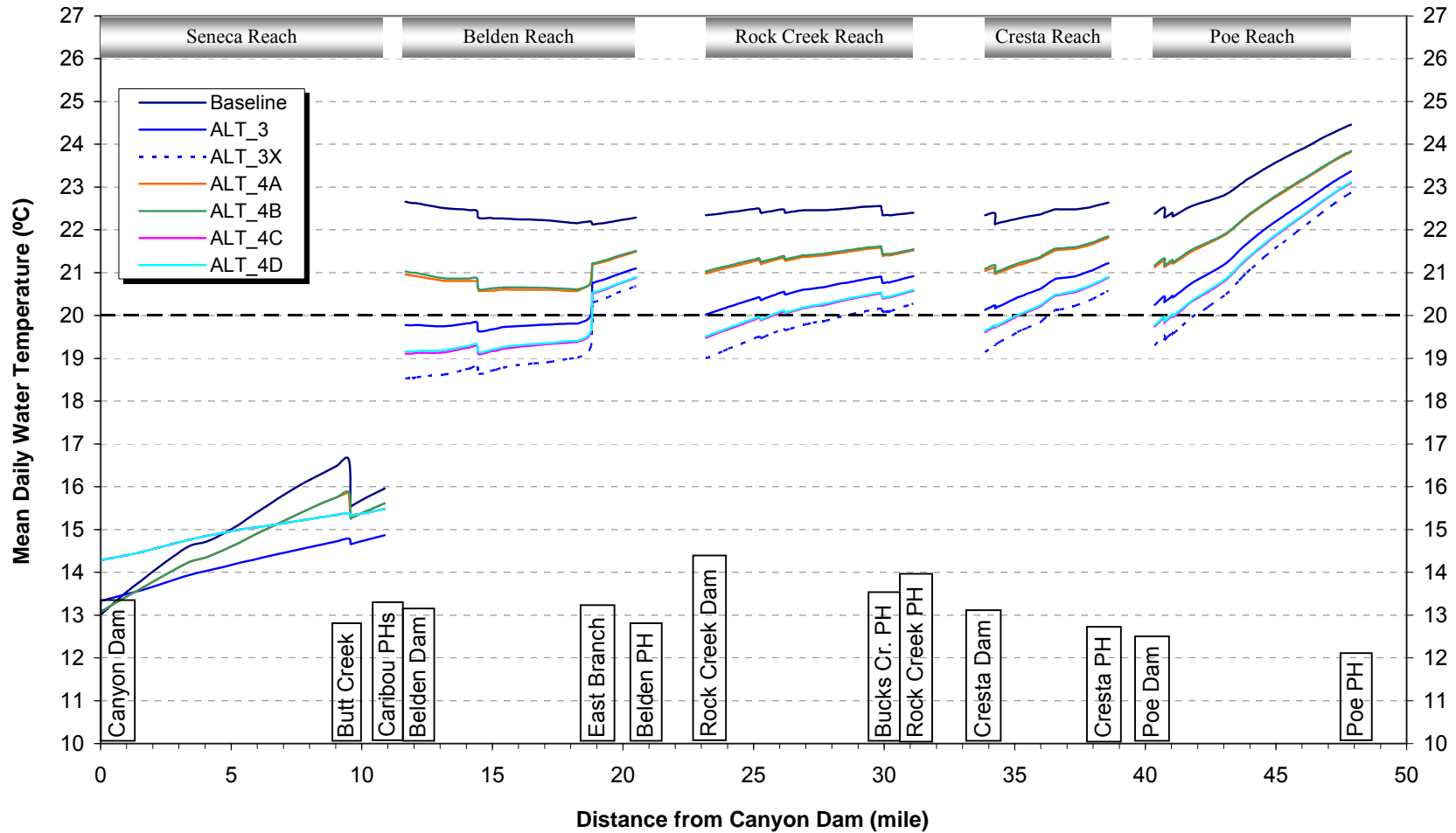
Figure 8. Comparison of NFFR water temperature longitudinal profiles between alternatives — August, 10% exceedance (from Stetson Engineers 2009).
